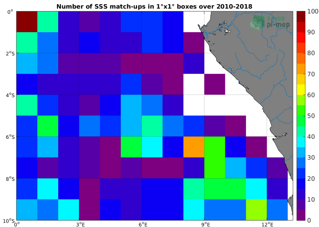
Figure 4: Number of SSS match-ups between Argo SSS and the CCI-L4-ESA-MERGED-OI-V1.8-7DAY-RUNNING SSS product for the Congo river plume Pi-MEP region over 1°x1° boxes and for the full satellite product period.
