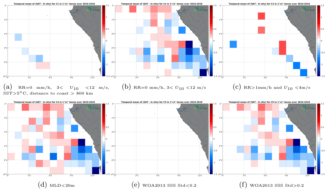
Figure 12: Temporal mean gridded over spatial boxes of size 1^\circ \times 1^\circ of \Delta SSS (CCI-L4-ESAMERGED-OI-V1.8-7DAY-RUNNING - Argo) for 6 different subdatasets corresponding to:RR=0 mm/h, 3 < U_{10} < 12 m/s, SST >5^\circ C, distance to coast > 800 km (a), RR=0 mm/h, 3 < U_{10} < 12 m/s (b), RR >1 mm/h and U_{10} < 4 m/s (c),MLD <20 m (d),WOA2013 SSS Std <0.2 (e),WOA2013 SSS Std >0.2 (f).
