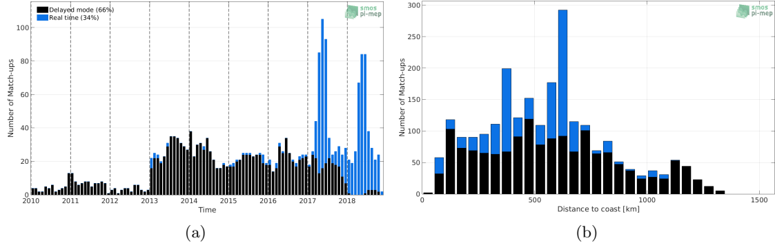
Figure 1: Number of match-ups between Argo and CCI-L4-ESA-MERGED-OI-V1.8-7DAY-RUNNING SSS as a function of time (a) and as function of the distance to coast (b) over the Congo river plume Pi-MEP region and for the full satellite product period.
