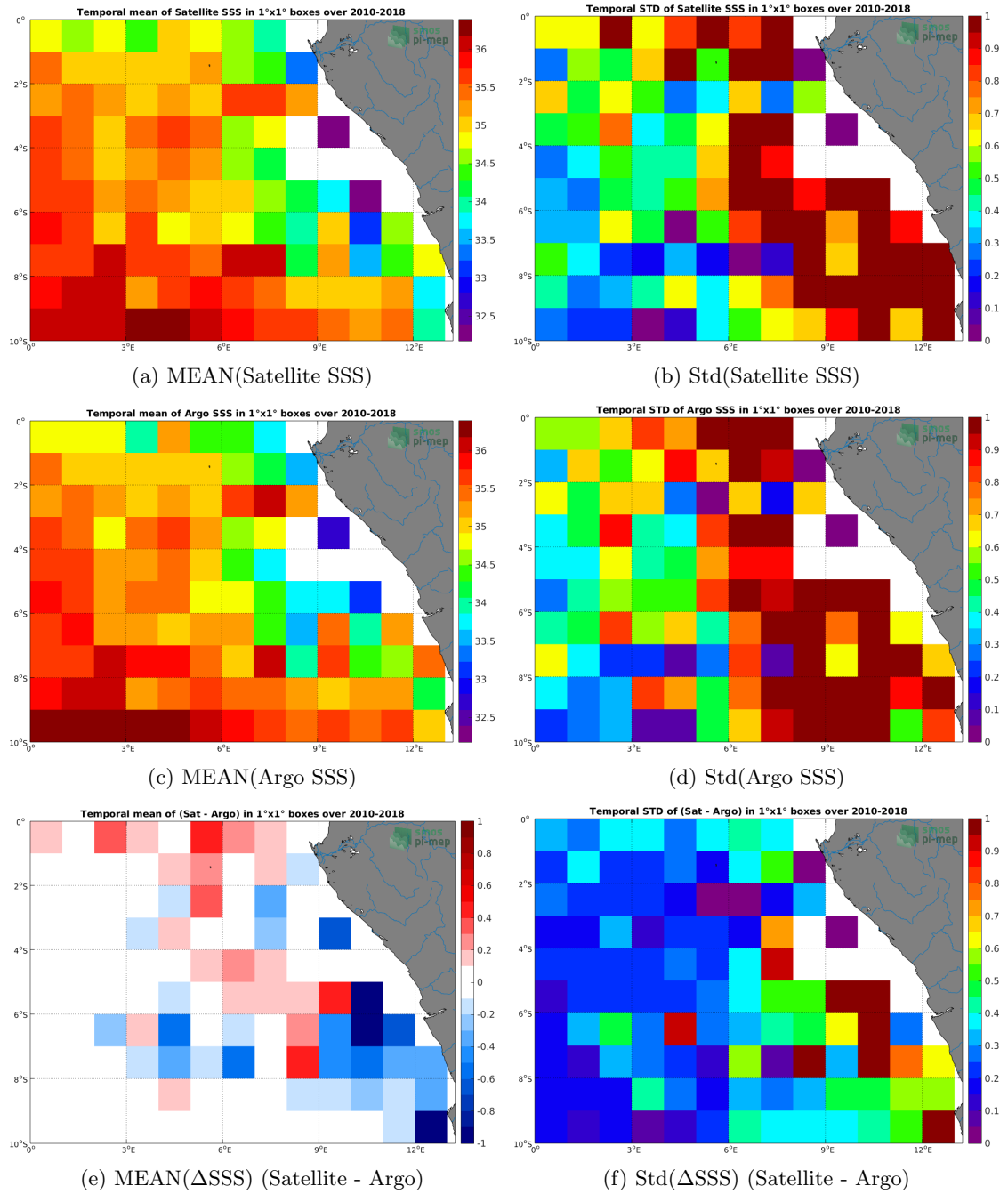
Figure 6: Temporal mean (left) and Std (right) of SSS from CCI-L4-ESA-MERGED-OI-V1.8-7DAY-RUNNING (top), Argo (middle), and of \Delta SSS (Satellite - Argo). Only match-up pairs are used to generate these maps.
