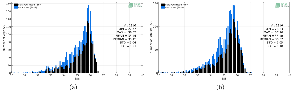
Figure 2: Histograms of SSS from Argo (a) and CCI-L4-ESA-MERGED-OI-V1.8-7DAY-RUNNING (b) considering all match-up pairs per bins of 0.1 over the Congo river plume Pi-MEP region and for the full satellite product period.
