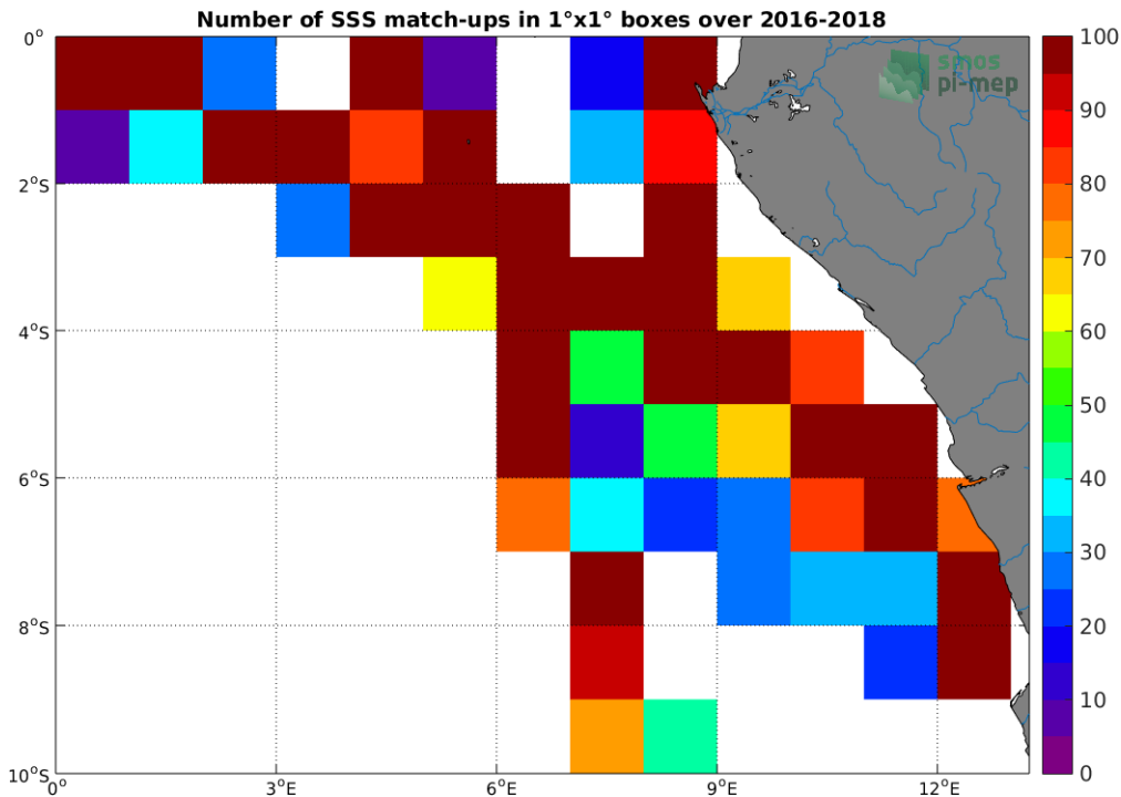
Figure 4: Number of SSS match-ups between TSG-LEGOS-DM SSS and the CCI L4 Merged-OI v1.8 - 30-day running (ESA) SSS product for the Congo river plume Pi-MEP region over 1°x1° boxes and for the full satellite product period.
