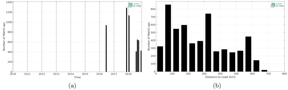
Figure 1: Number of match-ups between TSG-LEGOS-DM and CCI L4 Merged-OI v1.8 - 30-day running (ESA) SSS as a function of time (a) and as function of the distance to coast (b) over the Congo river plume Pi-MEP region and for the full satellite product period.
