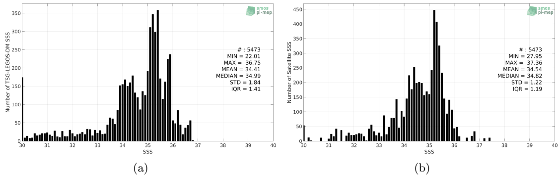
Figure 2: Histograms of SSS from TSG-LEGOS-DM (a) and CCI L4 Merged-OI v1.8 - 30-day running (ESA) (b) considering all match-up pairs per bins of 0.1 over the Congo river plume Pi-MEP region and for the full satellite product period.
