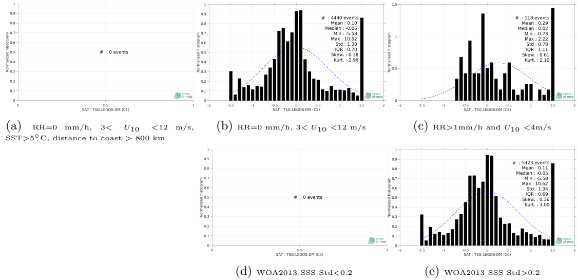
Figure 13: Normalized histogram of \Delta\text{SSS} (CCI-L4-ESA-MERGED-OI-V1.8-30DAY-RUNNING - TSG-LEGOS-DM) for 5 different subdatasets corresponding to: RR=0 mm/h, 3 < U_{10} < 12 m/s, SST > 5^{\circ}\text{C} , distance to coast > 800 km (a), RR=0 mm/h, 3 < U_{10} < 12 m/s (b), RR > 1 mm/h and U_{10} < 4 m/s (c), WOA2013 SSS Std < 0.2 (d), WOA2013 SSS Std > 0.2 (e).
