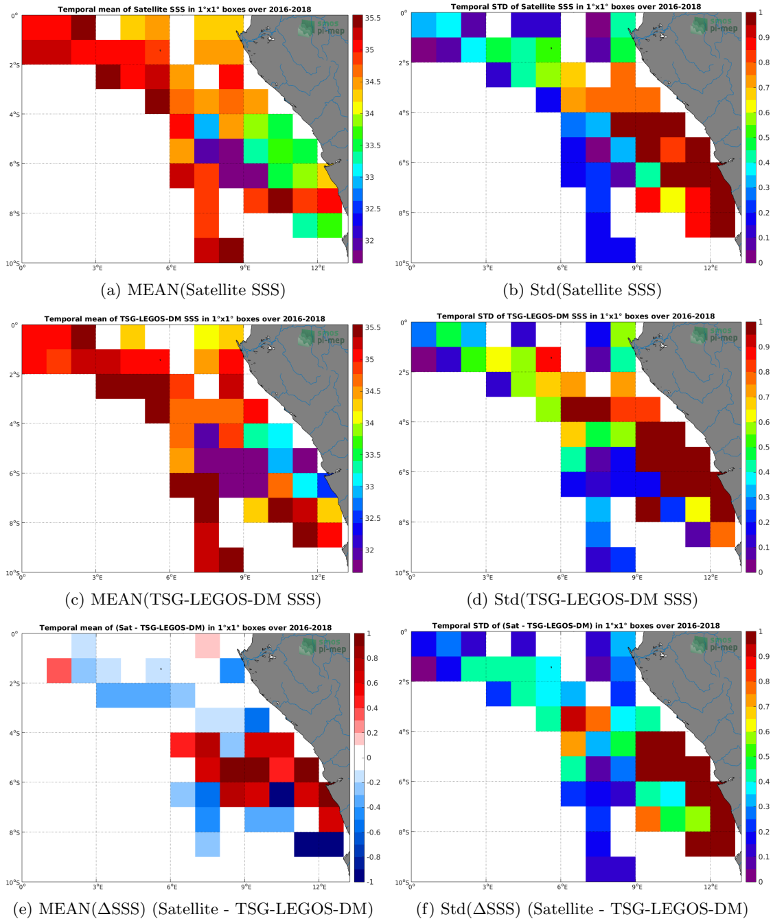
Figure 6: Temporal mean (left) and Std (right) of SSS from CCI-L4-ESA-MERGED-OI-V1.8-30DAY-RUNNING (top), TSG-LEGOS-DM (middle), and of \Delta SSS (Satellite - TSG-LEGOS-DM). Only match-up pairs are used to generate these maps.
