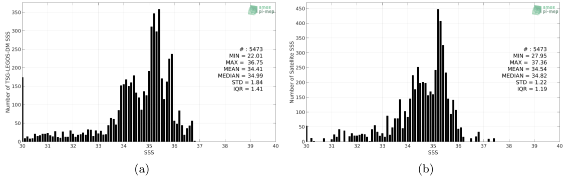
Figure 2: Histograms of SSS from TSG-LEGOS-DM (a) and CCI-L4-ESA-MERGED-OI-V1.8-30DAY-RUNNING (b) considering all match-up pairs per bins of 0.1 over the Congo river plume Pi-MEP region and for the full satellite product period.
