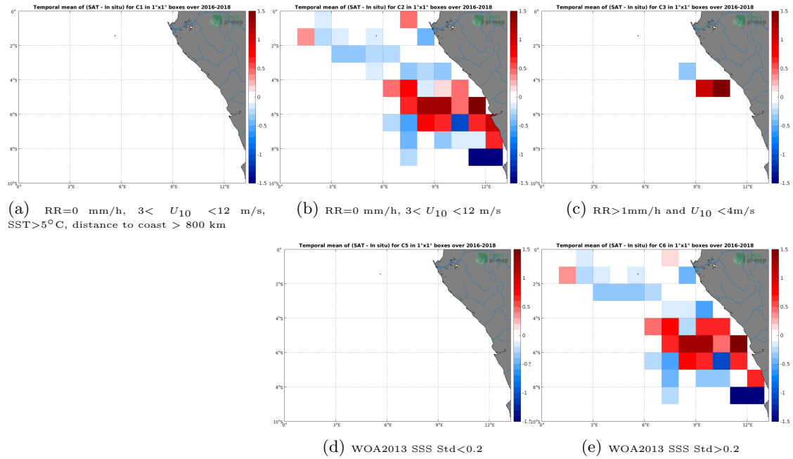
Figure 12: Temporal mean gridded over spatial boxes of size 1^\circ \times 1^\circ of \Delta SSS (CCI-L4-ESA-MERGED-OI-V1.8-30DAY-RUNNING - TSG-LEGOS-DM) for 5 different subdatasets corresponding to:RR=0 mm/h, 3 < U_{10} < 12 m/s, SST > 5^\circ\text{C} , distance to coast > 800 km (a), RR=0 mm/h, 3 < U_{10} < 12 m/s (b), RR > 1 mm/h and U_{10} < 4 m/s (c), WOA2013 SSS Std < 0.2 (d), WOA2013 SSS Std > 0.2 (e).
