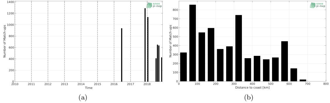
Figure 1: Number of match-ups between TSG-LEGOS-DM and CCI-L4-ESA-MERGED-OI-V1.8-30DAY-RUNNING SSS as a function of time (a) and as function of the distance to coast (b) over the Congo river plume Pi-MEP region and for the full satellite product period.
