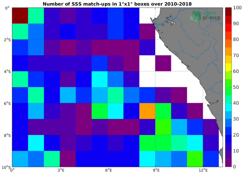
Figure 4: Number of SSS match-ups between Argo SSS and the CCI L4 Merged-OI v1.8 - 30-day running (ESA) SSS product for the Congo river plume Pi-MEP region over 1°x1° boxes and for the full satellite product period.
