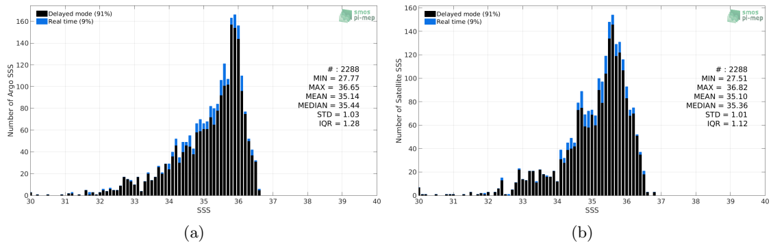
Figure 2: Histograms of SSS from Argo (a) and CCI L4 Merged-OI v1.8 - 30-day running (ESA) (b) considering all match-up pairs per bins of 0.1 over the Congo river plume Pi-MEP region and for the full satellite product period.
