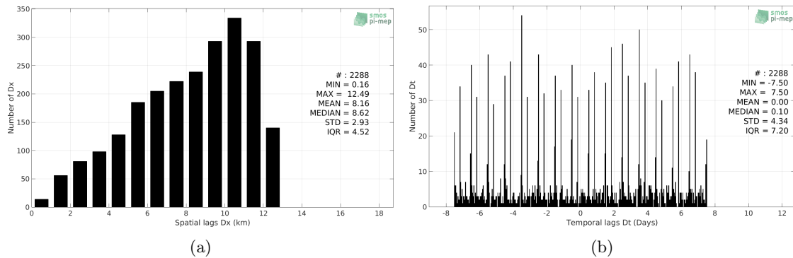
Figure 5: Histograms of the spatial (a) and temporal (b) lags between the time of the Argo measurements and the date of the corresponding CCI L4 Merged-OI v1.8 - 30-day running (ESA) SSS product.
