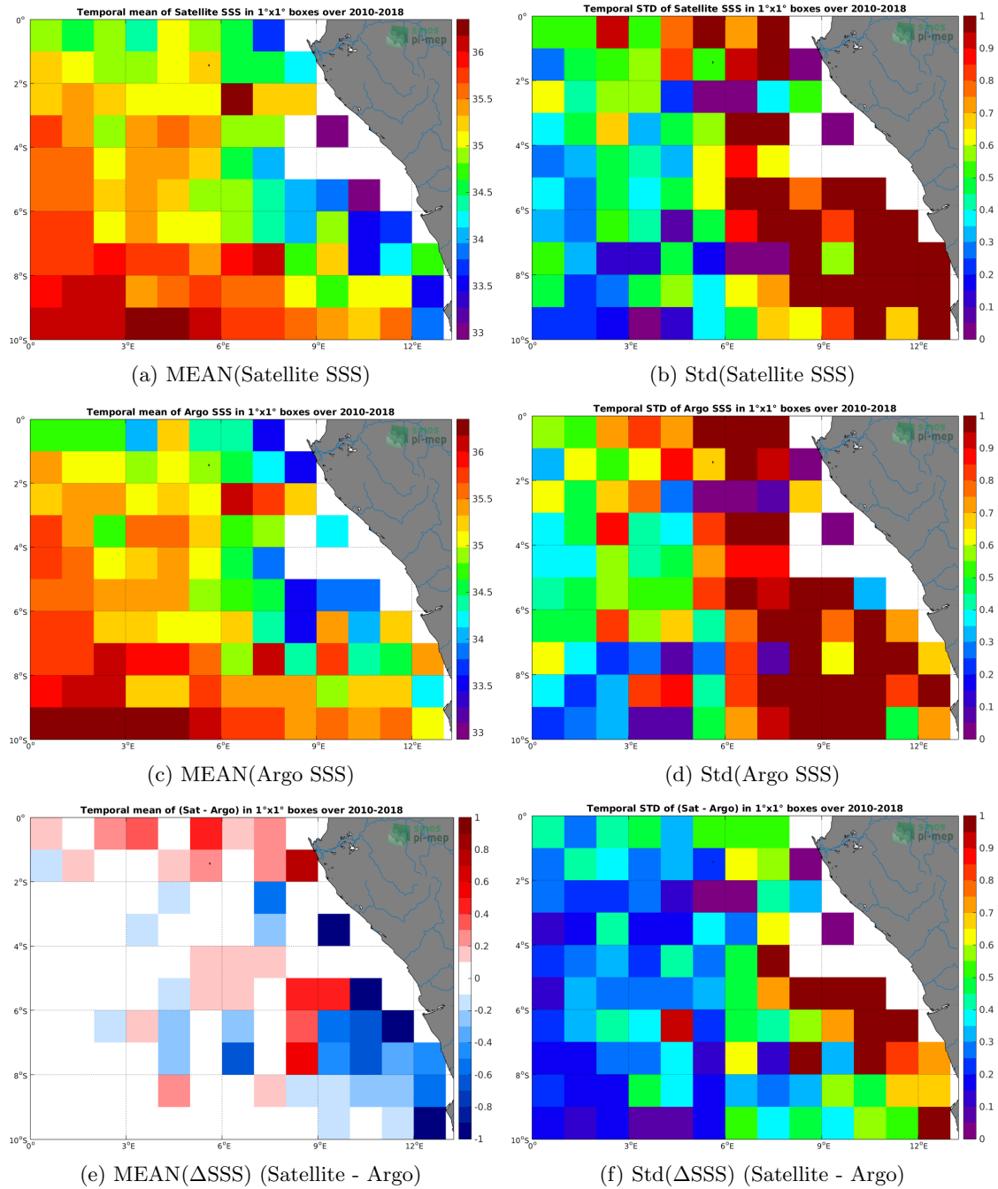
Figure 6: Temporal mean (left) and Std (right) of SSS from CCI L4 Merged-OI v1.8 - 30-day running (ESA) (top), Argo (middle), and of \Delta SSS (Satellite - Argo). Only match-up pairs are used to generate these maps.
