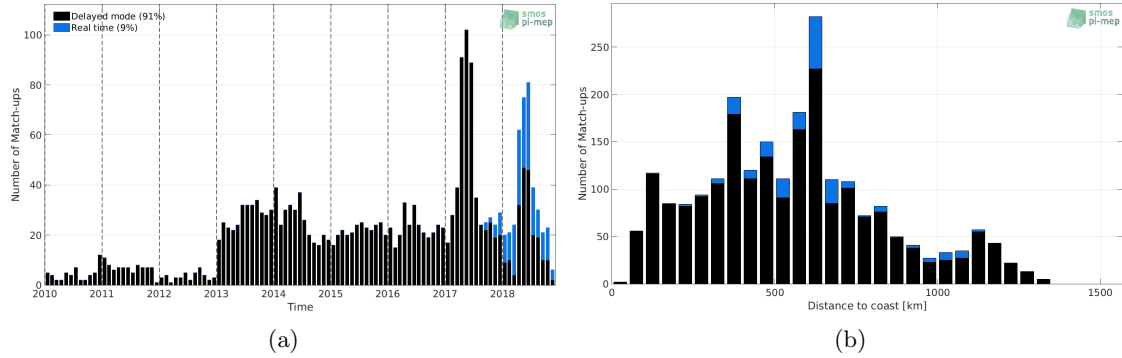
Figure 1: Number of match-ups between Argo and CCI L4 Merged-OI v1.8 - 30-day running (ESA) SSS as a function of time (a) and as function of the distance to coast (b) over the Congo river plume Pi-MEP region and for the full satellite product period.
