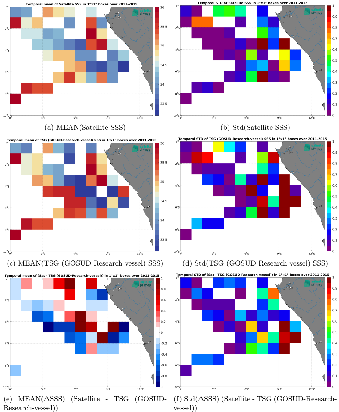
Figure 7: Temporal mean (left) and Std (right) of SSS from Aquarius SSS L4 OI v5 - Weekly (IPRC) (top), TSG (GOSUD-Research-vessel) (middle), and of \Delta SSS (Satellite - TSG (GOSUD-Research-vessel)). Only match-up pairs are used to generate these maps.
