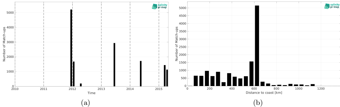
Figure 2: Number of match-ups between TSG (GOSUD-Research-vessel) and Aquarius SSS L4 OI v5 - Weekly (IPRC) SSS as a function of time (a) and as function of the distance to coast (b) over the Congo river plume Pi-MEP region and for the full satellite product period.
