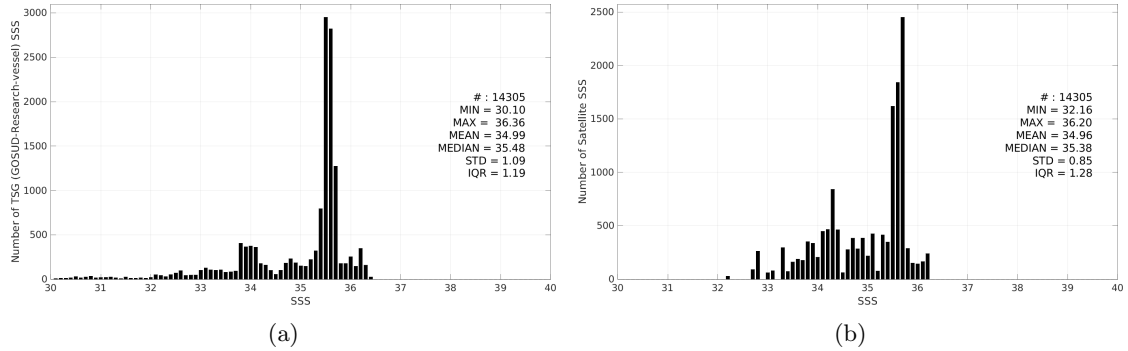
Figure 3: Histograms of SSS from TSG (GOSUD-Research-vessel) (a) and Aquarius SSS L4 OI v5 - Weekly (IPRC) (b) considering all match-up pairs per bins of 0.1 over the Congo river plume Pi-MEP region and for the full satellite product period.
