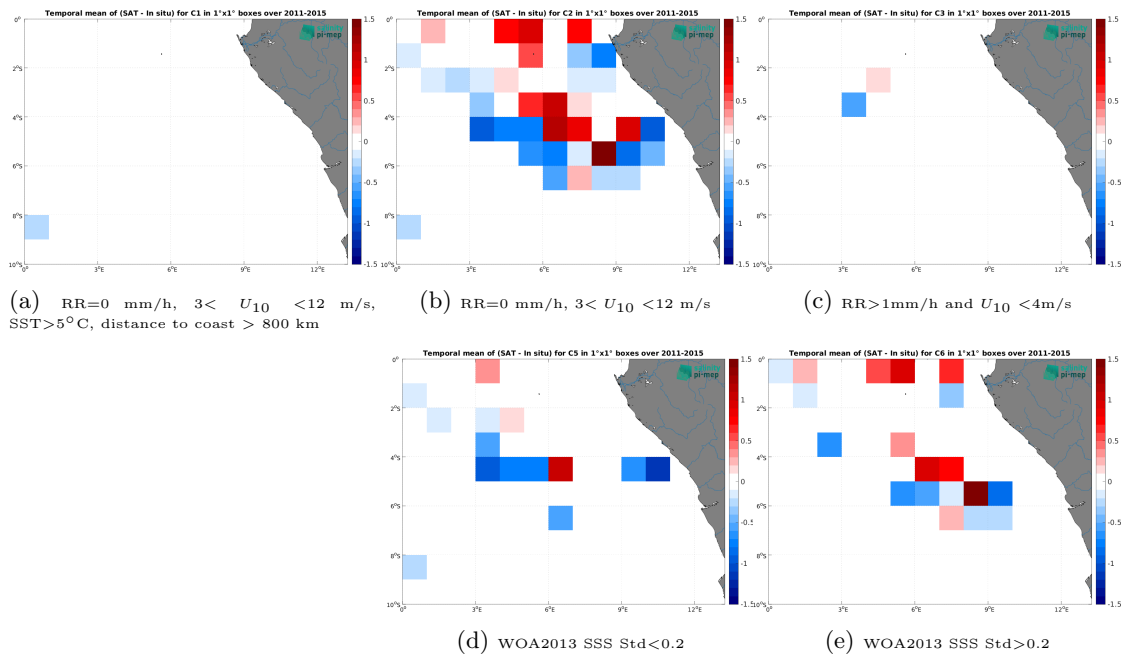
Figure 14: Temporal mean gridded over spatial boxes of size 1^\circ \times 1^\circ of \Delta SSS (Aquarius SSS L4 OI v5 - Weekly (IPRC) - TSG (GOSUD-Research-vessel)) for 5 different subdatasets corresponding to:RR=0 mm/h, 3 < U_{10} < 12 m/s, SST>5°C, distance to coast > 800 km (a), RR=0 mm/h, 3 < U_{10} < 12 m/s (b), RR>1mm/h and U_{10} < 4 m/s (c), WOA2013 SSS Std<0.2 (d), WOA2013 SSS Std>0.2 (e).
