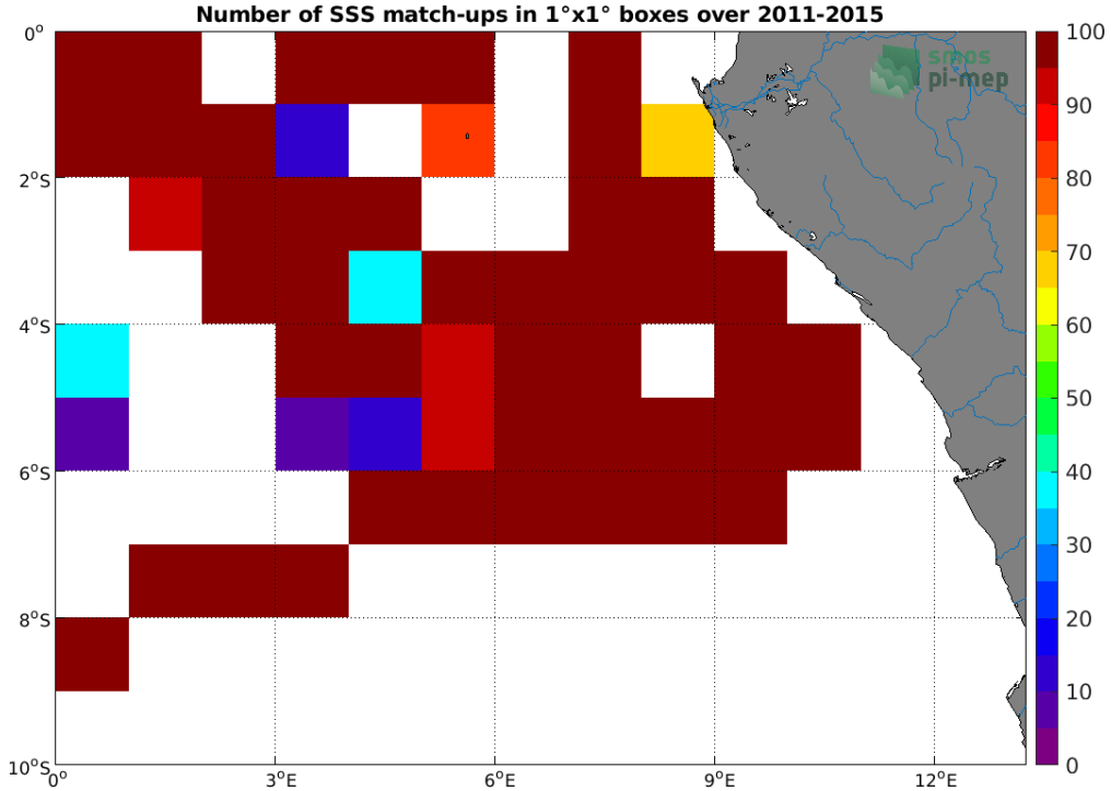
Figure 4: Number of SSS match-ups between TSG (GOSUD-Research-vessel) SSS and the Aquarius SSS L4 OI v5 - Monthly (IPRC) SSS product for the Congo river plume Pi-MEP region over 1^\circ \times 1^\circ boxes and for the full satellite product period.
