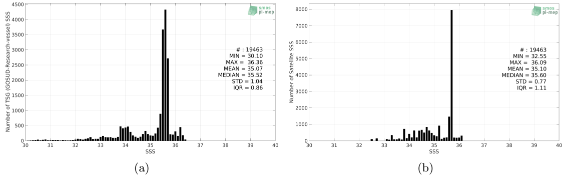
Figure 2: Histograms of SSS from TSG (GOSUD-Research-vessel) (a) and Aquarius SSS L4 OI v5 - Monthly (IPRC) (b) considering all match-up pairs per bins of 0.1 over the Congo river plume Pi-MEP region and for the full satellite product period.
