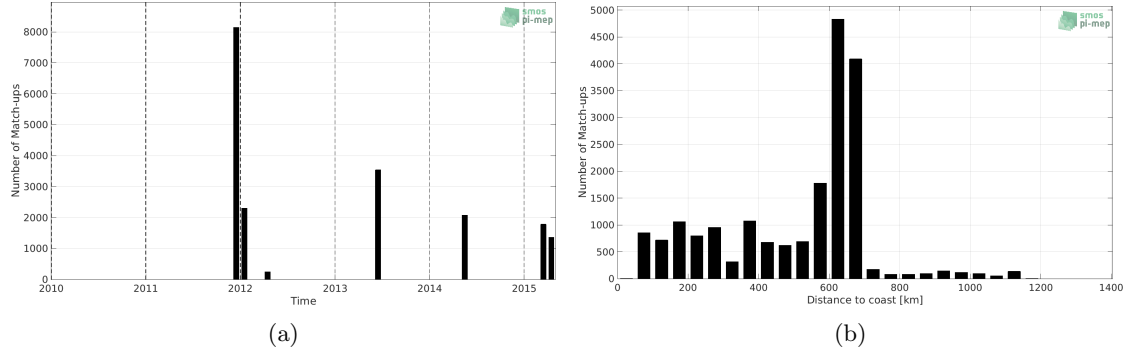
Figure 1: Number of match-ups between TSG (GOSUD-Research-vessel) and Aquarius SSS L4 OI v5 - Monthly (IPRC) SSS as a function of time (a) and as function of the distance to coast (b) over the Congo river plume Pi-MEP region and for the full satellite product period.
