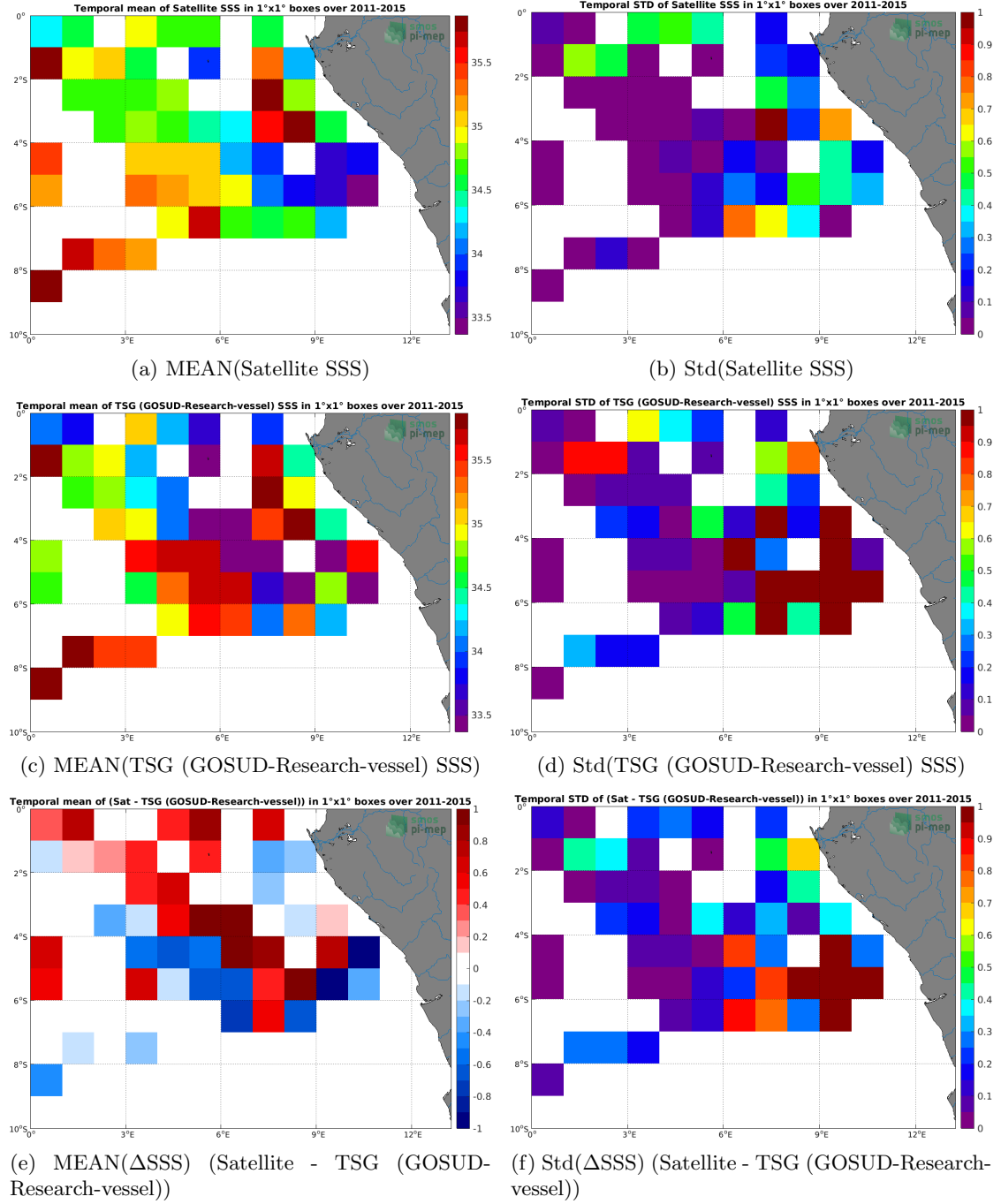
Figure 6: Temporal mean (left) and Std (right) of SSS from Aquarius SSS L4 OI v5 - Monthly (IPRC) (top), TSG (GOSUD-Research-vessel) (middle), and of \Delta SSS (Satellite - TSG (GOSUD-Research-vessel)). Only match-up pairs are used to generate these maps.
