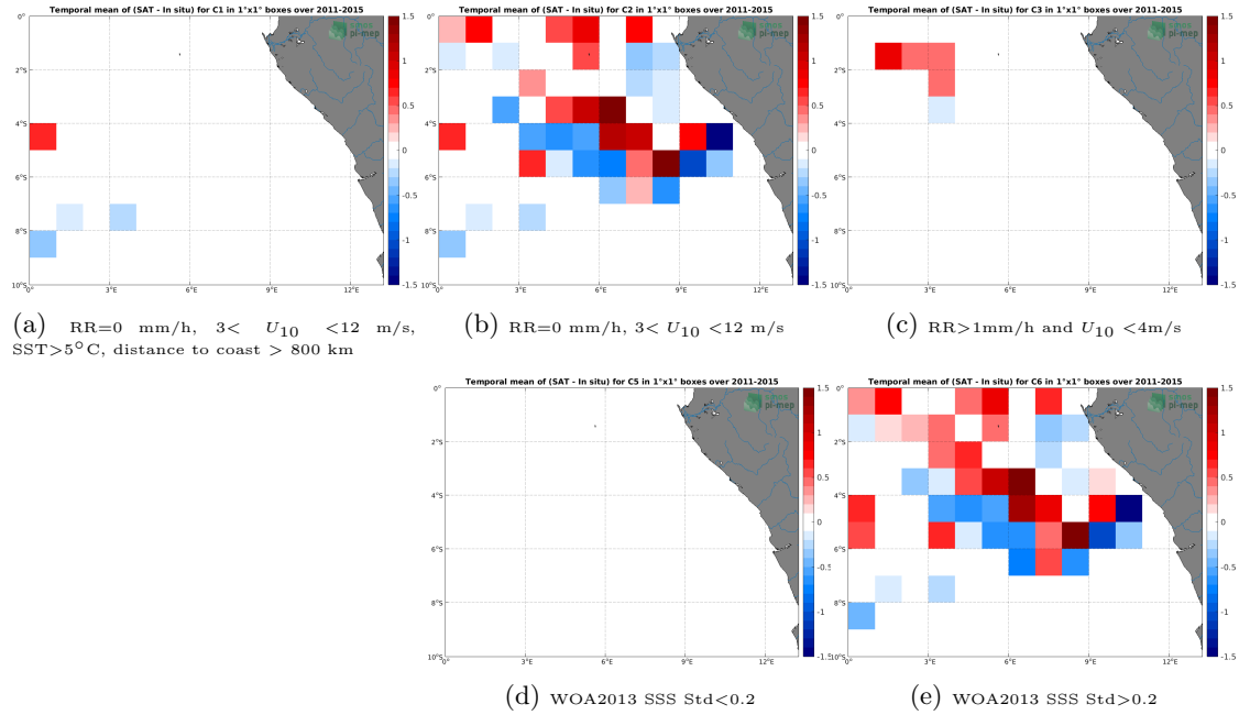
Figure 12: Temporal mean gridded over spatial boxes of size 1^\circ \times 1^\circ of \Delta SSS (Aquarius SSS L4 OI v5 - Monthly (IPRC) - TSG (GOSUD-Research-vessel)) for 5 different subdatasets corresponding to: RR=0 mm/h, 3 < U_{10} < 12 m/s, SST > 5^\circ\text{C} , distance to coast > 800 km (a), RR=0 mm/h, 3 < U_{10} < 12 m/s (b), RR > 1 mm/h and U_{10} < 4 m/s (c), WOA2013 SSS Std < 0.2 (d), WOA2013 SSS Std > 0.2 (e).
