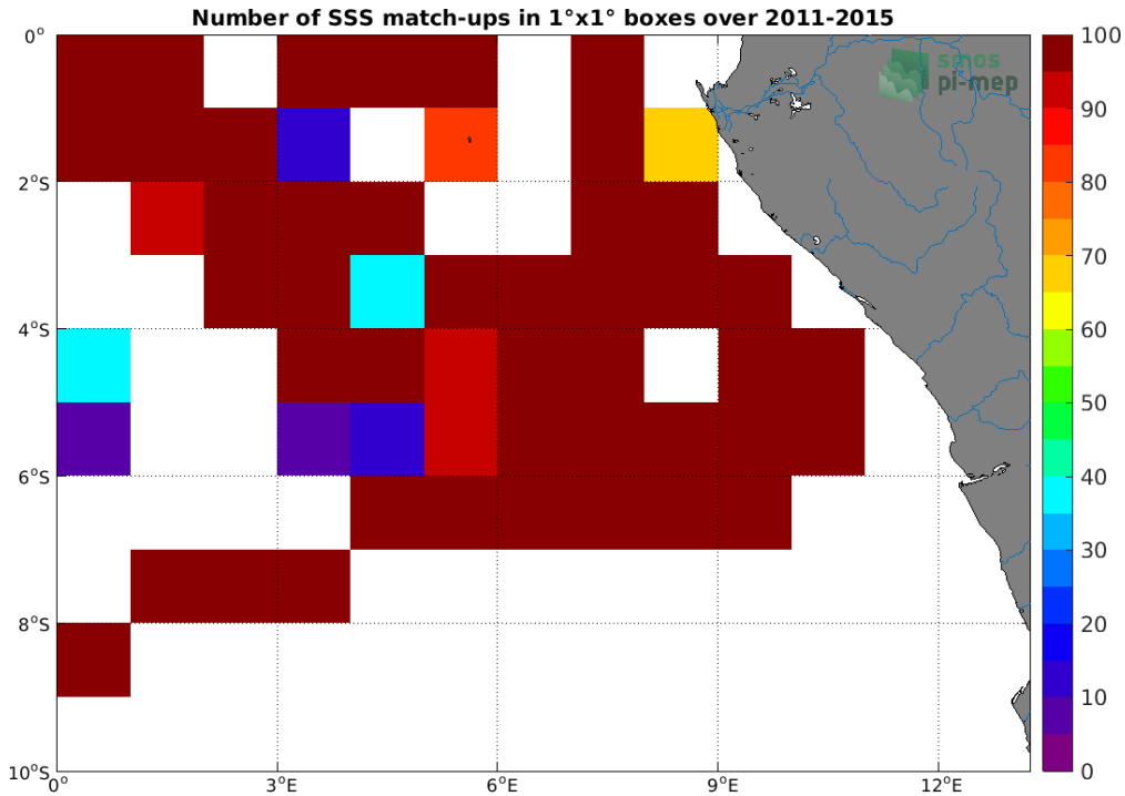
Figure 4: Number of SSS match-ups between TSG (GOSUD-Research-vessel) SSS and the Aquarius SSS L4 OI v5 - Monthly (IPRC) SSS product for the Congo river plume Pi-MEP region over 1°x1° boxes and for the full satellite product period.
