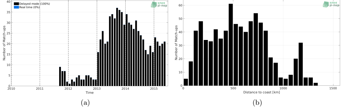
Figure 1: Number of match-ups between Argo and Aquarius-L4-IPRC-V5-MONTHLY SSS as a function of time (a) and as function of the distance to coast (b) over the Congo river plume Pi-MEP region and for the full satellite product period.
