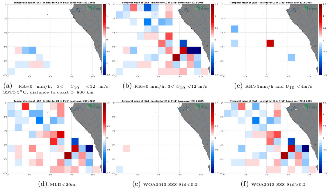
Figure 12: Temporal mean gridded over spatial boxes of size 1^\circ \times 1^\circ of \Delta SSS (Aquarius-L4-IPRC-V5-MONTHLY - Argo) for 6 different subdatasets corresponding to: RR=0 mm/h, 3 < U_{10} < 12 m/s, SST > 5^\circ\text{C} , distance to coast > 800 km (a), RR=0 mm/h, 3 < U_{10} < 12 m/s (b), RR > 1 mm/h and U_{10} < 4 m/s (c), MLD < 20 m (d), WOA2013 SSS Std < 0.2 (e), WOA2013 SSS Std > 0.2 (f).
