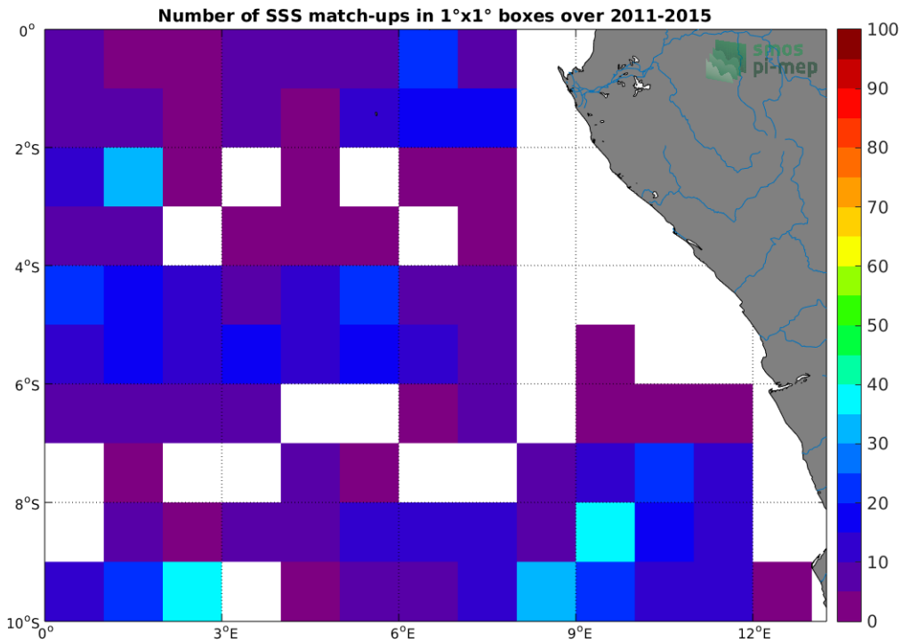
Figure 4: Number of SSS match-ups between Argo SSS and the Aquarius-L4-IPRC-V5-MONTHLY SSS product for the Congo river plume Pi-MEP region over 1°x1° boxes and for the full satellite product period.
