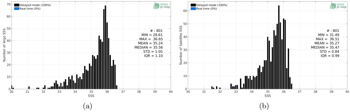
Figure 2: Histograms of SSS from Argo (a) and Aquarius-L4-IPRC-V5-MONTHLY (b) considering all match-up pairs per bins of 0.1 over the Congo river plume Pi-MEP region and for the full satellite product period.
