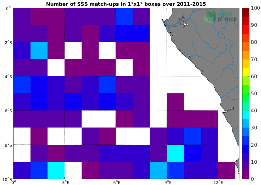
Figure 4: Number of SSS match-ups between Argo SSS and the Aquarius-L4-IPRC-V5-MONTHLY SSS product for the Congo river plume Pi-MEP region over 1^\circ \times 1^\circ boxes and for the full satellite product period.
