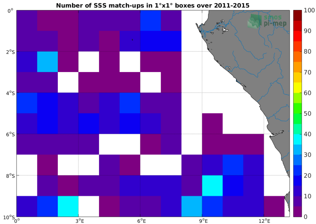
Figure 4: Number of SSS match-ups between Argos SSS and the Aquarius-L4-IPRC-V5-MONTHLY SSS product for the Congo river plume Pi-MEP region over 1^\circ \times 1^\circ boxes and for the full satellite product period.
