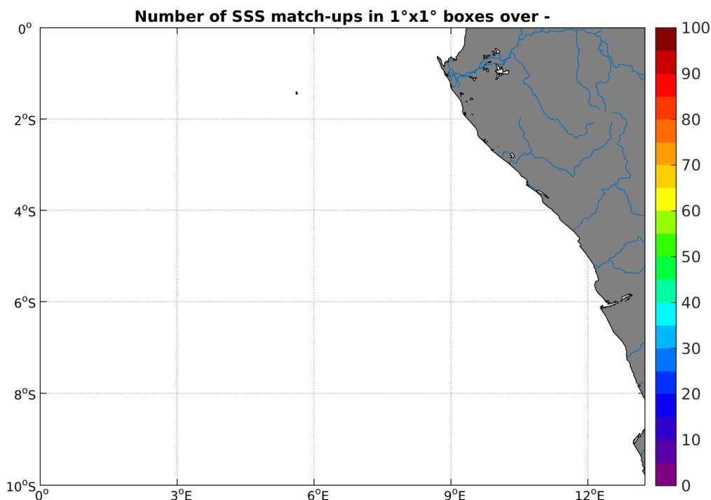
Figure 4: Number of SSS match-ups between TSG-SAMOS SSS and the Aquarius-L4-IPRC-V4-WEEKLY SSS product for the Congo river plume Pi-MEP region over 1^\circ \times 1^\circ boxes and for the full satellite product period.
