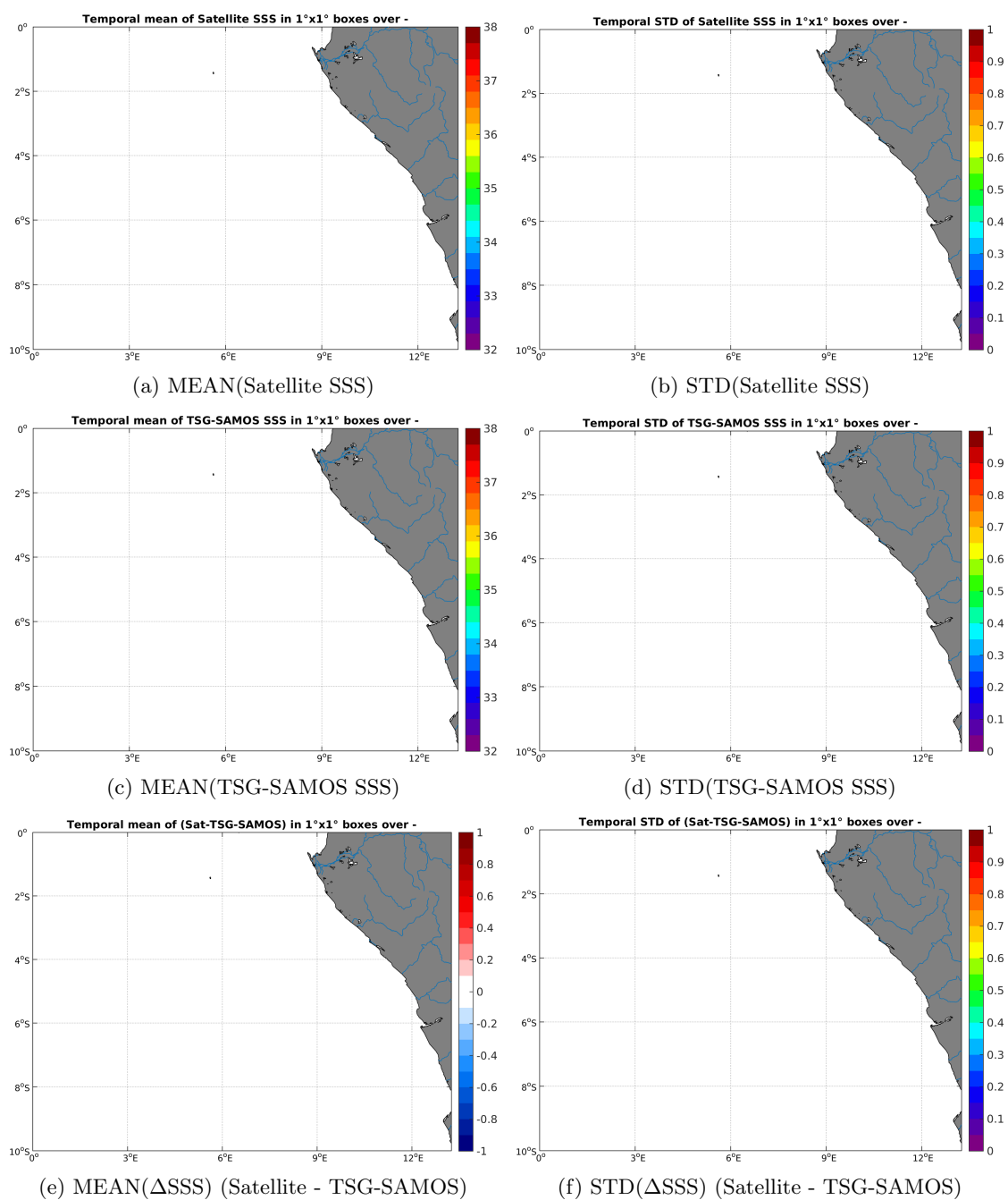
Figure 6: Temporal mean (left) and STD (right) of SSS from Aquarius-L4-IPRC-V4-WEEKLY (top), TSG-SAMOS (middle), and of \Delta SSS (Satellite - TSG-SAMOS). Only match-up pairs are used to generate these maps.
