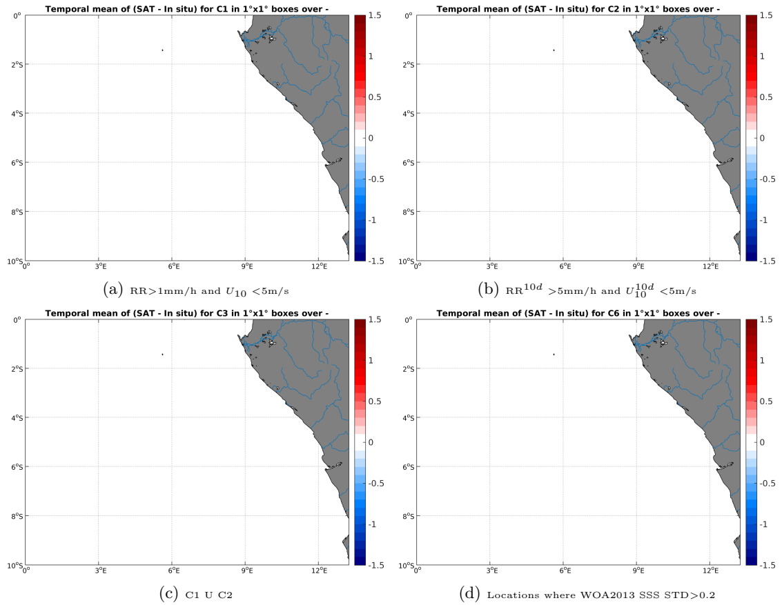
Figure 12: Temporal mean gridded over spatial boxes of size 1^\circ \times 1^\circ of \Delta SSS (Aquarius-L4-IPRC-V4-WEEKLY - TSG-SAMOS) for 4 different subdatasets corresponding to:RR >1 mm/h and U_{10} < 5 m/s (a), RR ^{10d} > 5 mm/h and U_{10}^{10d} < 5 m/s (b), C1 U C2 (c),Locations where WOA2013 SSS STD >0.2 (d).
