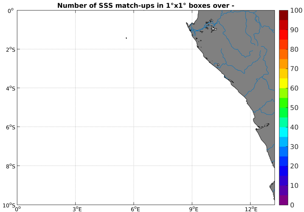
Figure 4: Number of SSS match-ups between TSG-LEGOS-DM SSS and the Aquarius-L4-IPRC-V4-WEEKLY SSS product for the Congo river plume Pi-MEP region over 1^\circ \times 1^\circ boxes and for the full satellite product period.
