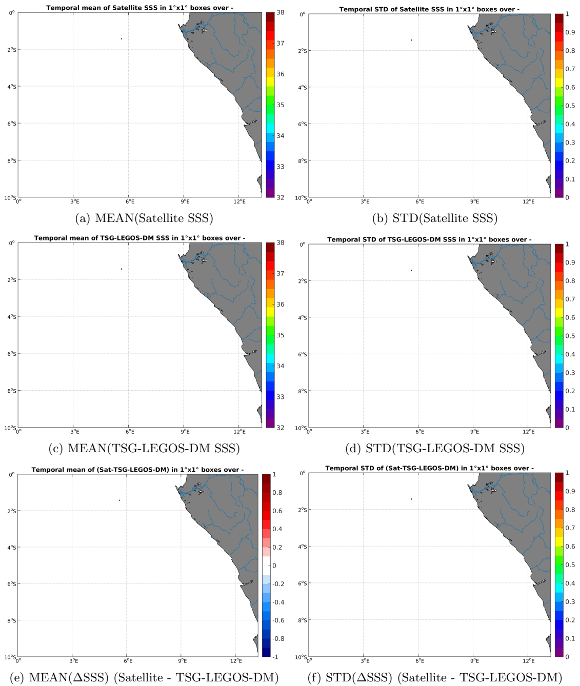
Figure 6: Temporal mean (left) and STD (right) of SSS from Aquarius-L4-IPRC-V4-WEEKLY (top), TSG-LEGOS-DM (middle), and of \Delta SSS (Satellite - TSG-LEGOS-DM). Only match-up pairs are used to generate these maps.
