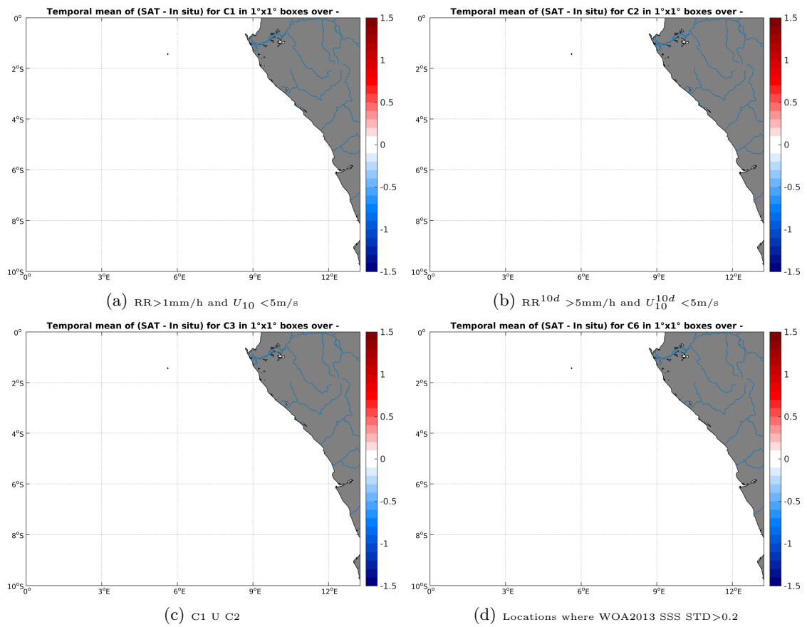
Figure 12: Temporal mean gridded over spatial boxes of size 1^\circ \times 1^\circ of \Delta SSS (Aquarius-L4-IPRC-V4-WEEKLY - TSG-LEGOS-DM) for 4 different subdatasets corresponding to:RR >1 mm/h and U_{10} < 5 m/s (a), RR ^{10d} > 5 mm/h and U_{10}^{10d} < 5 m/s (b), C1 U C2 (c),Locations where WOA2013 SSS STD >0.2 (d).
