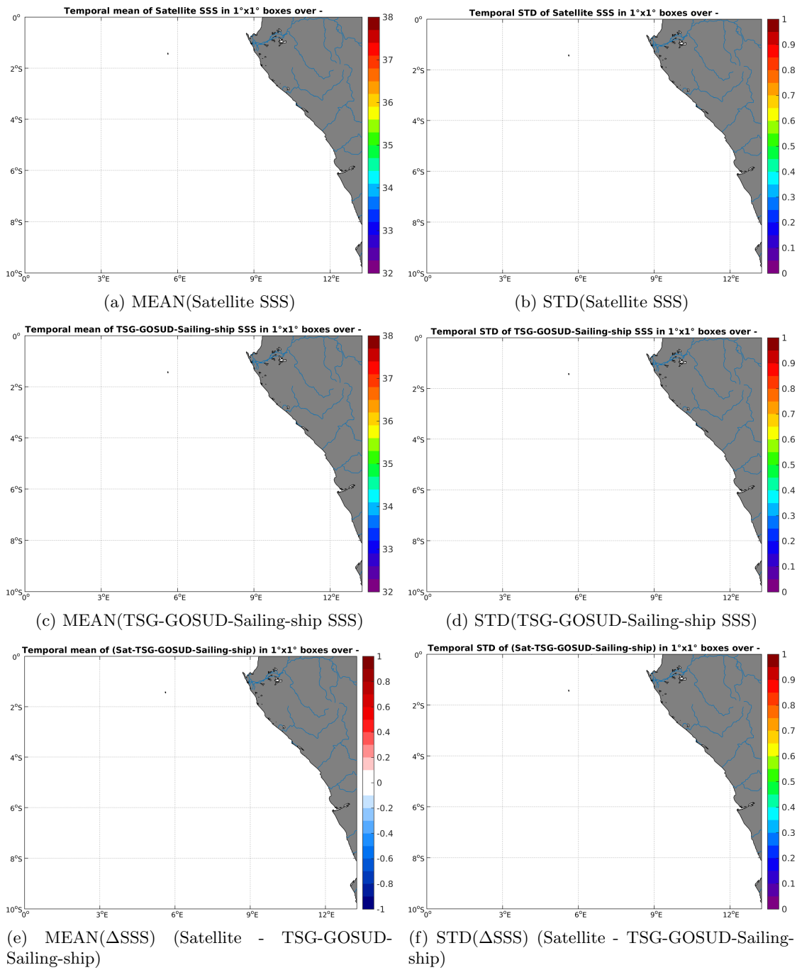
Figure 6: Temporal mean (left) and STD (right) of SSS from Aquarius-L4-IPRC-V4-WEEKLY (top), TSG-GOSUD-Sailing-ship (middle), and of \Delta SSS (Satellite - TSG-GOSUD-Sailing-ship). Only match-up pairs are used to generate these maps.
