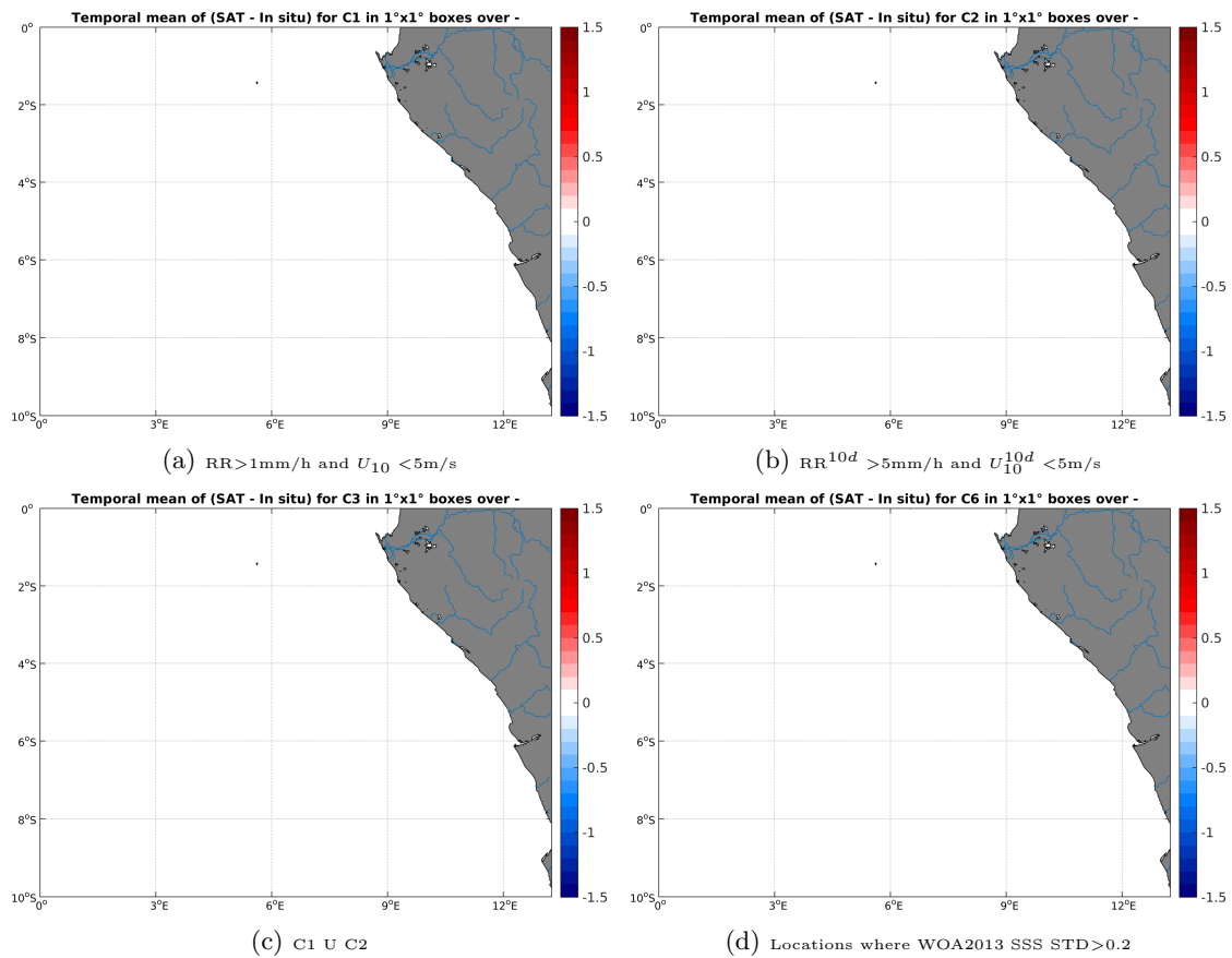
Figure 12: Temporal mean gridded over spatial boxes of size 1^\circ \times 1^\circ of \Delta SSS (Aquarius-L4-IPRC-V4-WEEKLY - TSG-GOSUD-Sailing-ship) for 4 different subdatasets corresponding to:RR >1 mm/h and U_{10} < 5 m/s (a), RR ^{10d} > 5 mm/h and U_{10}^{10d} < 5 m/s (b), C1 U C2 (c),Locations where WOA2013 SSS STD >0.2 (d).
