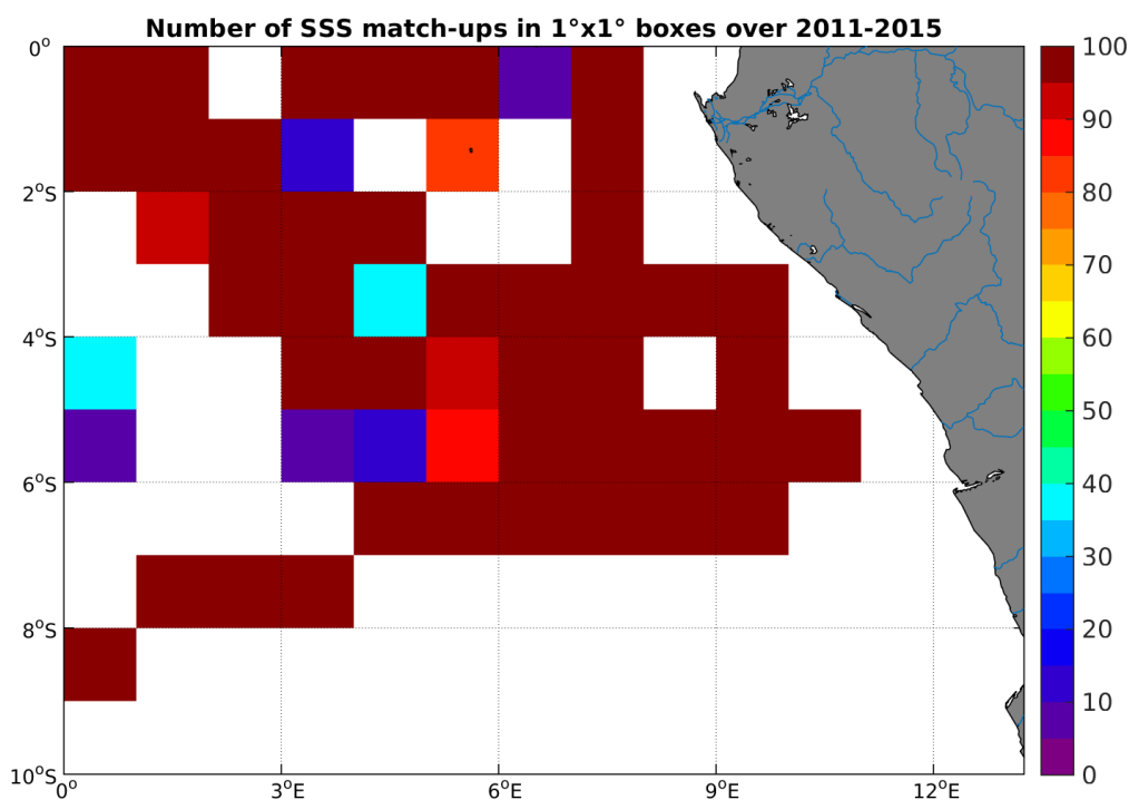
Figure 4: Number of SSS match-ups between TSG-GOSUD-Research-vessel SSS and the Aquarius-L4-IPRC-V4-WEEKLY SSS product for the Congo river plume Pi-MEP region over 1°x1° boxes and for the full satellite product period.
