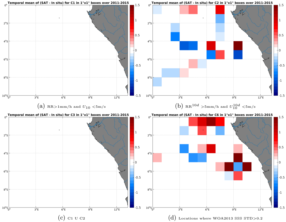
Figure 12: Temporal mean gridded over spatial boxes of size 1°x1° of \Delta SSS (Aquarius-L4-IPRC-V4-WEEKLY - TSG-GOSUD-Research-vessel) for 4 different subdatasets corresponding to: RR > 1mm/h and U_{10} < 5\text{m/s} (a), RR^{10d} > 5\text{mm/h} and U_{10}^{10d} < 5\text{m/s} (b), C1 U C2 (c), Locations where WOA2013 SSS STD > 0.2 (d).
