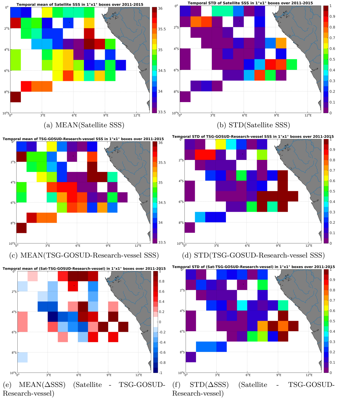
Figure 6: Temporal mean (left) and STD (right) of SSS from Aquarius-L4-IPRC-V4-WEEKLY (top), TSG-GOSUD-Research-vessel (middle), and of \Delta SSS (Satellite - TSG-GOSUD-Research-vessel). Only match-up pairs are used to generate these maps.
