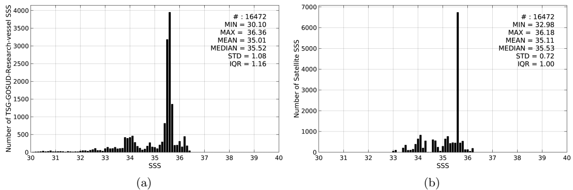
Figure 2: Histograms of SSS from TSG-GOSUD-Research-vessel (a) and Aquarius-L4-IPRC-V4-WEEKLY (b) considering all match-up pairs per bins of 0.1 over the Congo river plume Pi-MEP region and for the full satellite product period.
