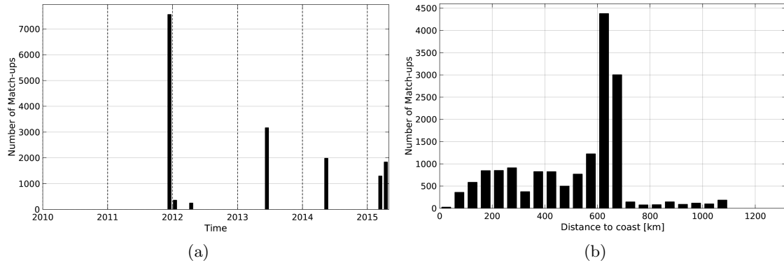
Figure 1: Number of match-ups between TSG-GOSUD-Research-vessel and Aquarius-L4-IPRC-V4-WEEKLY SSS as a function of time (a) and as function of the distance to coast (b) over the Congo river plume Pi-MEP region and for the full satellite product period.
