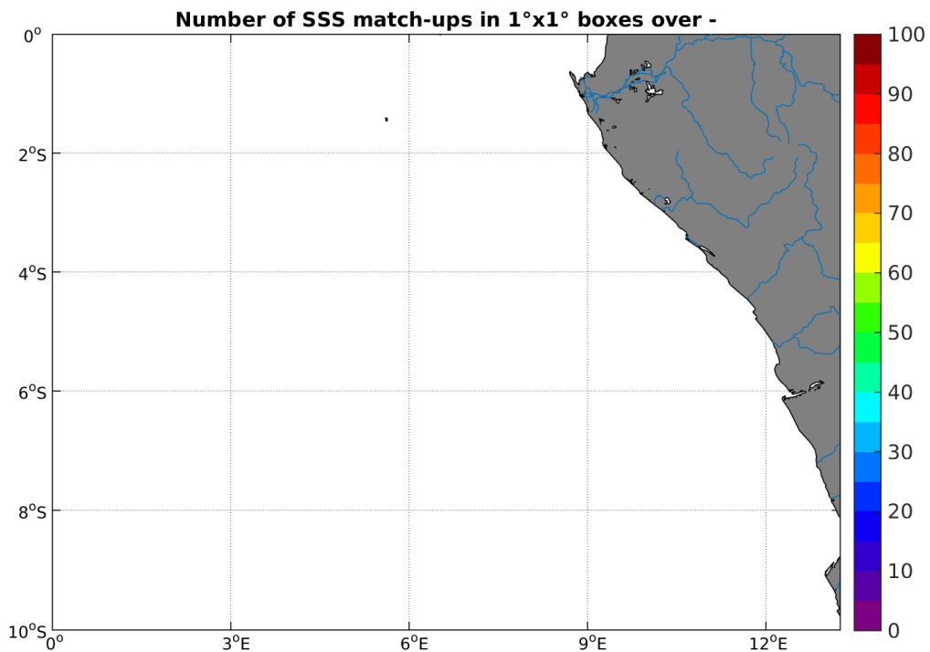
Figure 4: Number of SSS match-ups between Sea mammals SSS and the Aquarius-L4-IPRC-V4-WEEKLY SSS product for the Congo river plume Pi-MEP region over 1^\circ \times 1^\circ boxes and for the full satellite product period.
