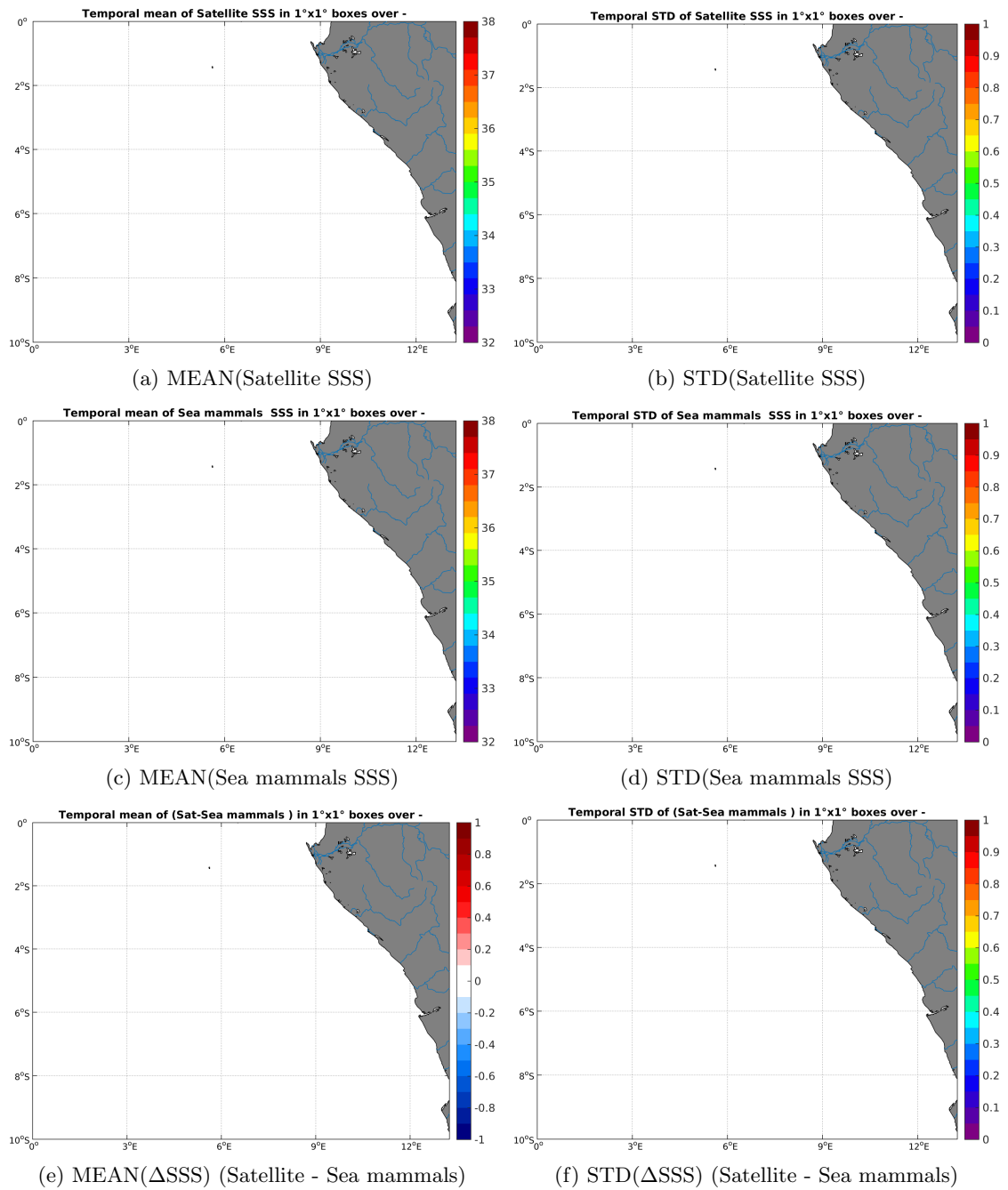
Figure 6: Temporal mean (left) and STD (right) of SSS from Aquarius-L4-IPRC-V4-WEEKLY (top), Sea mammals (middle), and of \Delta SSS (Satellite - Sea mammals). Only match-up pairs are used to generate these maps.
