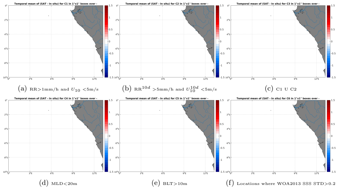
Figure 12: Temporal mean gridded over spatial boxes of size 1^\circ \times 1^\circ of \Delta SSS (Aquarius-L4-IPRC-V4-WEEKLY - Sea mammals) for 6 different subdatasets corresponding to: RR > 1\text{mm/h} and U_{10} < 5\text{m/s} (a), RR^{10d} > 5\text{mm/h} and U_{10}^{10d} < 5\text{m/s} (b), C1 U C2 (c), MLD < 20\text{m} (d), BLT > 10\text{m} (e), Locations where WOA2013 SSS STD > 0.2 (f).
