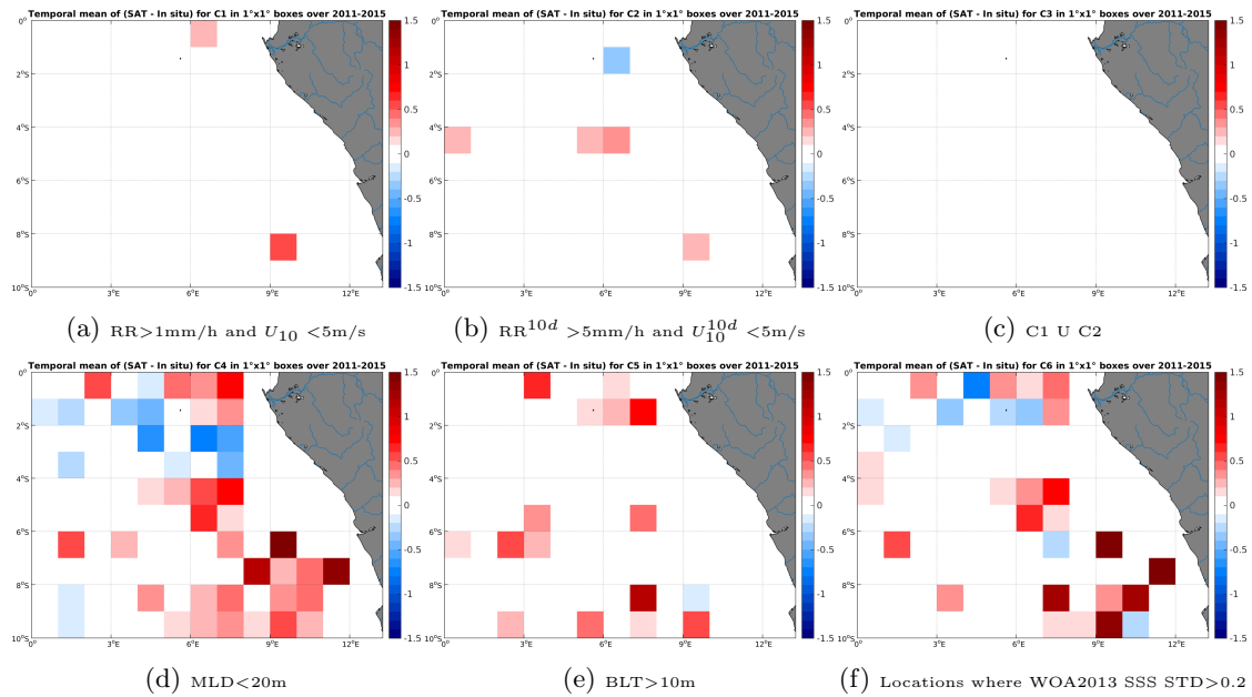
Figure 12: Temporal mean gridded over spatial boxes of size 1^\circ \times 1^\circ of \Delta SSS (Aquarius-L4-IPRC-V4-WEEKLY - Argo) for 6 different subdatasets corresponding to:RR > 1 mm/h and U_{10} < 5 m/s (a), RR^{10d} > 5 mm/h and U_{10}^{10d} < 5 m/s (b), C1 U C2 (c),MLD < 20 m (d),BLT > 10 m (e),Locations where WOA2013 SSS STD > 0.2 (f).
