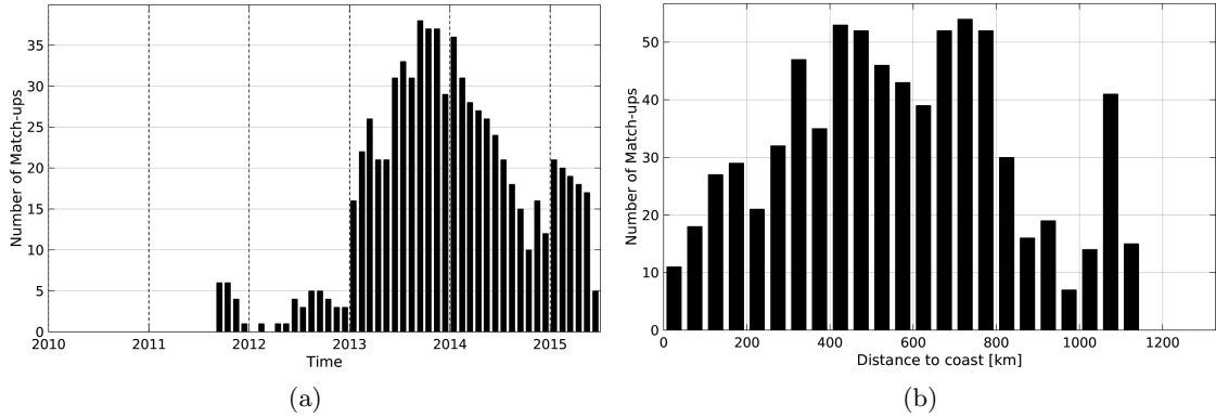
Figure 1: Number of match-ups between Argo and Aquarius-L4-IPRC-V4-WEEKLY SSS as a function of time (a) and as function of the distance to coast (b) over the Congo river plume Pi-MEP region and for the full satellite product period.
