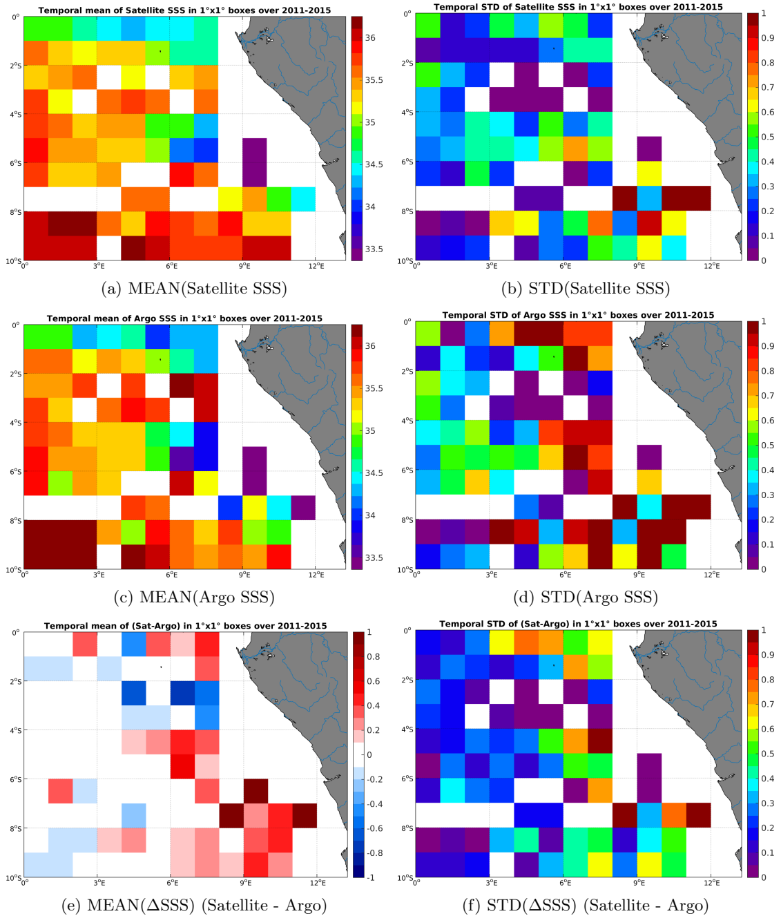
Figure 6: Temporal mean (left) and STD (right) of SSS from Aquarius-L4-IPRC-V4-WEEKLY (top), Argo (middle), and of \Delta SSS (Satellite - Argo). Only match-up pairs are used to generate these maps.
