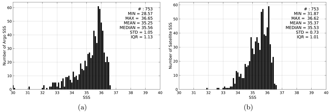
Figure 2: Histograms of SSS from Argo (a) and Aquarius-L4-IPRC-V4-WEEKLY (b) considering all match-up pairs per bins of 0.1 over the Congo river plume Pi-MEP region and for the full satellite product period.
