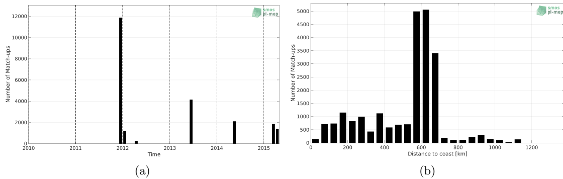
Figure 1: Number of match-ups between TSG (GOSUD-Research-vessel) and Aquarius SSS L3 CAP v5 - 7-Day running (JPL) SSS as a function of time (a) and as function of the distance to coast (b) over the Congo river plume Pi-MEP region and for the full satellite product period.
