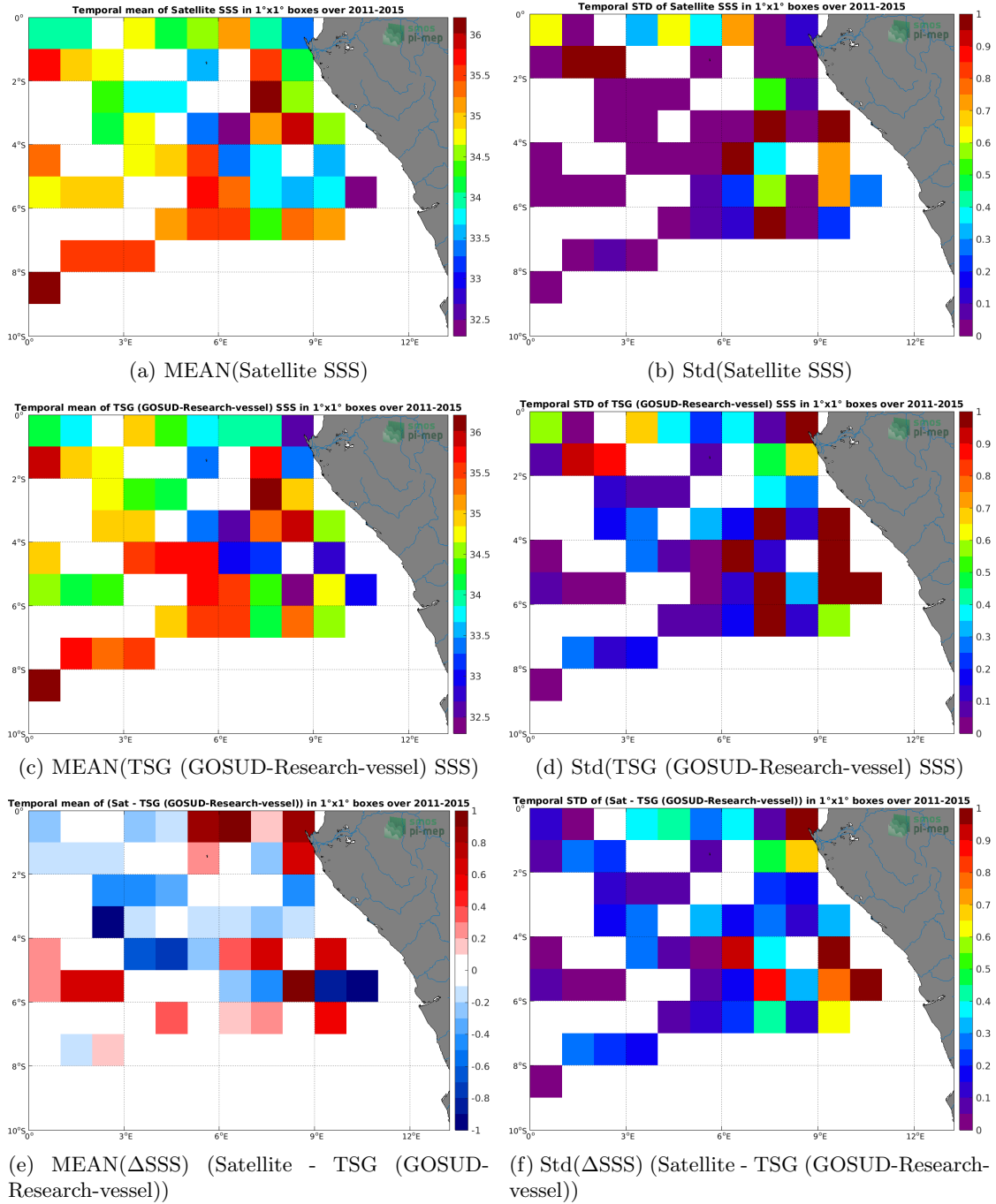
Figure 6: Temporal mean (left) and Std (right) of SSS from Aquarius SSS L3 CAP v5 - 7-Day running (JPL) (top), TSG (GOSUD-Research-vessel) (middle), and of \Delta SSS (Satellite - TSG (GOSUD-Research-vessel)). Only match-up pairs are used to generate these maps.
