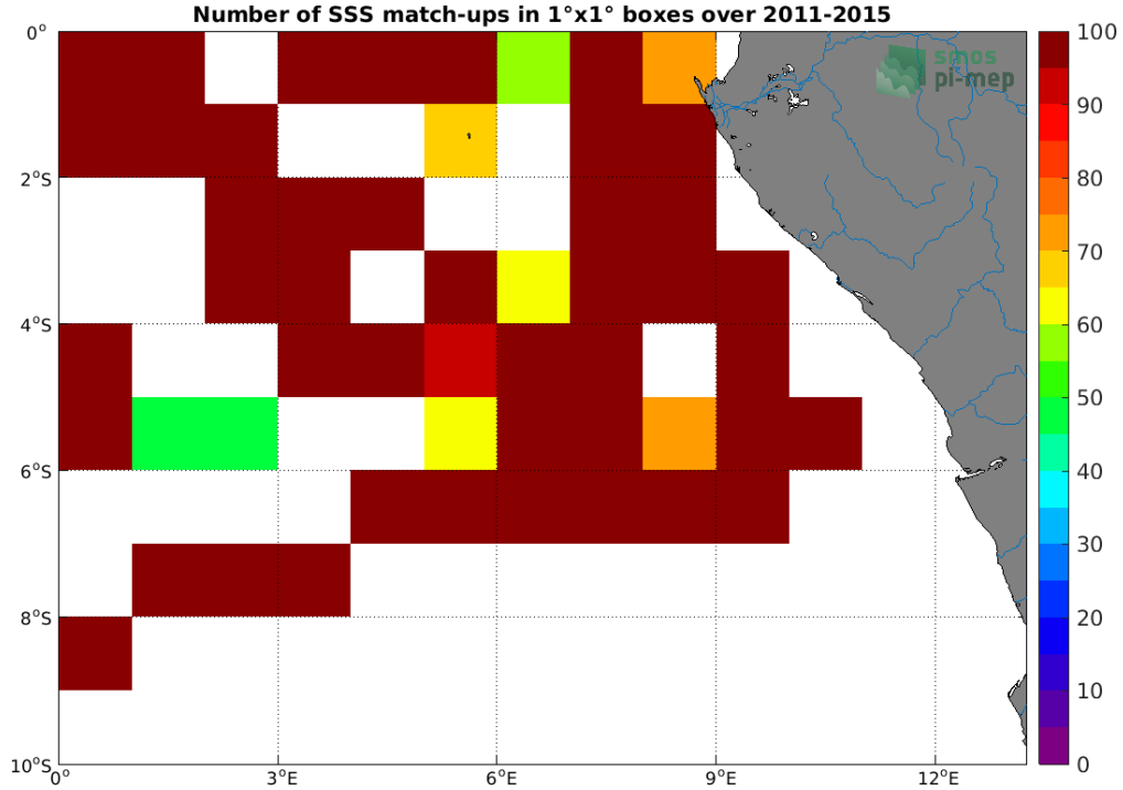
Figure 4: Number of SSS match-ups between TSG (GOSUD-Research-vessel) SSS and the Aquarius SSS L3 CAP v5 - 7-Day running (JPL) SSS product for the Congo river plume Pi-MEP region over 1^\circ \times 1^\circ boxes and for the full satellite product period.
