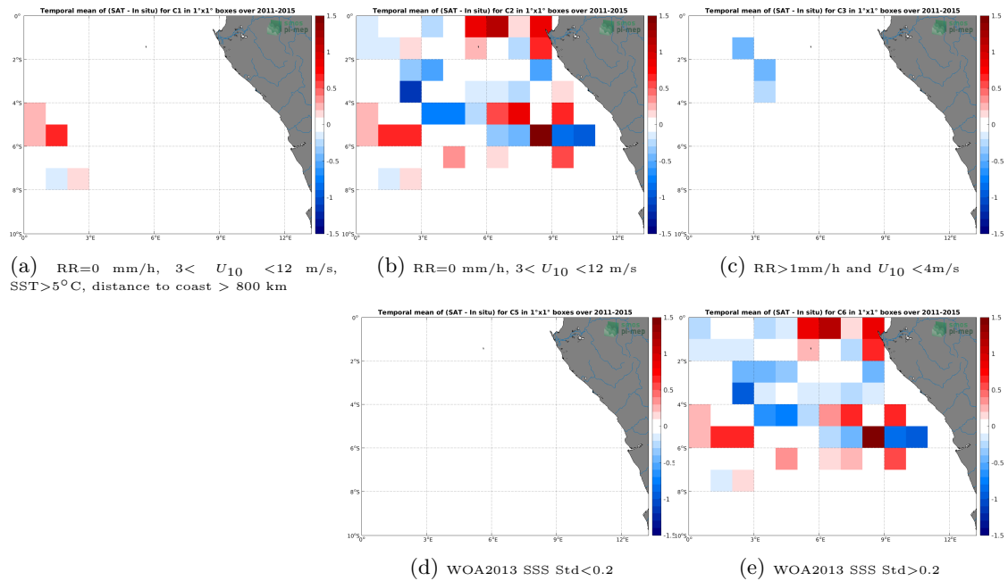
Figure 12: Temporal mean gridded over spatial boxes of size 1^\circ \times 1^\circ of \Delta SSS (Aquarius SSS L3 CAP v5 - 7-Day running (JPL) - TSG (GOSUD-Research-vessel)) for 5 different subdatasets corresponding to: RR=0 mm/h, 3 < U_{10} < 12 m/s, SST > 5^\circ\text{C} , distance to coast > 800 km (a), RR=0 mm/h, 3 < U_{10} < 12 m/s (b), RR > 1 mm/h and U_{10} < 4 m/s (c), WOA2013 SSS Std < 0.2 (d), WOA2013 SSS Std > 0.2 (e).
