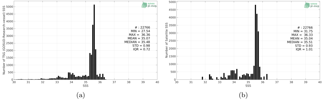
Figure 2: Histograms of SSS from TSG (GOSUD-Research-vessel) (a) and Aquarius SSS L3 CAP v5 - 7-Day running (JPL) (b) considering all match-up pairs per bins of 0.1 over the Congo river plume Pi-MEP region and for the full satellite product period.
