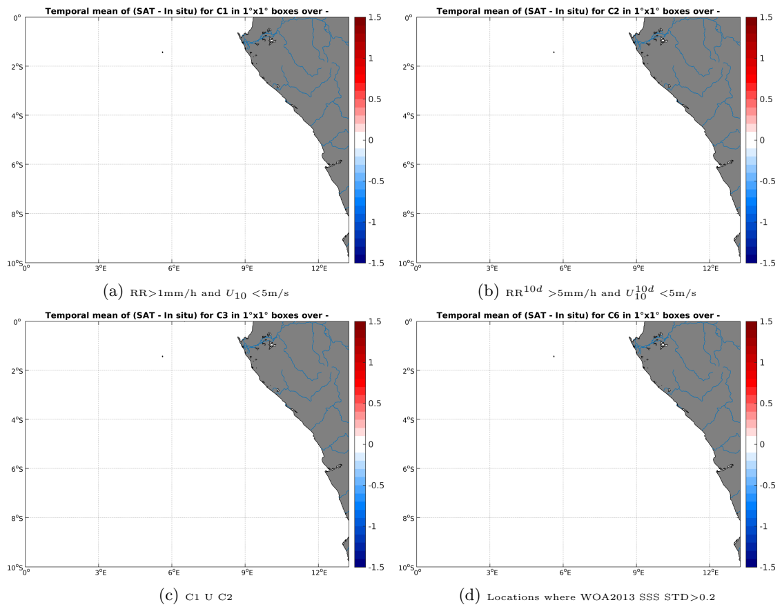
Figure 12: Temporal mean gridded over spatial boxes of size 1^\circ \times 1^\circ of \Delta SSS (Aquarius-L3-JPL-V4-7DAY-RUNNING - TSG-SAMOS) for 4 different subdatasets corresponding to:RR >1 mm/h and U_{10} < 5 m/s (a), RR ^{10d} > 5 mm/h and U_{10}^{10d} < 5 m/s (b), C1 U C2 (c),Locations where WOA2013 SSS STD >0.2 (d).
