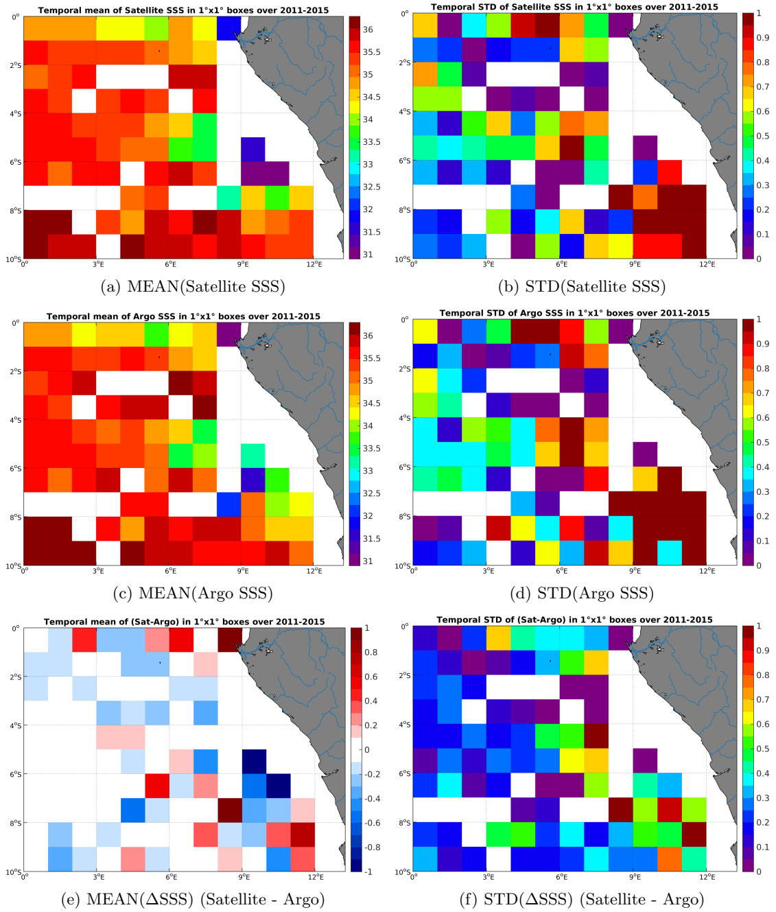
Figure 6: Temporal mean (left) and STD (right) of SSS from Aquarius-L3-JPL-V4-7DAY-RUNNING (top), Argo (middle), and of \Delta SSS (Satellite - Argo). Only match-up pairs are used to generate these maps.
