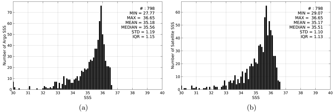
Figure 2: Histograms of SSS from Argo (a) and Aquarius-L3-JPL-V4-7DAY-RUNNING (b) considering all match-up pairs per bins of 0.1 over the Congo river plume Pi-MEP region and for the full satellite product period.
