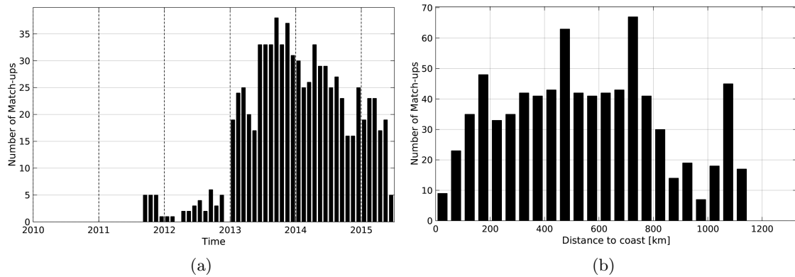
Figure 1: Number of match-ups between Argo and Aquarius-L3-JPL-V4-7DAY-RUNNING SSS as a function of time (a) and as function of the distance to coast (b) over the Congo river plume Pi-MEP region and for the full satellite product period.
