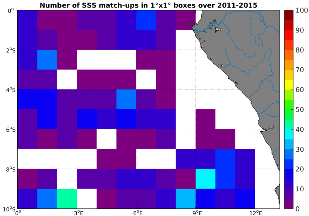
Figure 4: Number of SSS match-ups between Argo SSS and the Aquarius-L3-JPL-V4-7DAY-RUNNING SSS product for the Congo river plume Pi-MEP region over 1°x1° boxes and for the full satellite product period.
