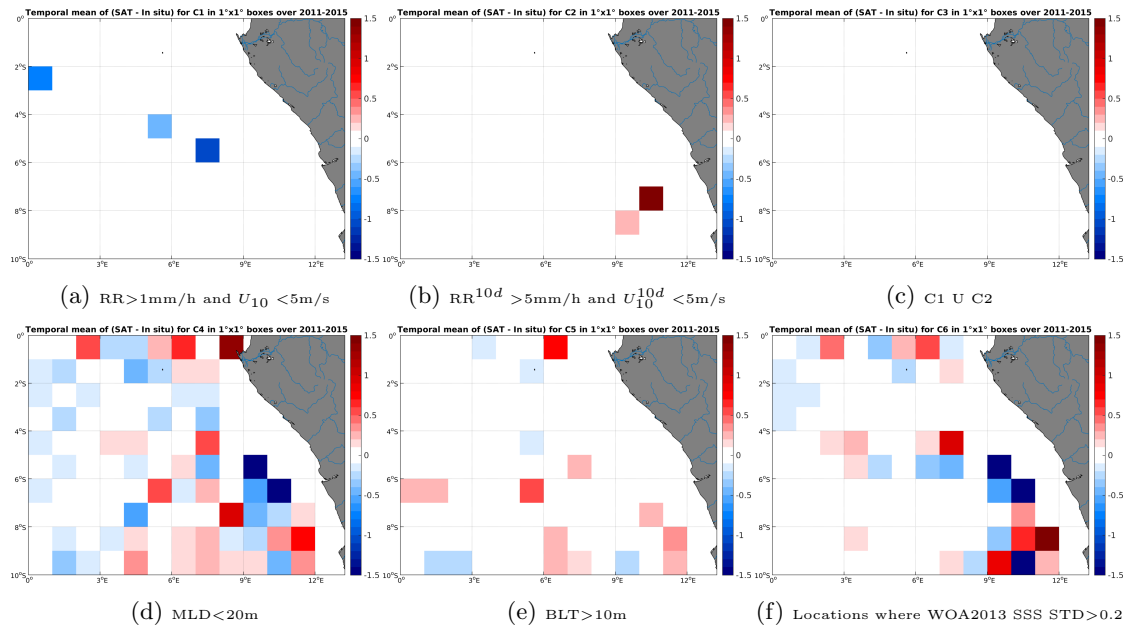
Figure 12: Temporal mean gridded over spatial boxes of size 1^\circ \times 1^\circ of \Delta SSS (Aquarius-L3-JPL-V4-7DAY-RUNNING - Argo) for 6 different subdatasets corresponding to:RR >1 mm/h and U_{10} < 5 m/s (a), RR^{10d} > 5 mm/h and U_{10}^{10d} < 5 m/s (b), C1 U C2 (c),MLD <20 m (d),BLT >10 m (e),Locations where WOA2013 SSS STD >0.2 (f).
