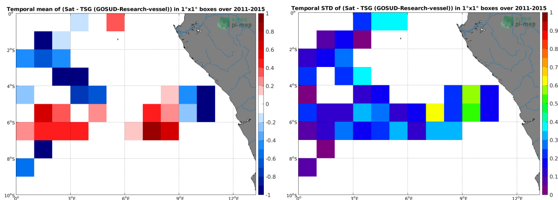
(e) MEAN( \Delta SSS) (Satellite - TSG (GOSUD-Research-vessel))
