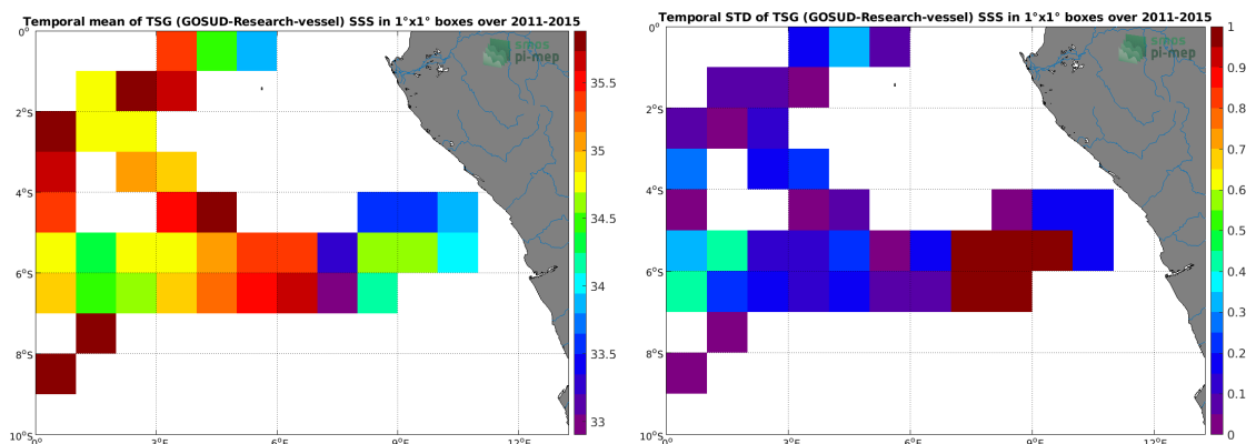
(c) MEAN(TSG (GOSUD-Research-vessel) SSS)
