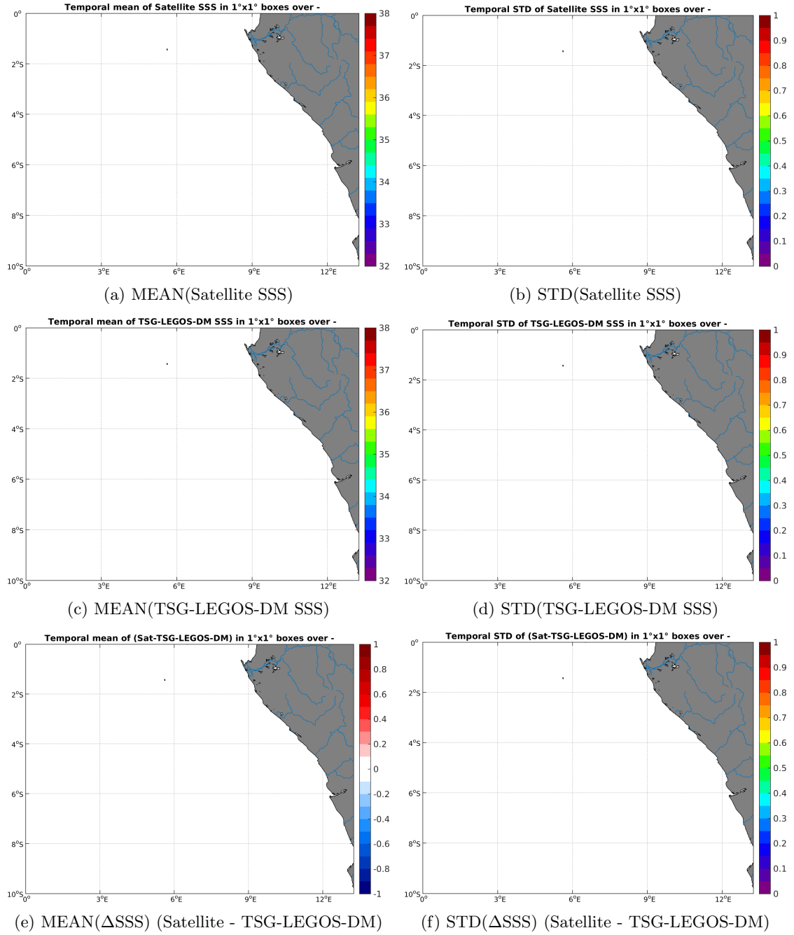
Figure 6: Temporal mean (left) and STD (right) of SSS from AQUARIUS-L2-JPL-V4 (top), TSG-LEGOS-DM (middle), and of \Delta SSS (Satellite - TSG-LEGOS-DM). Only match-up pairs are used to generate these maps.
