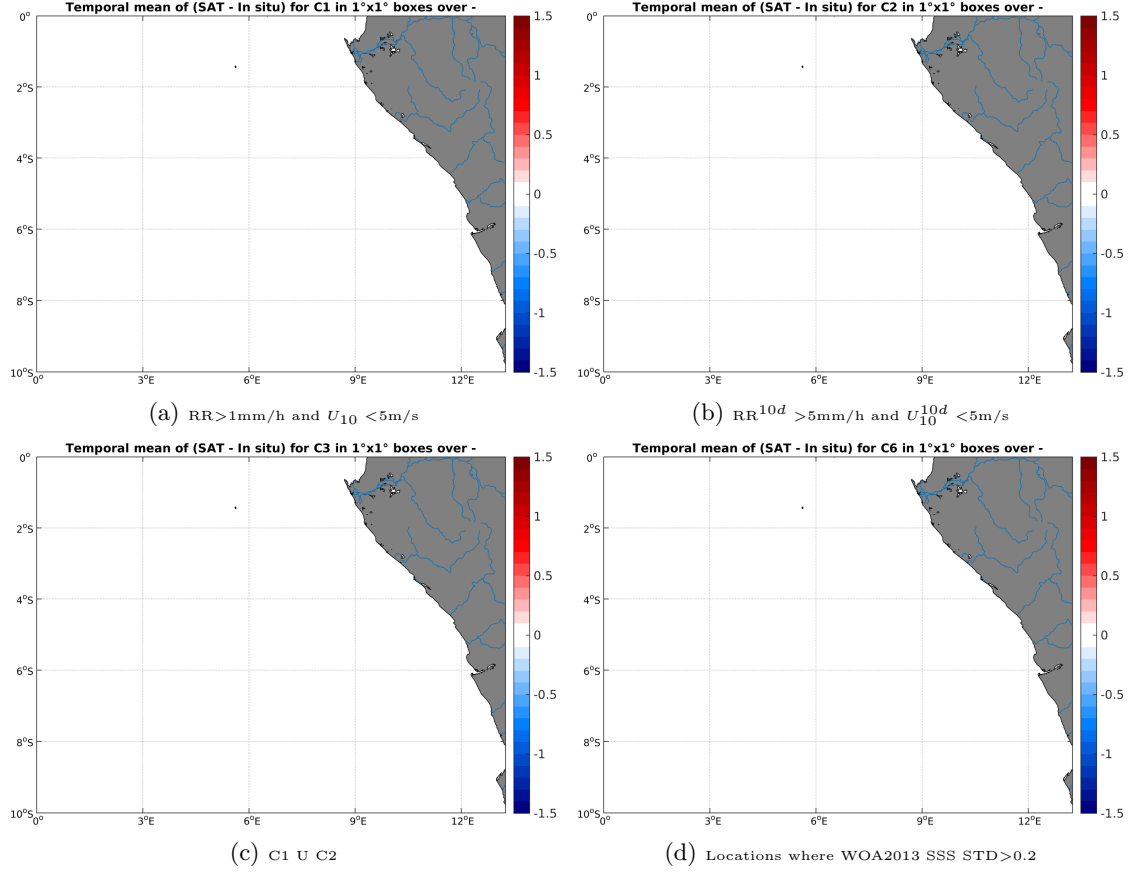
Figure 11: Temporal mean gridded over spatial boxes of size 1^\circ \times 1^\circ of \Delta SSS (AQUARIUS-L2-JPL-V4 - Surface drifters) for 4 different subdatasets corresponding to: RR > 1mm/h and U_{10} < 5 m/s (a), RR^{10d} > 5 mm/h and U_{10}^{10d} < 5 m/s (b), C1 U C2 (c), Locations where WOA2013 SSS STD > 0.2 (d).
