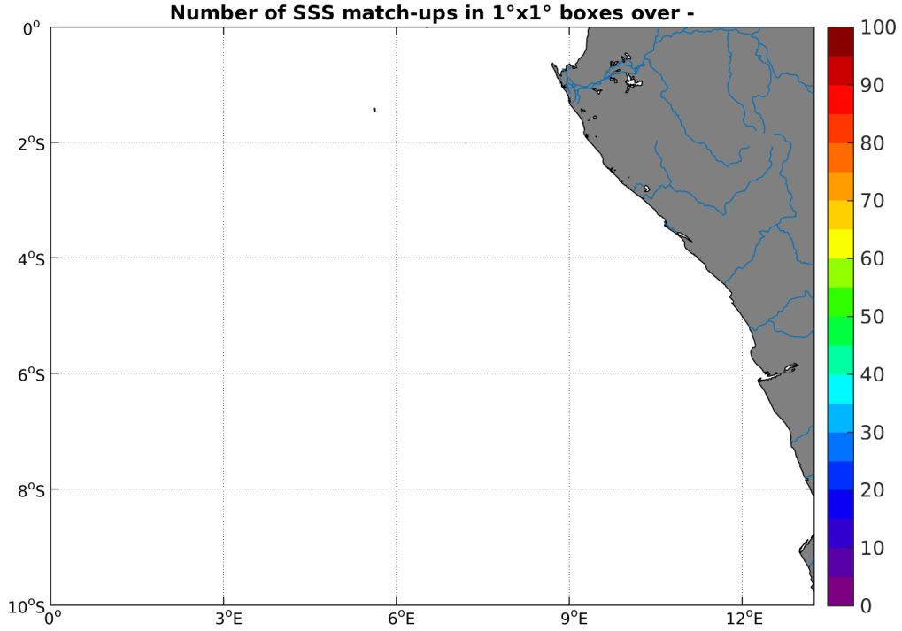
Figure 3: Number of SSS match-ups between Surface drifters SSS and the AQUARIUS-L2-JPL-V4 SSS product for the Congo river plume Pi-MEP region over 1^\circ \times 1^\circ boxes and for the full satellite product period.
