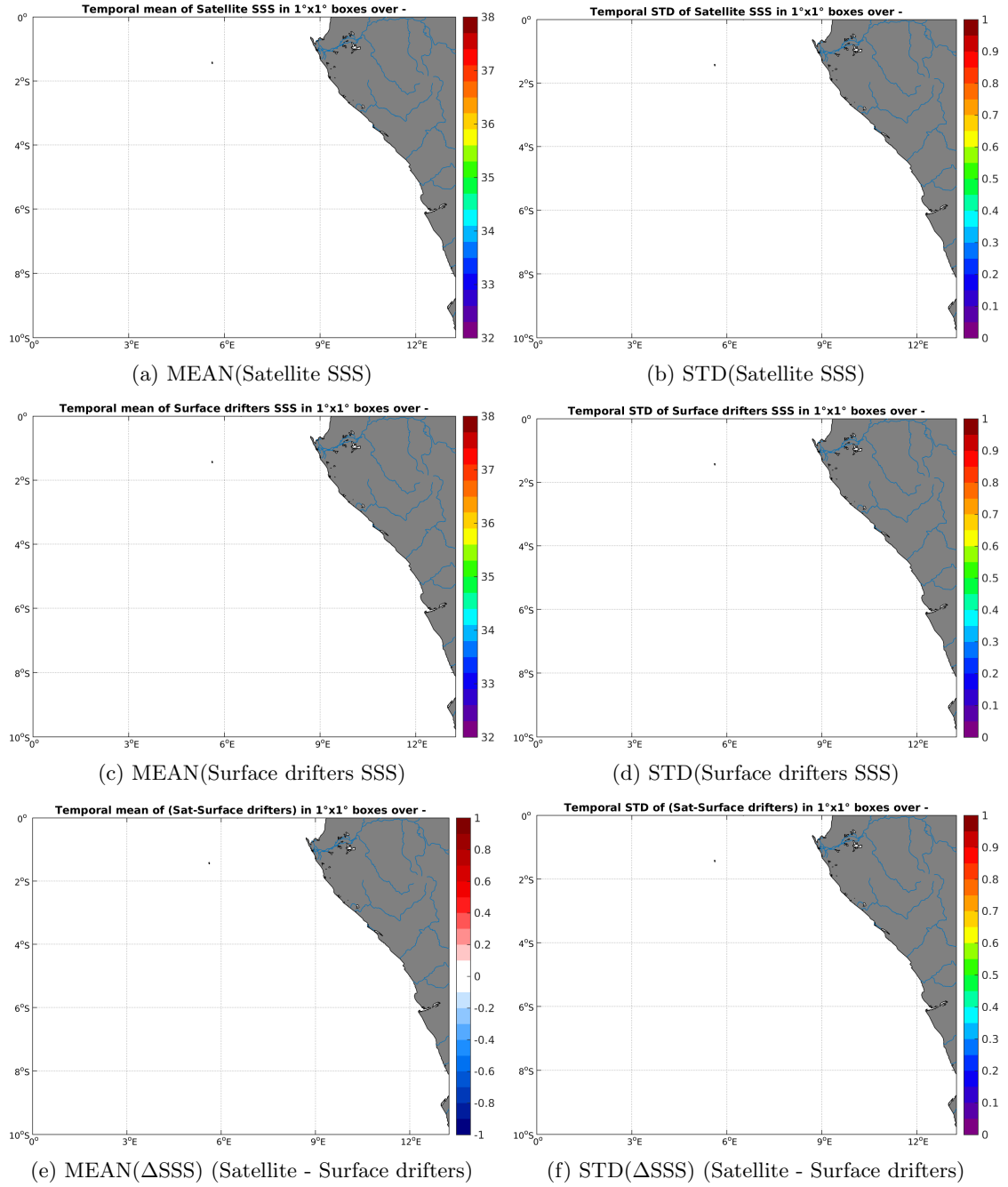
Figure 5: Temporal mean (left) and STD (right) of SSS from AQUARIUS-L2-JPL-V4 (top), Surface drifters (middle), and of \Delta SSS (Satellite - Surface drifters). Only match-up pairs are used to generate these maps.
