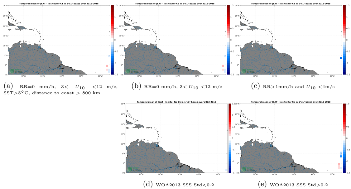
Figure 12: Temporal mean gridded over spatial boxes of size 1^\circ \times 1^\circ of \Delta SSS (SMOS and SMAP SSS L4 OI v1 - 7 Days (LOPS) - TSG (Polarstern)) for 5 different subdatasets corresponding to:RR=0 mm/h, 3 < U_{10} < 12 m/s, SST >5^\circ\text{C} , distance to coast > 800 km (a), RR=0 mm/h, 3 < U_{10} < 12 m/s (b), RR >1 mm/h and U_{10} < 4 m/s (c), WOA2013 SSS Std <0.2 (d), WOA2013 SSS Std >0.2 (e).
