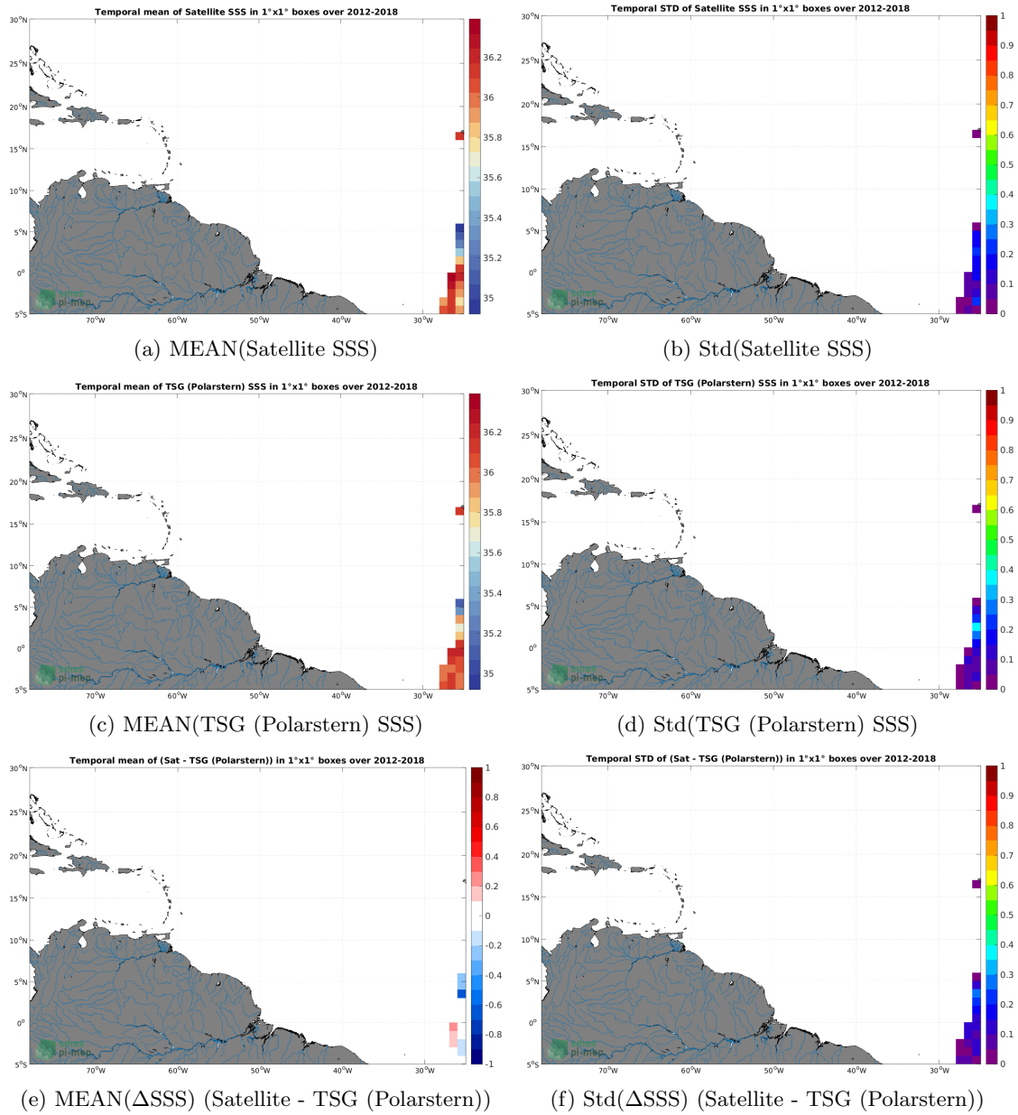
Figure 6: Temporal mean (left) and Std (right) of SSS from SMOS and SMAP SSS L4 OI v1 - 7 Days (LOPS) (top), TSG (Polarstern) (middle), and of \Delta SSS (Satellite - TSG (Polarstern)). Only match-up pairs are used to generate these maps.
