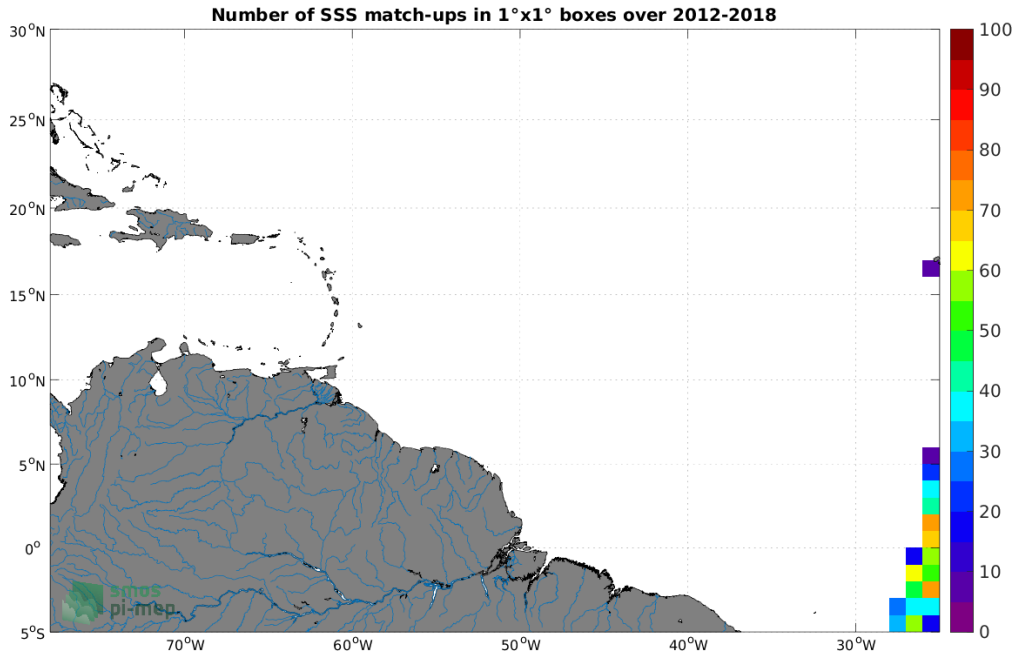
Figure 4: Number of SSS match-ups between TSG (Polarstern) SSS and the SMOS and SMAP SSS L4 OI v1 - 7 Days (LOPS) SSS product for the Amazon and Orinoco river plumes Pi-MEP region over 1^\circ \times 1^\circ boxes and for the full satellite product period.
