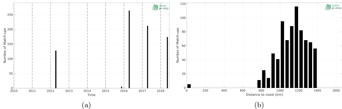
Figure 1: Number of match-ups between TSG (Polarstern) and SMOS and SMAP SSS L4 OI v1 - 7 Days (LOPS) SSS as a function of time (a) and as function of the distance to coast (b) over the Amazon and Orinoco river plumes Pi-MEP region and for the full satellite product period.
