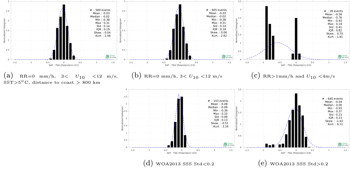
Figure 13: Normalized histogram of \Delta SSS (SMOS and SMAP SSS L4 OI v1 - 7 Days (LOPS) - TSG (Polarstern)) for 5 different subdatasets corresponding to: RR=0 mm/h, 3 < U_{10} < 12 m/s, SST > 5°C, distance to coast > 800 km (a), RR=0 mm/h, 3 < U_{10} < 12 m/s (b), RR > 1mm/h and U_{10} < 4 m/s (c), WOA2013 SSS Std < 0.2 (d), WOA2013 SSS Std > 0.2 (e).
