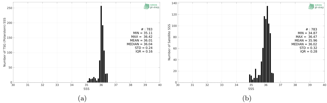
Figure 2: Histograms of SSS from TSG (Polarstern) (a) and SMOS and SMAP SSS L4 OI v1 - 7 Days (LOPS) (b) considering all match-up pairs per bins of 0.1 over the Amazon and Orinoco river plumes Pi-MEP region and for the full satellite product period.
