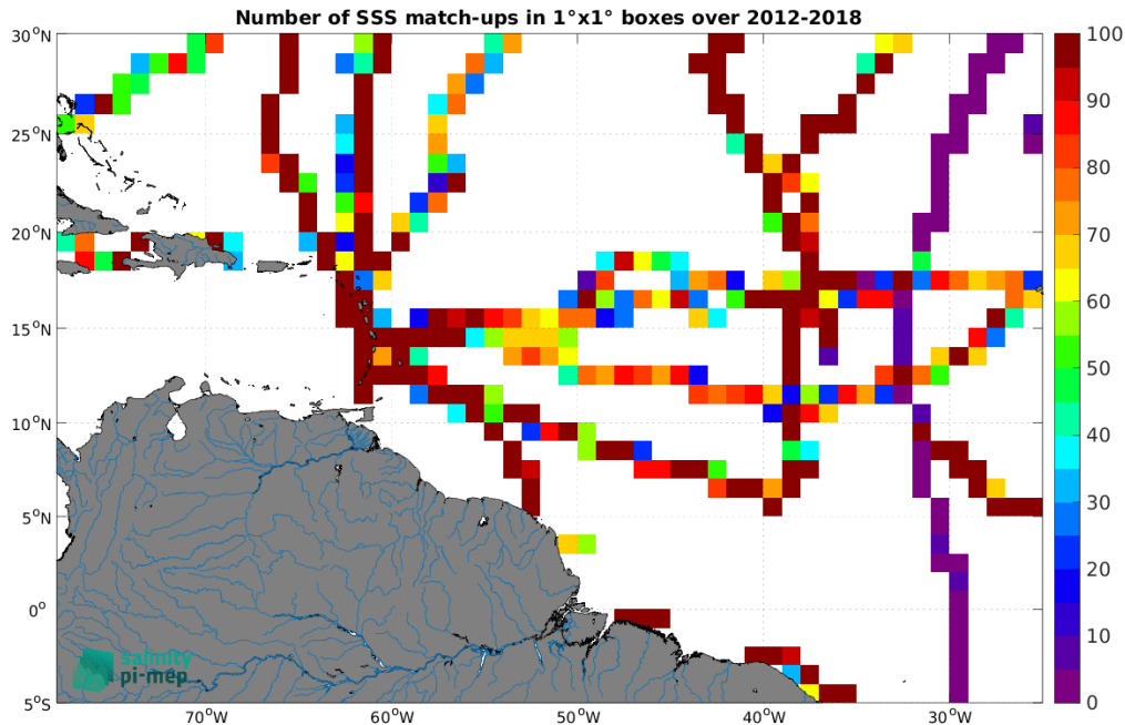
Figure 4: Number of SSS match-ups between TSG (GOSUD-Sailing-ship) SSS and the SMOS and SMAP SSS L4 OI v1 - 7 Days (LOPS) SSS product for the Amazon and Orinoco river plumes Pi-MEP region over 1^\circ \times 1^\circ boxes and for the full satellite product period.
