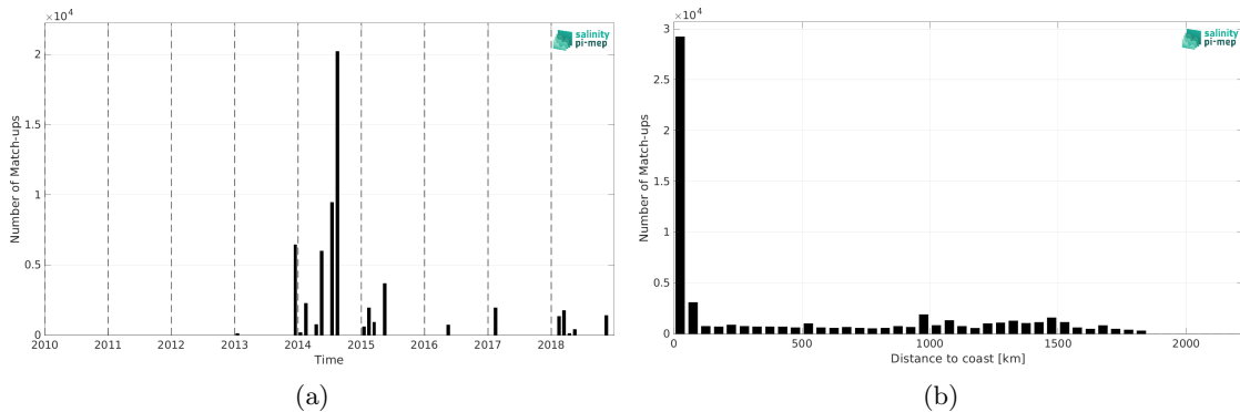
Figure 1: Number of match-ups between TSG (GOSUD-Sailing-ship) and SMOS and SMAP SSS L4 OI v1 - 7 Days (LOPS) SSS as a function of time (a) and as function of the distance to coast (b) over the Amazon and Orinoco river plumes Pi-MEP region and for the full satellite product period.
