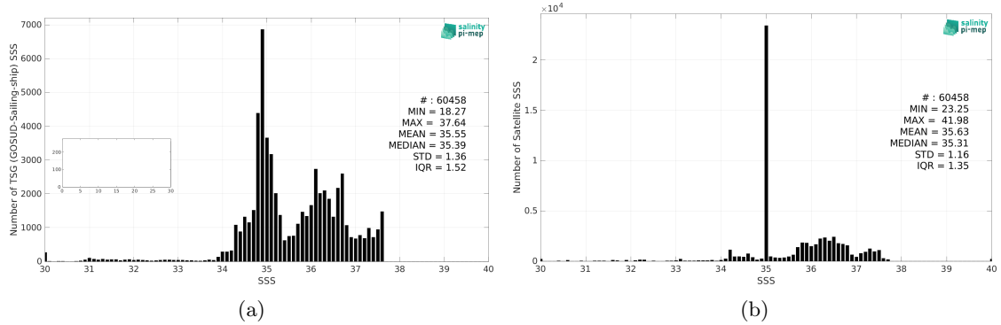
Figure 2: Histograms of SSS from TSG (GOSUD-Sailing-ship) (a) and SMOS and SMAP SSS L4 OI v1 - 7 Days (LOPS) (b) considering all match-up pairs per bins of 0.1 over the Amazon and Orinoco river plumes Pi-MEP region and for the full satellite product period.
