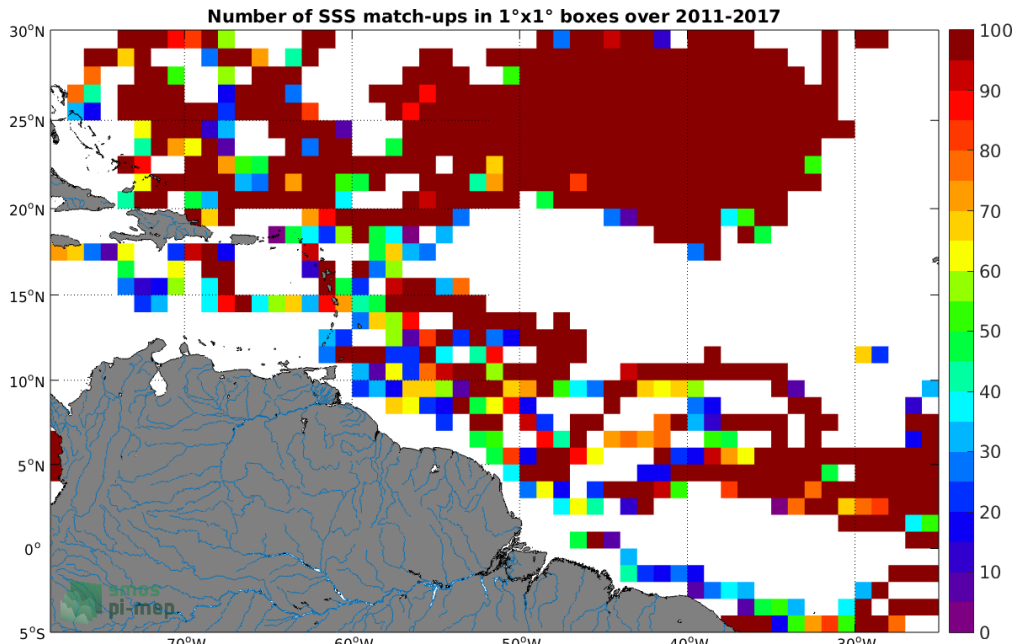
Figure 3: Number of SSS match-ups between Surface drifters SSS and the SMOS and SMAP SSS L4 OI v1 - 7 Days (LOPS) SSS product for the Amazon and Orinoco river plumes Pi-MEP region over 1^\circ \times 1^\circ boxes and for the full satellite product period.
