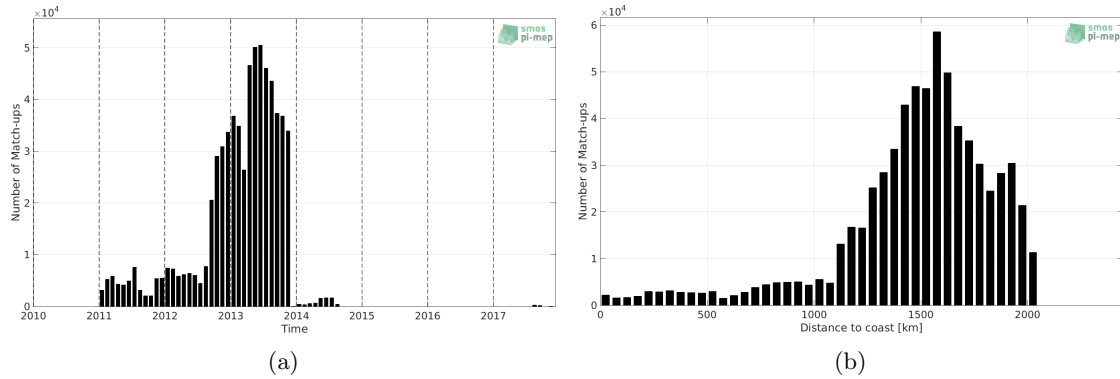
Figure 1: Number of match-ups between Surface drifters and SMOS and SMAP SSS L4 OI v1 - 7 Days (LOPS) SSS as a function of time (a) and as function of the distance to coast (b) over the Amazon and Orinoco river plumes Pi-MEP region and for the full satellite product period.
