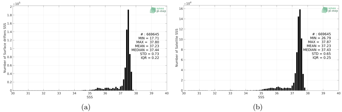
Figure 2: Histograms of SSS from Surface drifters (a) and SMOS and SMAP SSS L4 OI v1 - 7 Days (LOPS) (b) considering all match-up pairs per bins of 0.1 over the Amazon and Orinoco river plumes Pi-MEP region and for the full satellite product period.
