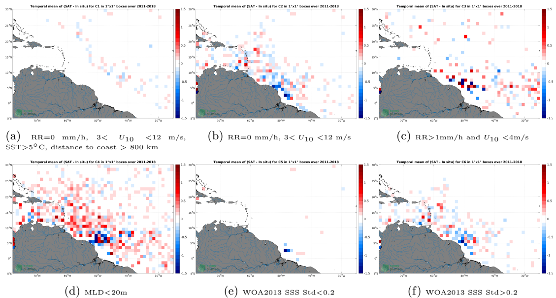
Figure 12: Temporal mean gridded over spatial boxes of size 1^\circ \times 1^\circ of \Delta SSS (SMOS and SMAP SSS L4 OI v1 - 7 Days (LOPS) - Argo) for 6 different subdatasets corresponding to: RR=0 mm/h, 3 < U_{10} < 12 m/s, SST >5^\circ C, distance to coast > 800 km (a), RR=0 mm/h, 3 < U_{10} < 12 m/s (b), RR >1 mm/h and U_{10} < 4 m/s (c),MLD <20 m (d),WOA2013 SSS Std <0.2 (e),WOA2013 SSS Std >0.2 (f).
