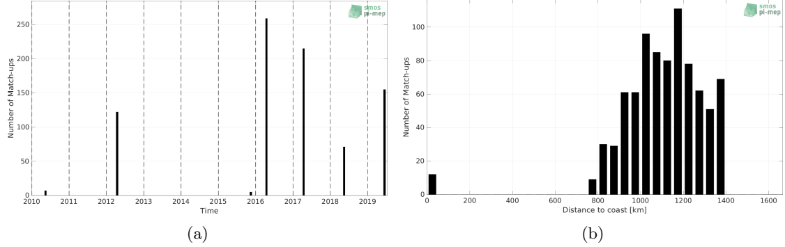
Figure 1: Number of match-ups between TSG (Polarstern) and SMOS SSS L4 v1 - Weekly (CMEMS-CNR) SSS as a function of time (a) and as function of the distance to coast (b) over the Amazon and Orinoco river plumes Pi-MEP region and for the full satellite product period.
