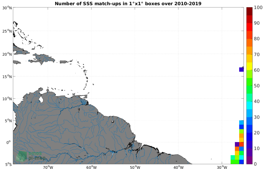
Figure 4: Number of SSS match-ups between TSG (Polarstern) SSS and the SMOS SSS L4 v1 - Weekly (CMEMS-CNR) SSS product for the Amazon and Orinoco river plumes Pi-MEP region over 1^\circ \times 1^\circ boxes and for the full satellite product period.
