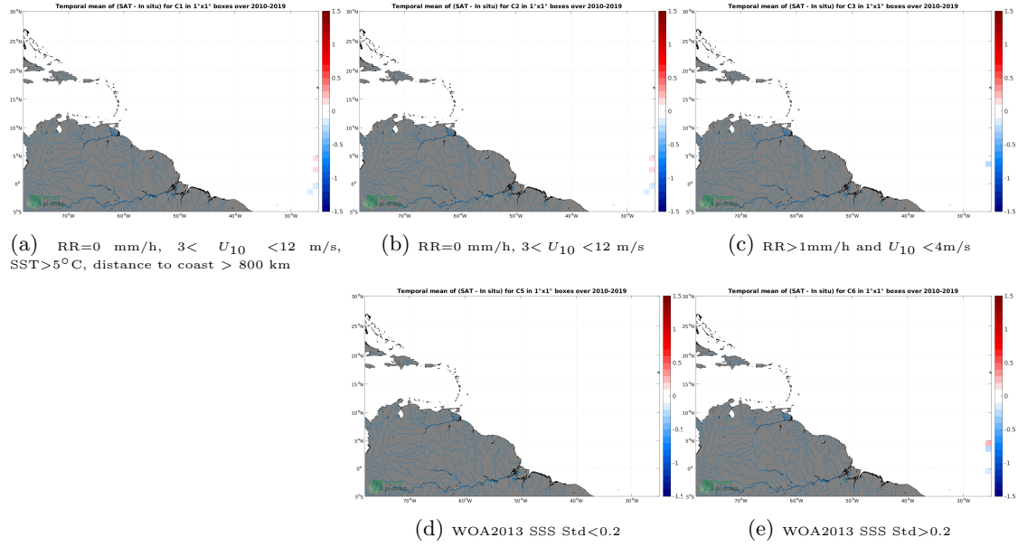
Figure 12: Temporal mean gridded over spatial boxes of size 1^\circ \times 1^\circ of \Delta SSS (SMOS SSS L4 v1 - Weekly (CMEMS-CNR) - TSG (Polarstern)) for 5 different subdatasets corresponding to: RR=0 mm/h, 3 < U_{10} < 12 m/s, SST > 5^\circ C , distance to coast > 800 km (a), RR=0 mm/h, 3 < U_{10} < 12 m/s (b), RR > 1 mm/h and U_{10} < 4 m/s (c), WOA2013 SSS Std < 0.2 (d), WOA2013 SSS Std > 0.2 (e).
