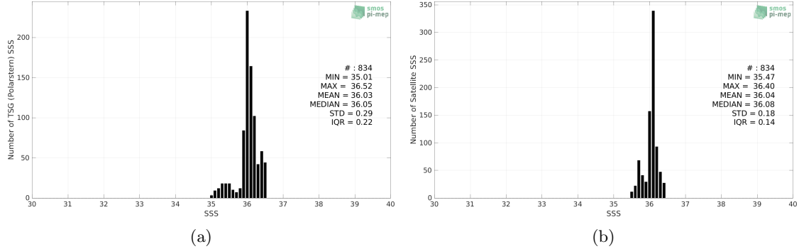
Figure 2: Histograms of SSS from TSG (Polarstern) (a) and SMOS SSS L4 v1 - Weekly (CMEMS-CNR) (b) considering all match-up pairs per bins of 0.1 over the Amazon and Orinoco river plumes Pi-MEP region and for the full satellite product period.
