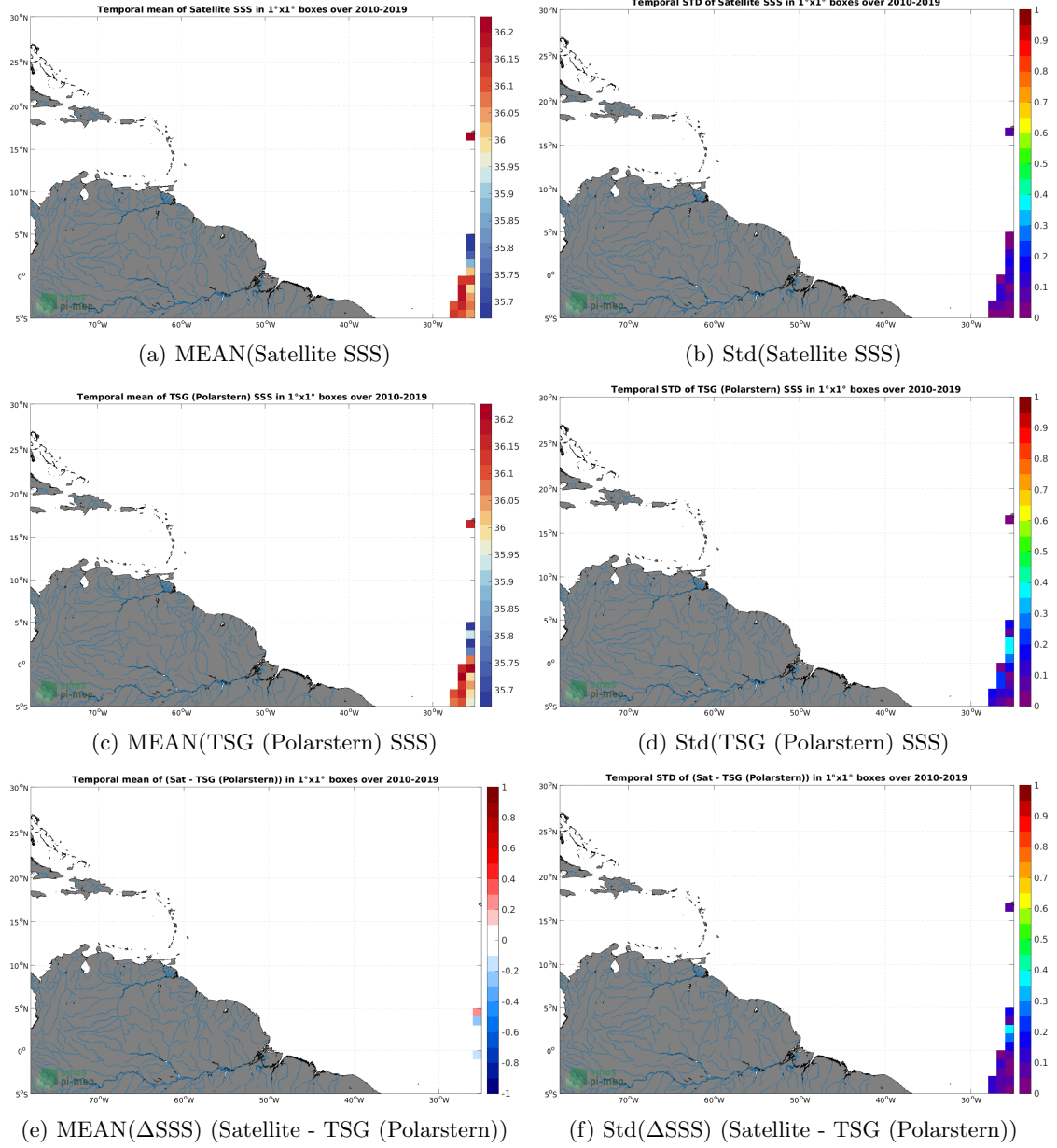
Figure 6: Temporal mean (left) and Std (right) of SSS from SMOS SSS L4 v1 - Weekly (CMEMS-CNR) (top), TSG (Polarstern) (middle), and of \Delta SSS (Satellite - TSG (Polarstern)). Only match-up pairs are used to generate these maps.
