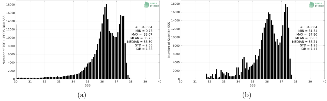
Figure 2: Histograms of SSS from TSG (LEGOS-DM) (a) and SMOS SSS L4 v1 - Weekly (CMEMS-CNR) (b) considering all match-up pairs per bins of 0.1 over the Amazon and Orinoco river plumes Pi-MEP region and for the full satellite product period.
