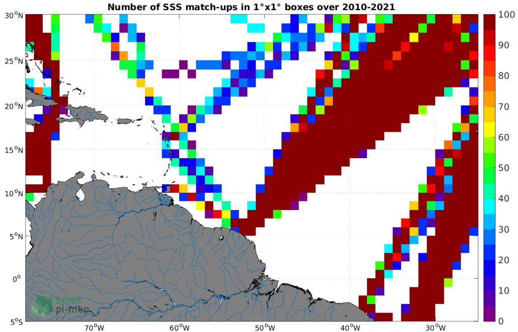
Figure 4: Number of SSS match-ups between TSG (LEGOS-DM) SSS and the SMOS SSS L4 v1 - Weekly (CMEMS-CNR) SSS product for the Amazon and Orinoco river plumes Pi-MEP region over 1^\circ \times 1^\circ boxes and for the full satellite product period.
