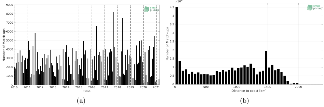
Figure 1: Number of match-ups between TSG (LEGOS-DM) and SMOS SSS L4 v1 - Weekly (CMEMS-CNR) SSS as a function of time (a) and as function of the distance to coast (b) over the Amazon and Orinoco river plumes Pi-MEP region and for the full satellite product period.
