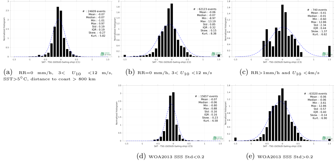
Figure 13: Normalized histogram of \Delta SSS (SMOS SSS L4 v1 - Weekly (CMEMS-CNR) - TSG (GOSUD-Sailing-ship)) for 5 different subdatasets corresponding to: RR=0 mm/h, 3 < U_{10} < 12 m/s, SST > 5^\circ C , distance to coast > 800 km (a), RR=0 mm/h, 3 < U_{10} < 12 m/s (b), RR > 1 mm/h and U_{10} < 4 m/s (c), WOA2013 SSS Std < 0.2 (d), WOA2013 SSS Std > 0.2 (e).
