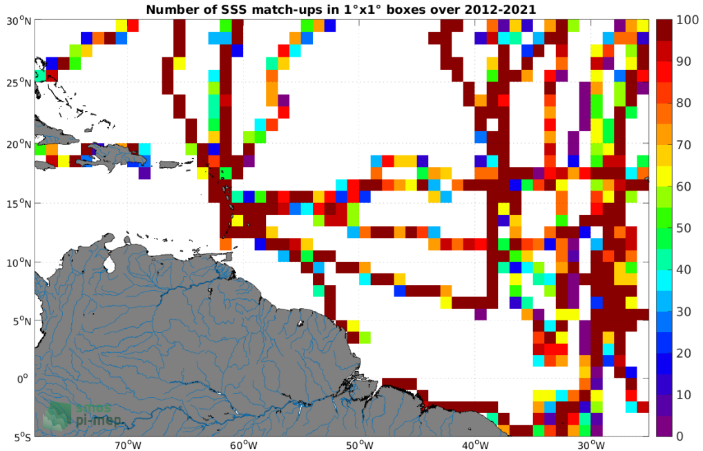
Figure 4: Number of SSS match-ups between TSG (GOSUD-Sailing-ship) SSS and the SMOS SSS L4 v1 - Weekly (CMEMS-CNR) SSS product for the Amazon and Orinoco river plumes Pi-MEP region over 1^\circ \times 1^\circ boxes and for the full satellite product period.
