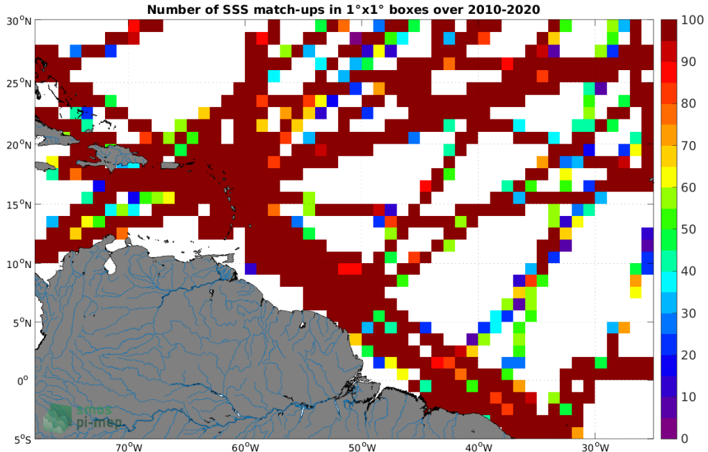
Figure 4: Number of SSS match-ups between TSG (GOSUD-Research-vessel) SSS and the SMOS SSS L4 v1 - Weekly (CMEMS-CNR) SSS product for the Amazon and Orinoco river plumes Pi-MEP region over 1^\circ \times 1^\circ boxes and for the full satellite product period.
