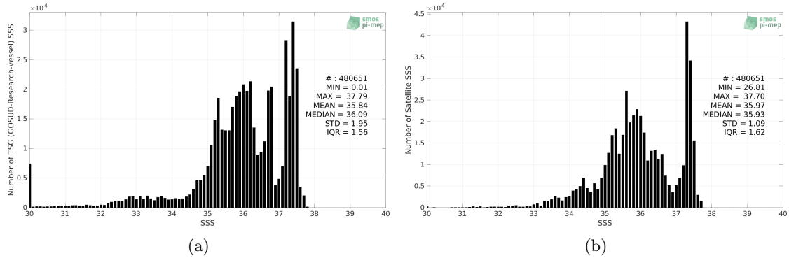
Figure 2: Histograms of SSS from TSG (GOSUD-Research-vessel) (a) and SMOS SSS L4 v1 - Weekly (CMEMS-CNR) (b) considering all match-up pairs per bins of 0.1 over the Amazon and Orinoco river plumes Pi-MEP region and for the full satellite product period.
