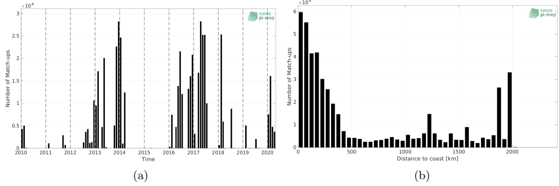
Figure 1: Number of match-ups between TSG (GOSUD-Research-vessel) and SMOS SSS L4 v1 - Weekly (CMEMS-CNR) SSS as a function of time (a) and as function of the distance to coast (b) over the Amazon and Orinoco river plumes Pi-MEP region and for the full satellite product period.
