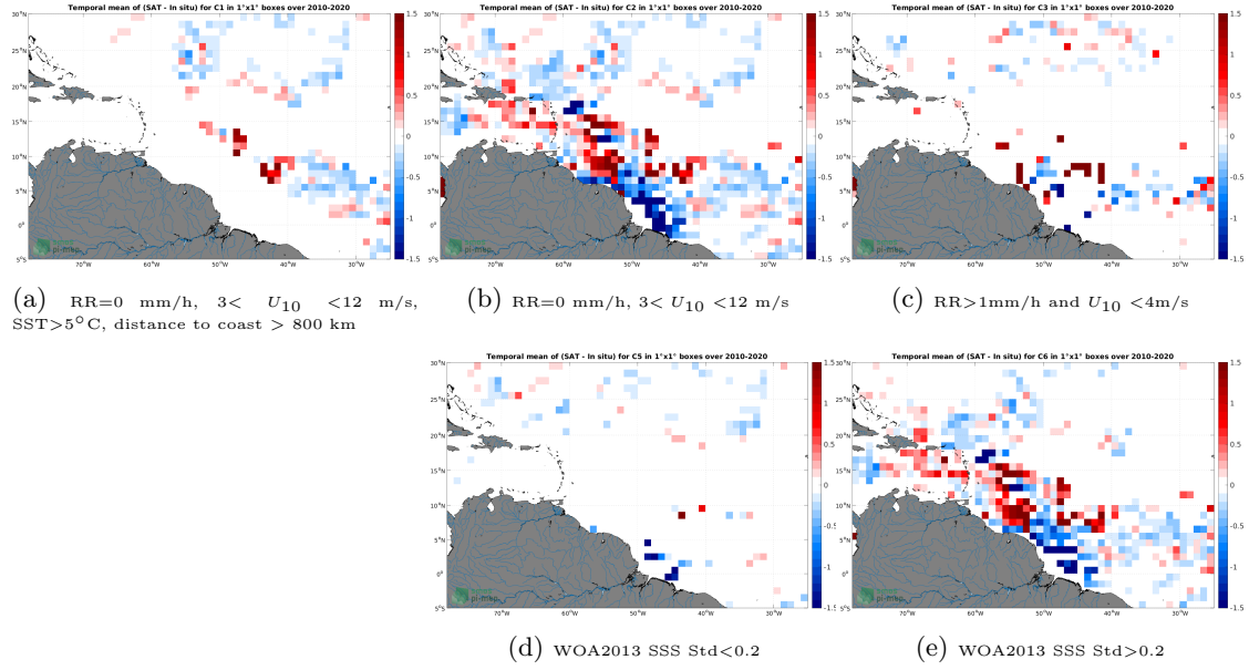
Figure 11: Temporal mean gridded over spatial boxes of size 1^\circ \times 1^\circ of \Delta SSS (SMOS SSS L4 v1 - Weekly (CMEMS-CNR) - Surface drifters) for 5 different subdatasets corresponding to: RR=0 mm/h, 3 < U_{10} < 12 m/s, SST > 5^\circ C , distance to coast > 800 km (a), RR=0 mm/h, 3 < U_{10} < 12 m/s (b), RR > 1 mm/h and U_{10} < 4 m/s (c), WOA2013 SSS Std < 0.2 (d), WOA2013 SSS Std > 0.2 (e).
