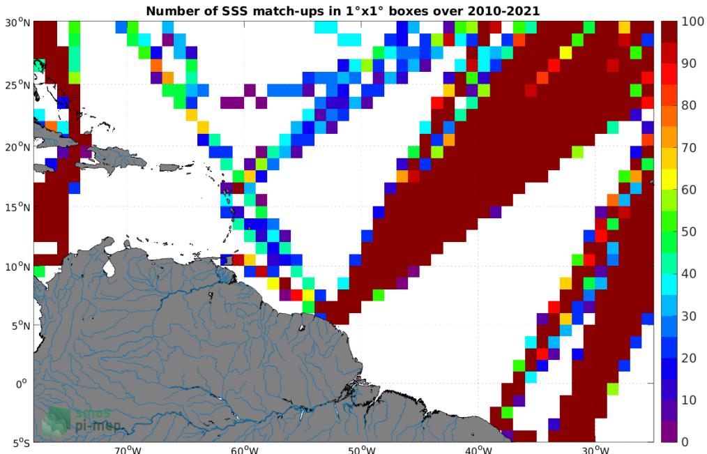
Figure 4: Number of SSS match-ups between TSG (LEGOS-DM) SSS and the SMOS SSS L4 v1 - Monthly (CMEMS-CNR) SSS product for the Amazon and Orinoco river plumes Pi-MEP region over 1^\circ \times 1^\circ boxes and for the full satellite product period.
