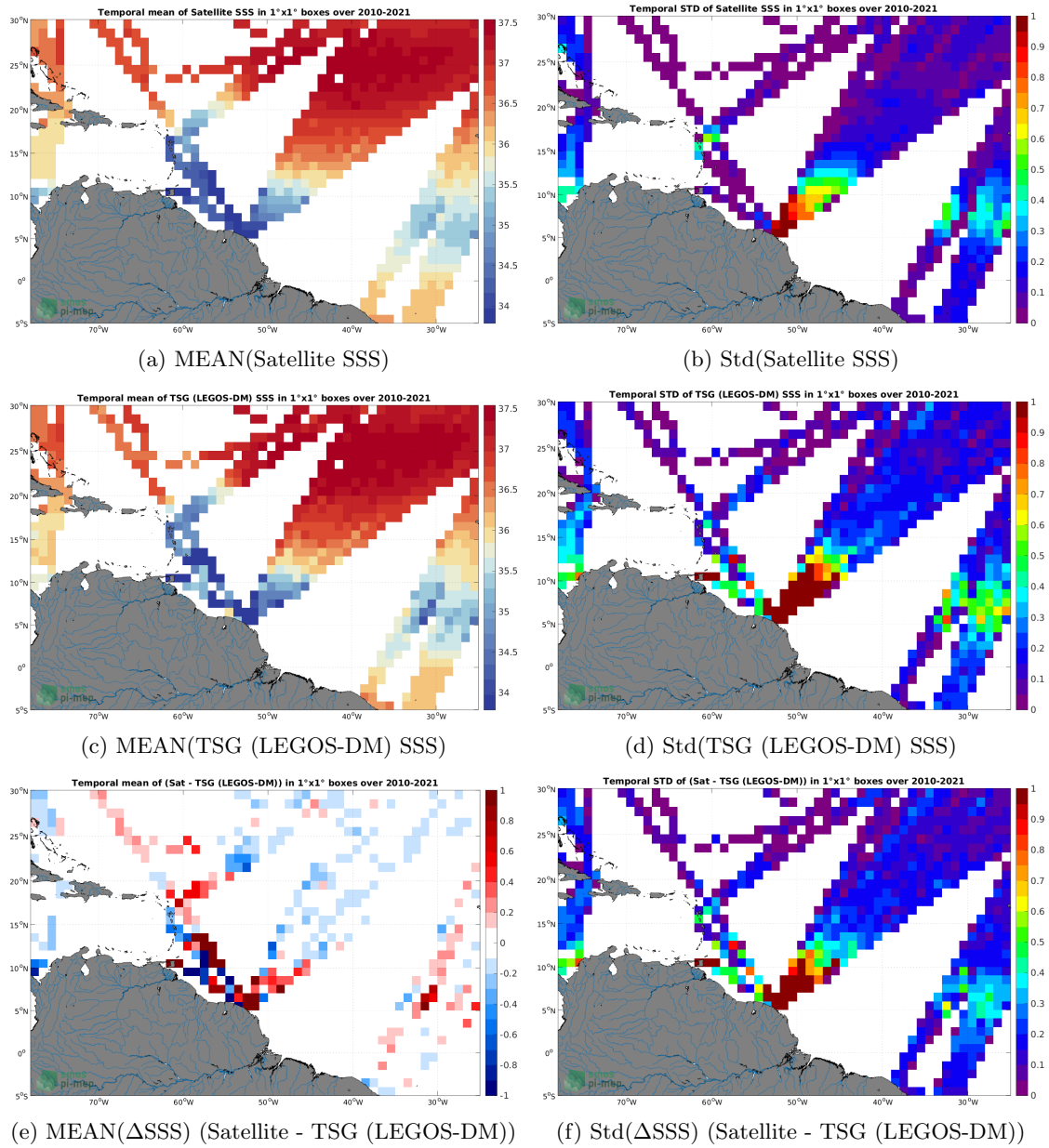
Figure 6: Temporal mean (left) and Std (right) of SSS from SMOS SSS L4 v1 - Monthly (CMEMS-CNR) (top), TSG (LEGOS-DM) (middle), and of \Delta SSS (Satellite - TSG (LEGOS-DM)). Only match-up pairs are used to generate these maps.
