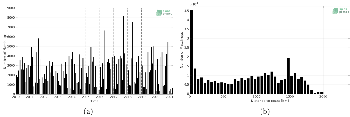
Figure 1: Number of match-ups between TSG (LEGOS-DM) and SMOS SSS L4 v1 - Monthly (CMEMS-CNR) SSS as a function of time (a) and as function of the distance to coast (b) over the Amazon and Orinoco river plumes Pi-MEP region and for the full satellite product period.
