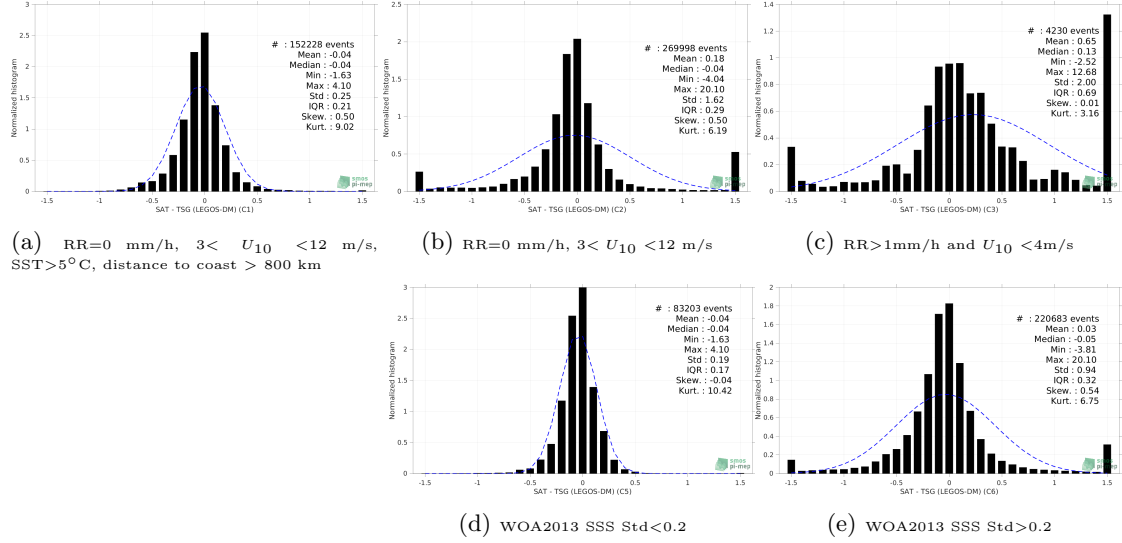
Figure 13: Normalized histogram of \Delta SSS (SMOS SSS L4 v1 - Monthly (CMEMS-CNR) - TSG (LEGOS-DM)) for 5 different subdatasets corresponding to: RR=0 mm/h, 3 < U_{10} < 12 m/s, SST > 5°C, distance to coast > 800 km (a), RR=0 mm/h, 3 < U_{10} < 12 m/s (b), RR > 1mm/h and U_{10} < 4 m/s (c), WOA2013 SSS Std < 0.2 (d), WOA2013 SSS Std > 0.2 (e).
