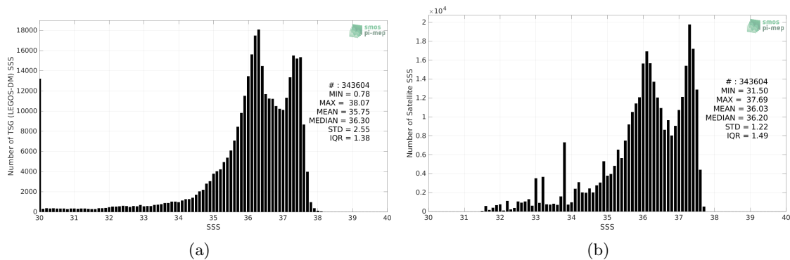
Figure 2: Histograms of SSS from TSG (LEGOS-DM) (a) and SMOS SSS L4 v1 - Monthly (CMEMS-CNR) (b) considering all match-up pairs per bins of 0.1 over the Amazon and Orinoco river plumes Pi-MEP region and for the full satellite product period.
