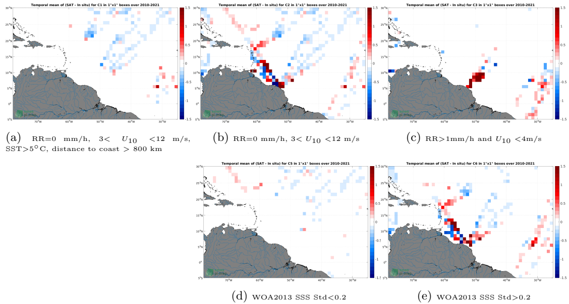
Figure 12: Temporal mean gridded over spatial boxes of size 1^\circ \times 1^\circ of \Delta SSS (SMOS SSS L4 v1 - Monthly (CMEMS-CNR) - TSG (LEGOS-DM)) for 5 different subdatasets corresponding to:RR=0 mm/h, 3 < U_{10} < 12 m/s, SST >5^\circ\text{C} , distance to coast > 800 km (a), RR=0 mm/h, 3 < U_{10} < 12 m/s (b), RR >1 mm/h and U_{10} < 4 m/s (c), WOA2013 SSS Std <0.2 (d), WOA2013 SSS Std >0.2 (e).
