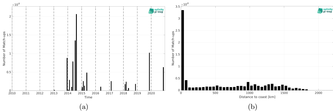
Figure 1: Number of match-ups between TSG (GOSUD-Sailing-ship) and SMOS SSS L4 v1 - Monthly (CMEMS-CNR) SSS as a function of time (a) and as function of the distance to coast (b) over the Amazon and Orinoco river plumes Pi-MEP region and for the full satellite product period.
