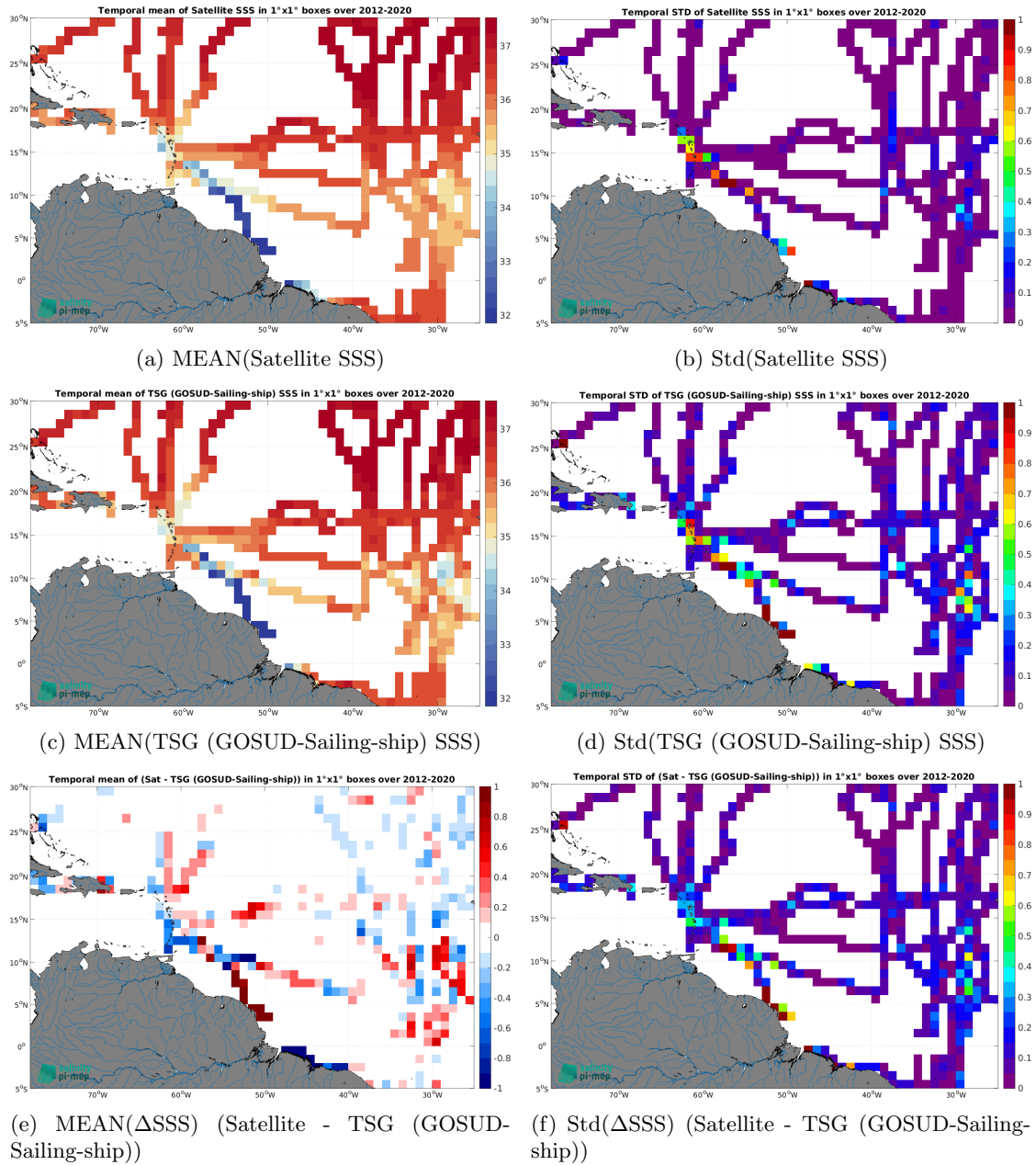
Figure 6: Temporal mean (left) and Std (right) of SSS from SMOS SSS L4 v1 - Monthly (CMEMS-CNR) (top), TSG (GOSUD-Sailing-ship) (middle), and of \Delta SSS (Satellite - TSG (GOSUD-Sailing-ship)). Only match-up pairs are used to generate these maps.
