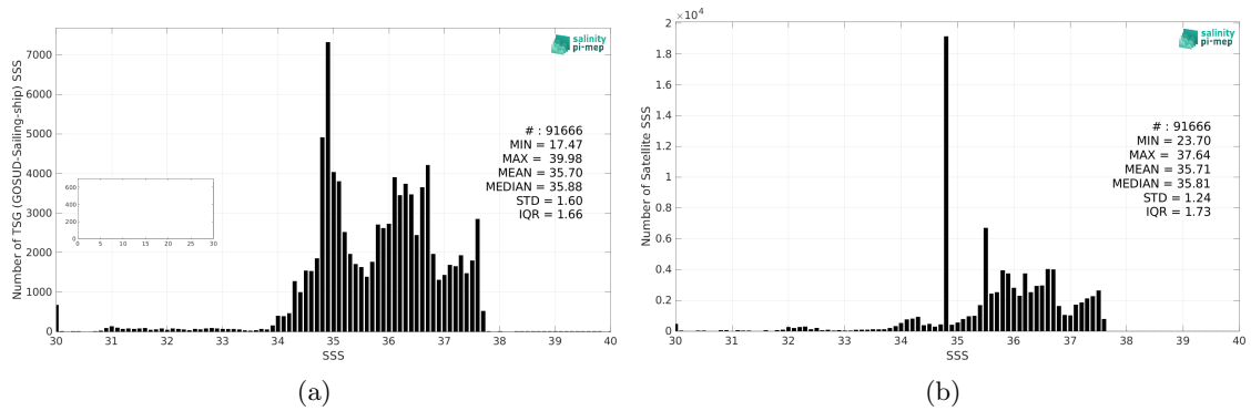
Figure 2: Histograms of SSS from TSG (GOSUD-Sailing-ship) (a) and SMOS SSS L4 v1 - Monthly (CMEMS-CNR) (b) considering all match-up pairs per bins of 0.1 over the Amazon and Orinoco river plumes Pi-MEP region and for the full satellite product period.
