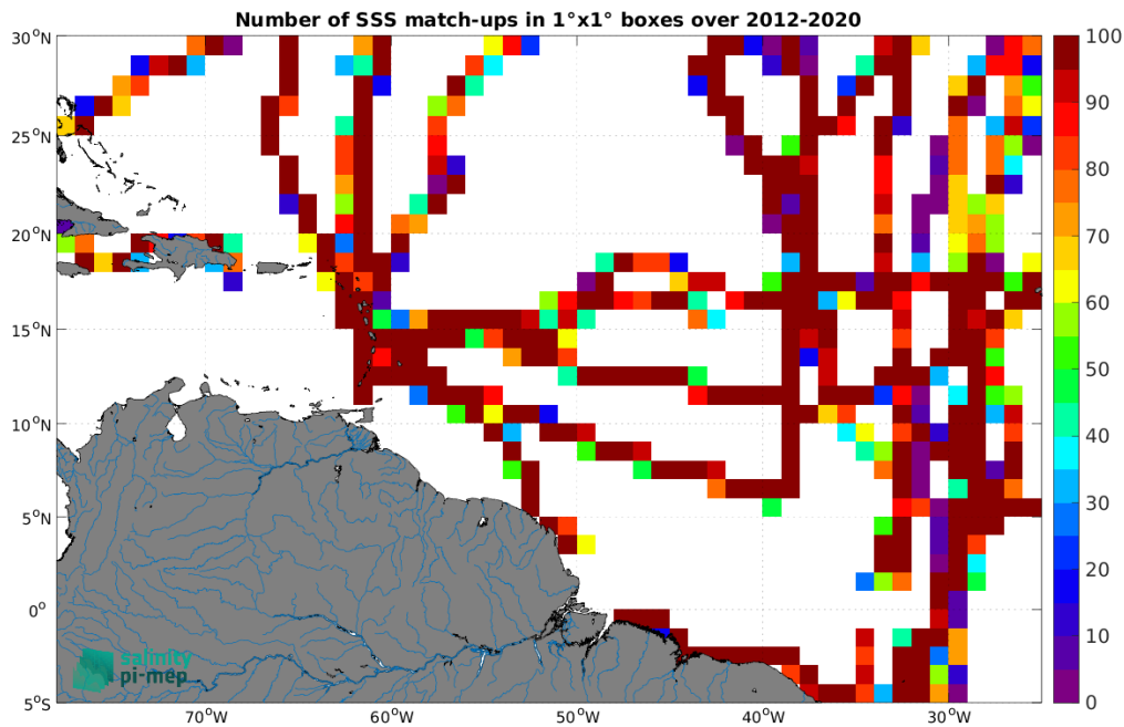
Figure 4: Number of SSS match-ups between TSG (GOSUD-Sailing-ship) SSS and the SMOS SSS L4 v1 - Monthly (CMEMS-CNR) SSS product for the Amazon and Orinoco river plumes Pi-MEP region over 1^\circ \times 1^\circ boxes and for the full satellite product period.
