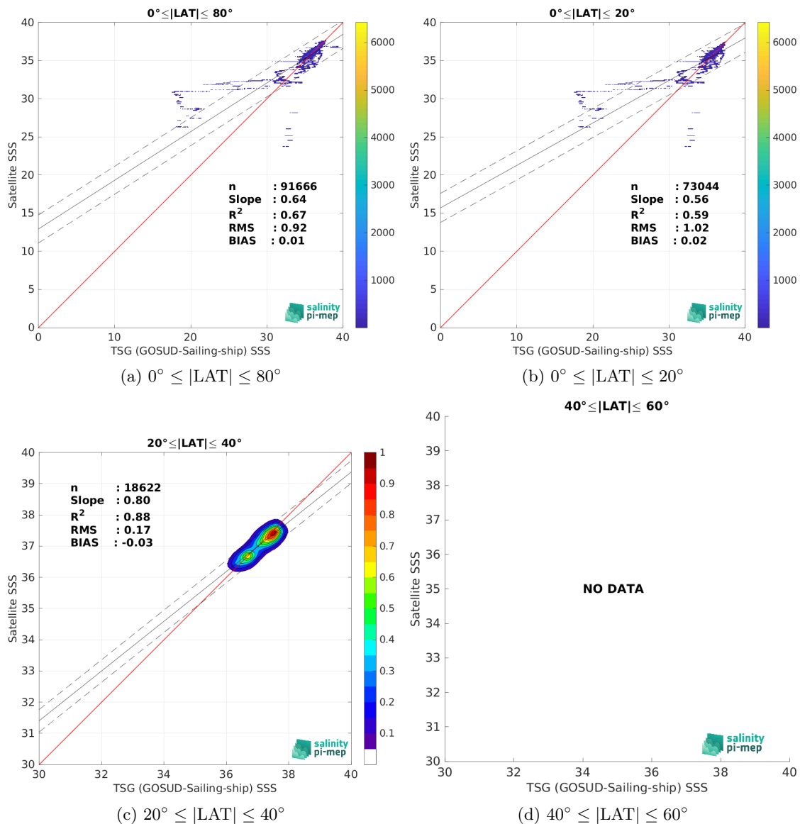
Figure 9: Contour maps of the concentration of SMOS SSS L4 v1 - Monthly (CMEMS-CNR) SSS (y-axis) versus TSG (GOSUD-Sailing-ship) SSS (x-axis) at match-up pairs for different latitude bands. For each plot, the red line shows x=y . The black thin and dashed lines indicate a linear fit through the data cloud and the \pm 95\% confidence levels, respectively. The number match-up pairs n , the slope and R^2 coefficient of the linear fit, the root mean square (RMS) and the mean bias between satellite and in situ data are indicated for each latitude band in each plots.
