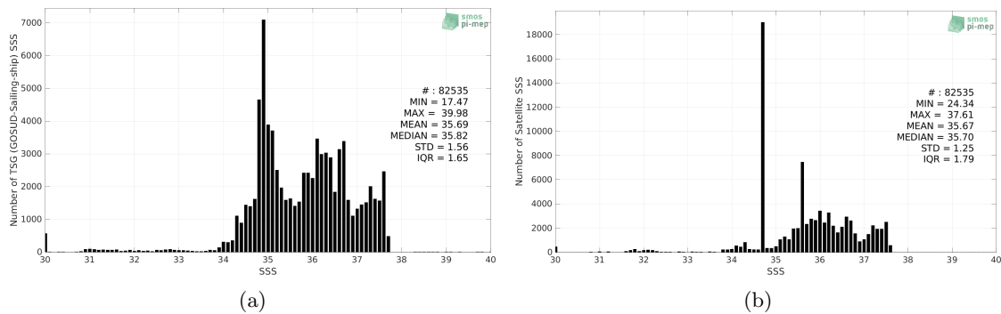
Figure 2: Histograms of SSS from TSG (GOSUD-Sailing-ship) (a) and SMOS SSS L4 v1 - Monthly (CMEMS-CNR) (b) considering all match-up pairs per bins of 0.1 over the Amazon and Orinoco river plumes Pi-MEP region and for the full satellite product period.
