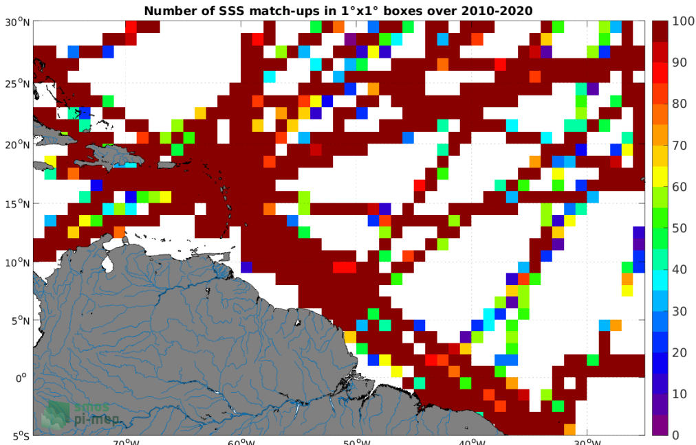
Figure 4: Number of SSS match-ups between TSG (GOSUD-Research-vessel) SSS and the SMOS SSS L4 v1 - Monthly (CMEMS-CNR) SSS product for the Amazon and Orinoco river plumes Pi-MEP region over 1°x1° boxes and for the full satellite product period.
