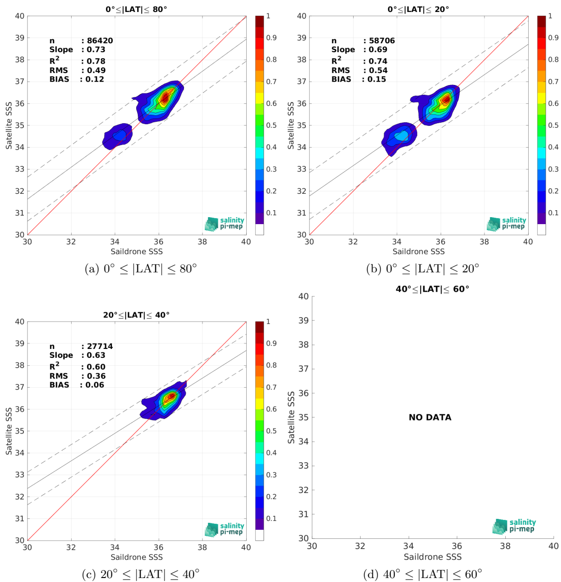
Figure 10: Contour maps of the concentration of SMOS SSS L4 v1 - Monthly (CMEMS-CNR) SSS (y-axis) versus Saildrone SSS (x-axis) at match-up pairs for different latitude bands. For each plot, the red line shows x=y . The black thin and dashed lines indicate a linear fit through the data cloud and the \pm 95\% confidence levels, respectively. The number match-up pairs n , the slope and R^2 coefficient of the linear fit, the root mean square (RMS) and the mean bias between satellite and in situ data are indicated for each latitude band in each plots.
