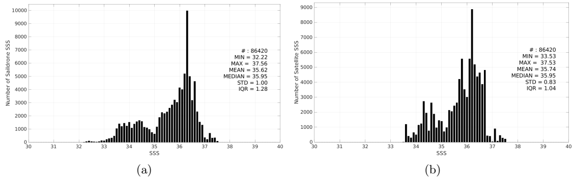
Figure 3: Histograms of SSS from Saildrone (a) and SMOS SSS L4 v1 - Monthly (CMEMS-CNR) (b) considering all match-up pairs per bins of 0.1 over the Amazon and Orinoco river plumes Pi-MEP region and for the full satellite product period.
