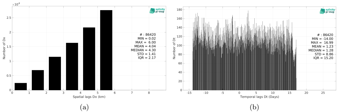
Figure 6: Histograms of the spatial (a) and temporal (b) lags between the location/time of the Saildrone measurement and the date of the corresponding SMOS SSS L4 v1 - Monthly (CMEMS-CNR) SSS pixel.
