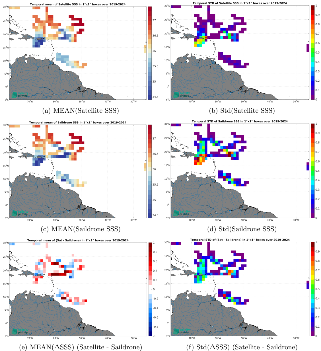
Figure 7: Temporal mean (left) and Std (right) of SSS from SMOS SSS L4 v1 - Monthly (CMEMS-CNR) (top), Saildrone (middle), and of \Delta SSS (Satellite - Saildrone). Only match-up pairs are used to generate these maps.
