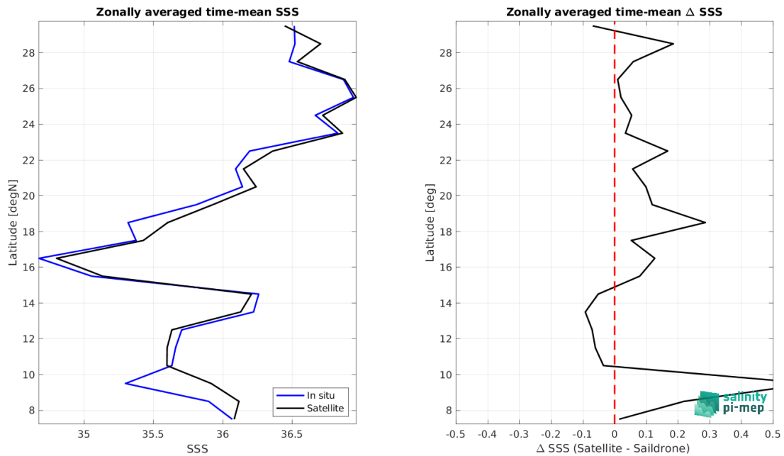
Figure 9: Left panel: Zonal mean SSS from SMOS SSS L4 v1 - Monthly (CMEMS-CNR) satellite product (black) and from Sairdron (blue). Right panel: Zonal mean of \Delta SSS (Satellite - Sairdron) for all the collected Pi-MEP match-up pairs estimated over the full satellite product period.
