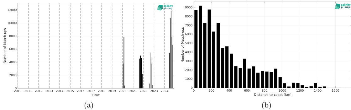
Figure 2: Number of match-ups between Saildrone and SMOS SSS L4 v1 - Monthly (CMEMS-CNR) SSS as a function of time (a) and as function of the distance to coast (b) over the Amazon and Orinoco river plumes Pi-MEP region and for the full satellite product period.
