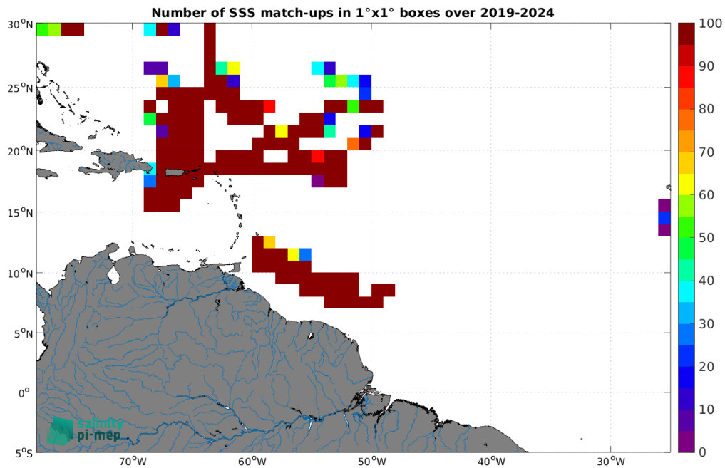
Figure 5: Number of SSS match-ups between Saildrone SSS and the SMOS SSS L4 v1 - Monthly (CMEMS-CNR) SSS product for the Amazon and Orinoco river plumes Pi-MEP region over 1^\circ \times 1^\circ boxes and for the full satellite product period.
