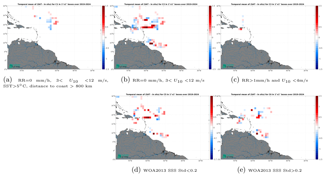
Figure 14: Temporal mean gridded over spatial boxes of size 1^\circ \times 1^\circ of \Delta SSS (SMOS SSS L4 v1 - Monthly (CMEMS-CNR) - Saildrone) for 5 different subdatasets corresponding to:RR=0 mm/h, 3 < U_{10} < 12 m/s, SST >5^\circ\text{C} , distance to coast > 800 km (a), RR=0 mm/h, 3 < U_{10} < 12 m/s (b), RR >1 mm/h and U_{10} < 4 m/s (c), WOA2013 SSS Std <0.2 (d), WOA2013 SSS Std >0.2 (e).
