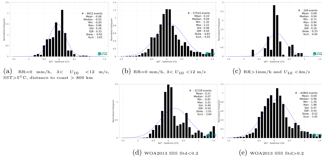
Figure 15: Normalized histogram of \Delta SSS (SMOS SSS L4 v1 - Monthly (CMEMS-CNR) - Saildrone) for 5 different subdatasets corresponding to: RR=0 mm/h, 3 < U_{10} < 12 m/s, SST>5°C, distance to coast > 800 km (a), RR=0 mm/h, 3 < U_{10} < 12 m/s (b), RR>1mm/h and U_{10} < 4 m/s (c), WOA2013 SSS Std<0.2 (d), WOA2013 SSS Std>0.2 (e).
