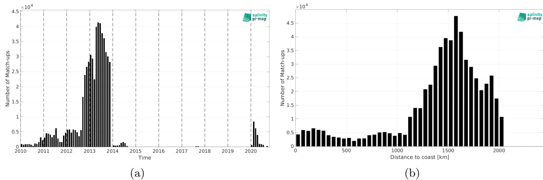
Figure 2: Number of match-ups between Surface drifters and SMOS SSS L4 v1 - Monthly (CMEMS-CNR) SSS as a function of time (a) and as function of the distance to coast (b) over the Amazon and Orinoco river plumes Pi-MEP region and for the full satellite product period.
