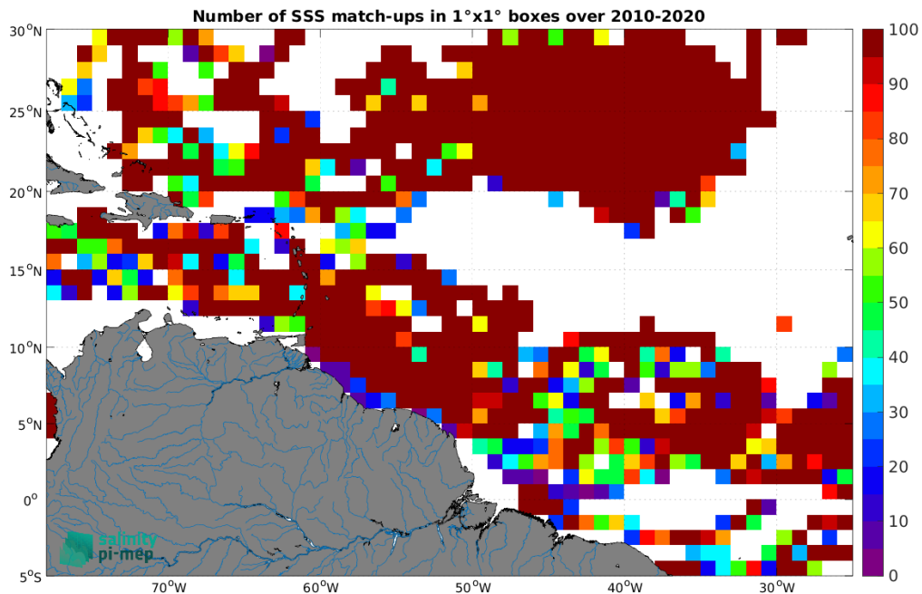
Figure 4: Number of SSS match-ups between Surface drifters SSS and the SMOS SSS L4 v1 - Monthly (CMEMS-CNR) SSS product for the Amazon and Orinoco river plumes Pi-MEP region over 1^\circ \times 1^\circ boxes and for the full satellite product period.
