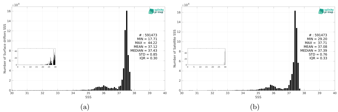
Figure 3: Histograms of SSS from Surface drifters (a) and SMOS SSS L4 v1 - Monthly (CMEMS-CNR) (b) considering all match-up pairs per bins of 0.1 over the Amazon and Orinoco river plumes Pi-MEP region and for the full satellite product period.
