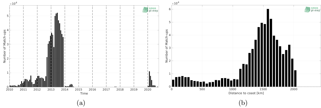
Figure 1: Number of match-ups between Surface drifters and SMOS SSS L4 v1 - Monthly (CMEMS-CNR) SSS as a function of time (a) and as function of the distance to coast (b) over the Amazon and Orinoco river plumes Pi-MEP region and for the full satellite product period.
