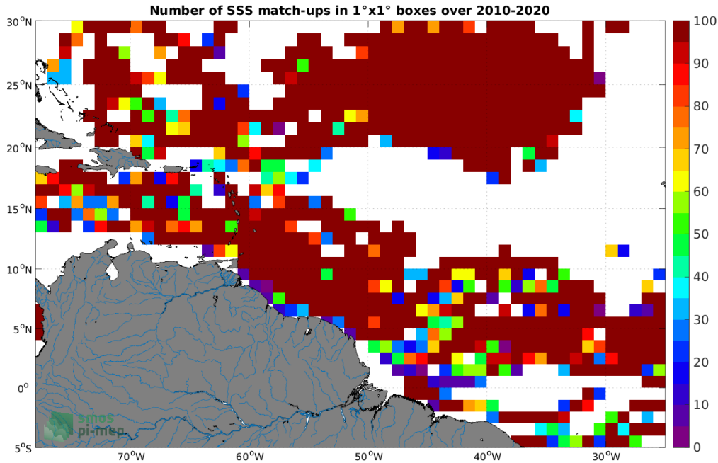
Figure 3: Number of SSS match-ups between Surface drifters SSS and the SMOS SSS L4 v1 - Monthly (CMEMS-CNR) SSS product for the Amazon and Orinoco river plumes Pi-MEP region over 1^\circ \times 1^\circ boxes and for the full satellite product period.
