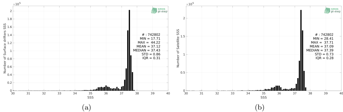
Figure 2: Histograms of SSS from Surface drifters (a) and SMOS SSS L4 v1 - Monthly (CMEMS-CNR) (b) considering all match-up pairs per bins of 0.1 over the Amazon and Orinoco river plumes Pi-MEP region and for the full satellite product period.
