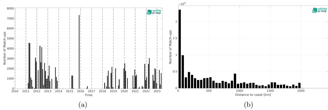
Figure 1: Number of match-ups between TSG (SAMOS) and SMOS SSS L4 OI v342 - Weekly (CMEMS-CATDS-LOPS) SSS as a function of time (a) and as function of the distance to coast (b) over the Amazon and Orinoco river plumes Pi-MEP region and for the full satellite product period.
