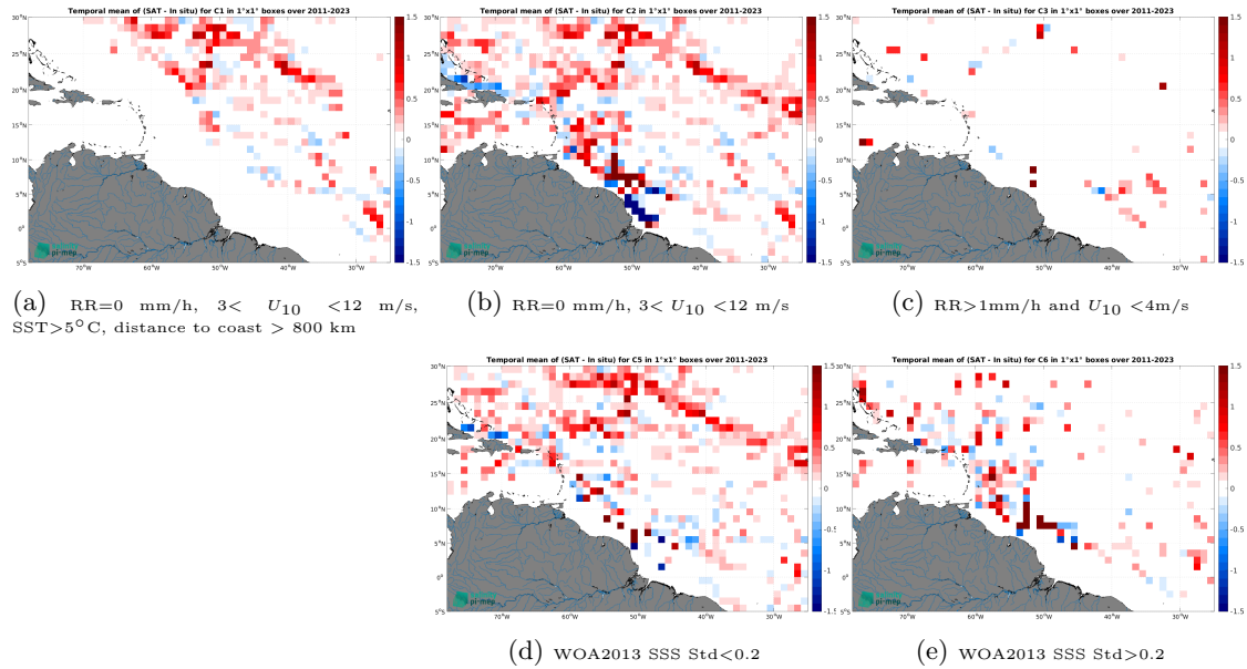
Figure 12: Temporal mean gridded over spatial boxes of size 1^\circ \times 1^\circ of \Delta SSS (SMOS SSS L4 OI v342 - Weekly (CMEMS-CATDS-LOPS) - TSG (SAMOS)) for 5 different subdatasets corresponding to:RR=0 mm/h, 3 < U_{10} < 12 m/s, SST >5^\circ\text{C} , distance to coast > 800 km (a), RR=0 mm/h, 3 < U_{10} < 12 m/s (b), RR >1 mm/h and U_{10} < 4 m/s (c), WOA2013 SSS Std <0.2 (d), WOA2013 SSS Std >0.2 (e).
