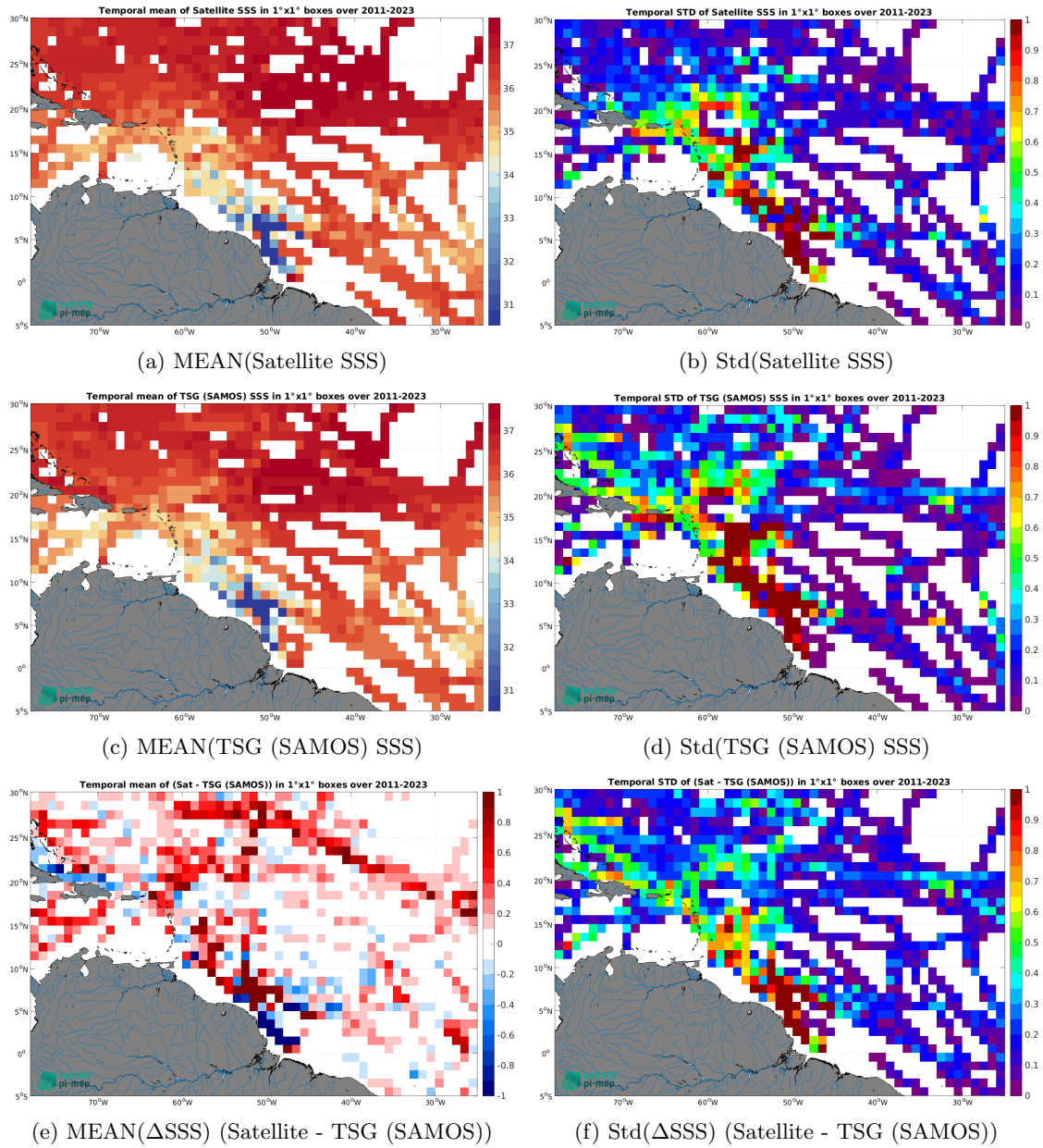
Figure 6: Temporal mean (left) and Std (right) of SSS from SMOS SSS L4 OI v342 - Weekly (CMEMS-CATDS-LOPS) (top), TSG (SAMOS) (middle), and of \Delta SSS (Satellite - TSG (SAMOS)). Only match-up pairs are used to generate these maps.
