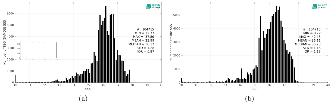
Figure 2: Histograms of SSS from TSG (SAMOS) (a) and SMOS SSS L4 OI v342 - Weekly (CMEMS-CATDS-LOPS) (b) considering all match-up pairs per bins of 0.1 over the Amazon and Orinoco river plumes Pi-MEP region and for the full satellite product period.
