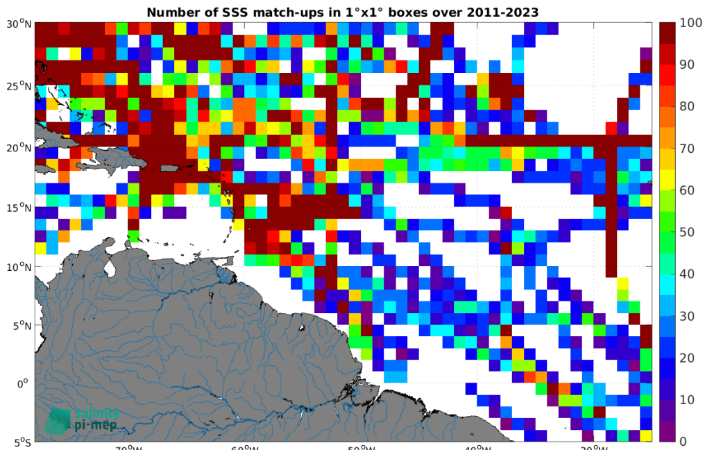
Figure 4: Number of SSS match-ups between TSG (SAMOS) SSS and the SMOS SSS L4 OI v342 - Weekly (CMEMS-CATDS-LOPS) SSS product for the Amazon and Orinoco river plumes Pi-MEP region over 1^\circ \times 1^\circ boxes and for the full satellite product period.
