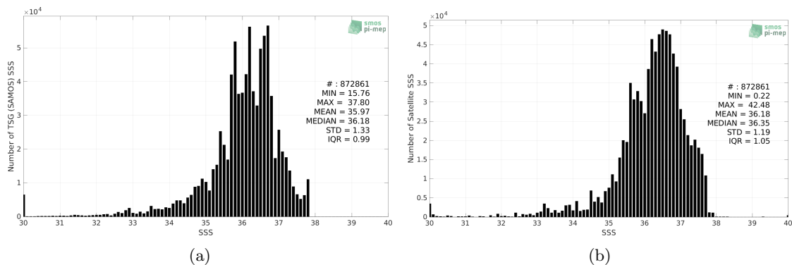
Figure 2: Histograms of SSS from TSG (SAMOS) (a) and SMOS SSS L4 OI v342 - Weekly (CMEMS-CATDS-LOPS) (b) considering all match-up pairs per bins of 0.1 over the Amazon and Orinoco river plumes Pi-MEP region and for the full satellite product period.
