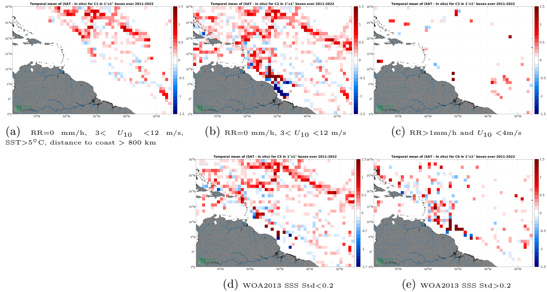
Figure 12: Temporal mean gridded over spatial boxes of size 1^{\circ}\times 1^{\circ} of \Delta\text{SSS} (SMOS SSS L4 OI v342 - Weekly (CMEMS-CATDS-LOPS) - TSG (SAMOS)) for 5 different subdatasets corresponding to:RR=0 mm/h, 3 < U_{10} < 12 m/s, SST >5^{\circ}\text{C} , distance to coast > 800 km (a), RR=0 mm/h, 3 < U_{10} < 12 m/s (b), RR >1 mm/h and U_{10} < 4 m/s (c), WOA2013 SSS Std <0.2 (d), WOA2013 SSS Std >0.2 (e).
