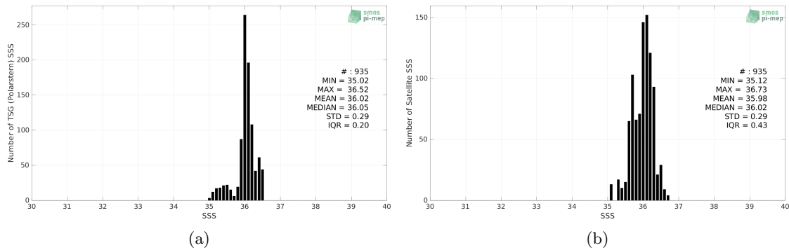
Figure 2: Histograms of SSS from TSG (Polarstern) (a) and SMOS SSS L4 OI v342 - Weekly (CMEMS-CATDS-LOPS) (b) considering all match-up pairs per bins of 0.1 over the Amazon and Orinoco river plumes Pi-MEP region and for the full satellite product period.
