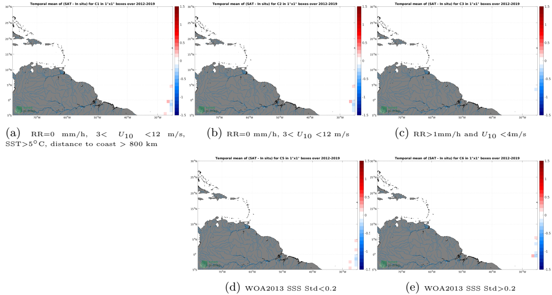
Figure 12: Temporal mean gridded over spatial boxes of size 1^{\circ}\times 1^{\circ} of \Delta\text{SSS} (SMOS SSS L4 OI v342 - Weekly (CMEMS-CATDS-LOPS) - TSG (Polarstern)) for 5 different subdatasets corresponding to:RR=0 mm/h, 3 < U_{10} < 12 m/s, SST > 5^{\circ}\text{C} , distance to coast > 800 km (a), RR=0 mm/h, 3 < U_{10} < 12 m/s (b), RR > 1 mm/h and U_{10} < 4 m/s (c), WOA2013 SSS Std < 0.2 (d), WOA2013 SSS Std > 0.2 (e).
