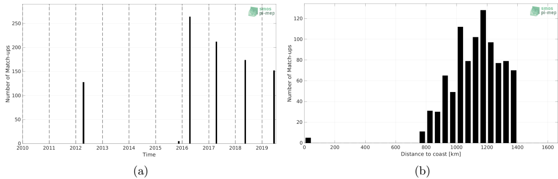
Figure 1: Number of match-ups between TSG (Polarstern) and SMOS SSS L4 OI v342 - Weekly (CMEMS-CATDS-LOPS) SSS as a function of time (a) and as function of the distance to coast (b) over the Amazon and Orinoco river plumes Pi-MEP region and for the full satellite product period.
