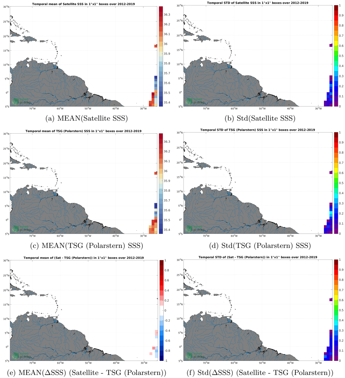
Figure 6: Temporal mean (left) and Std (right) of SSS from SMOS SSS L4 OI v342 - Weekly (CMEMS-CATDS-LOPS) (top), TSG (Polarstern) (middle), and of \Delta SSS (Satellite - TSG (Polarstern)). Only match-up pairs are used to generate these maps.
