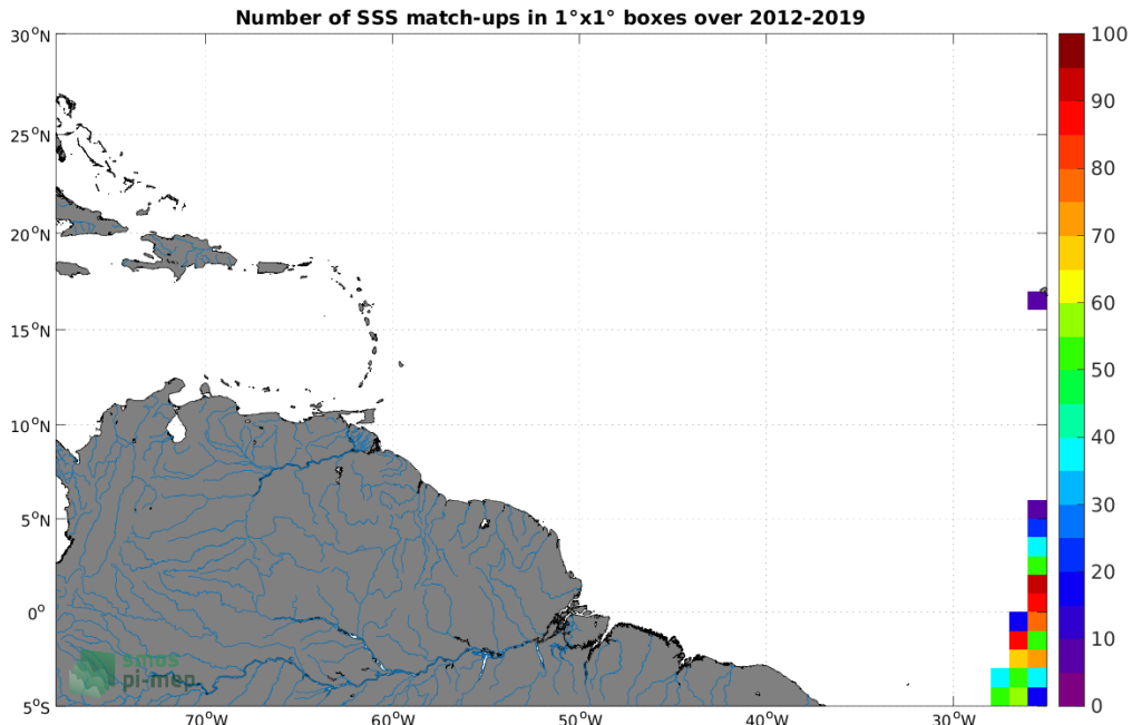
Figure 4: Number of SSS match-ups between TSG (Polarstern) SSS and the SMOS SSS L4 OI v342 - Weekly (CMEMS-CATDS-LOPS) SSS product for the Amazon and Orinoco river plumes Pi-MEP region over 1^\circ \times 1^\circ boxes and for the full satellite product period.
