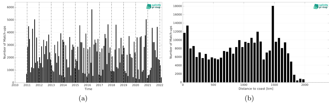
Figure 1: Number of match-ups between TSG (LEGOS-DM) and SMOS SSS L4 OI v342 - Weekly (CMEMS-CATDS-LOPS) SSS as a function of time (a) and as function of the distance to coast (b) over the Amazon and Orinoco river plumes Pi-MEP region and for the full satellite product period.
