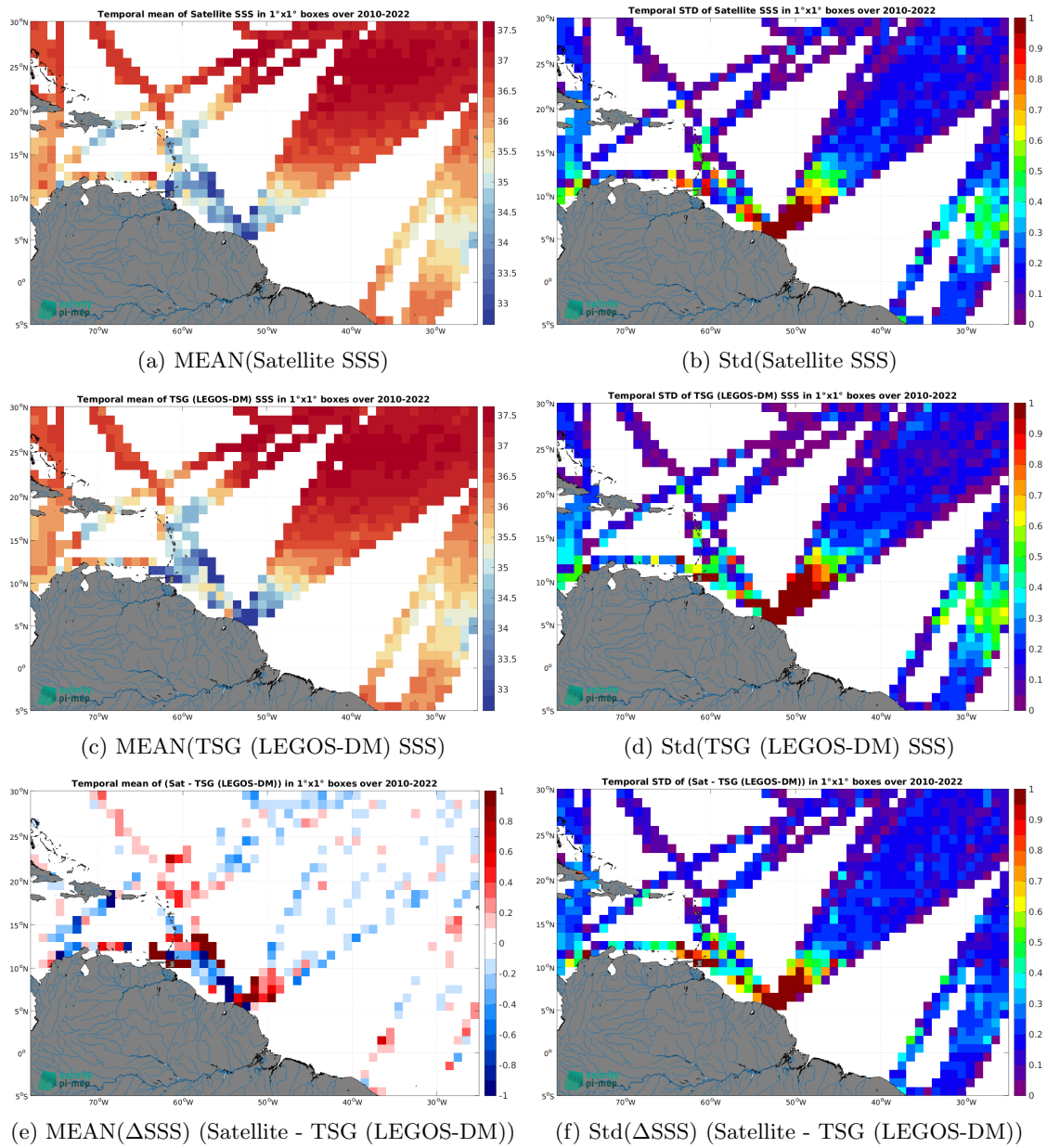
Figure 6: Temporal mean (left) and Std (right) of SSS from SMOS SSS L4 OI v342 - Weekly (CMEMS-CATDS-LOPS) (top), TSG (LEGOS-DM) (middle), and of \Delta SSS (Satellite - TSG (LEGOS-DM)). Only match-up pairs are used to generate these maps.
