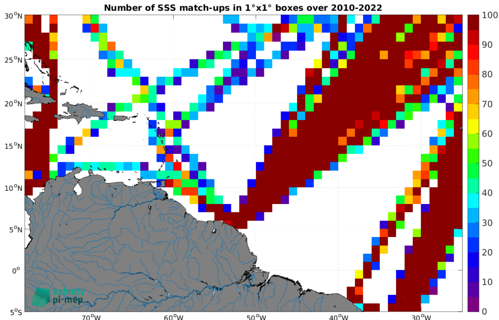
Figure 4: Number of SSS match-ups between TSG (LEGOS-DM) SSS and the SMOS SSS L4 OI v342 - Weekly (CMEMS-CATDS-LOPS) SSS product for the Amazon and Orinoco river plumes Pi-MEP region over 1^\circ \times 1^\circ boxes and for the full satellite product period.
