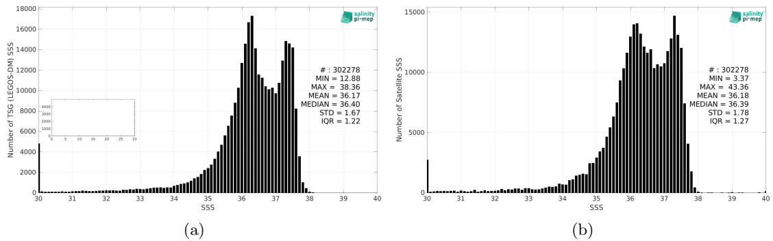
Figure 2: Histograms of SSS from TSG (LEGOS-DM) (a) and SMOS SSS L4 OI v342 - Weekly (CMEMS-CATDS-LOPS) (b) considering all match-up pairs per bins of 0.1 over the Amazon and Orinoco river plumes Pi-MEP region and for the full satellite product period.
