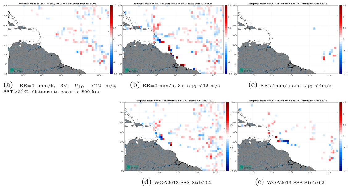
Figure 12: Temporal mean gridded over spatial boxes of size 1^{\circ}\times 1^{\circ} of \Delta SSS (SMOS SSS L4 OI v342 - Weekly (CMEMS-CATDS-LOPS) - TSG (GOSUD-Sailing-ship)) for 5 different sub-datasets corresponding to:RR=0 mm/h, 3 < U_{10} < 12 m/s, SST >5^{\circ}\text{C} , distance to coast > 800 km (a), RR=0 mm/h, 3 < U_{10} < 12 m/s (b), RR >1 mm/h and U_{10} < 4 m/s (c), WOA2013 SSS Std <0.2 (d), WOA2013 SSS Std >0.2 (e).
