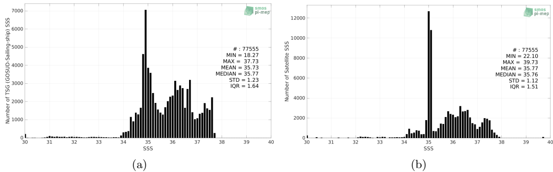
Figure 2: Histograms of SSS from TSG (GOSUD-Sailing-ship) (a) and SMOS SSS L4 OI v342 - Weekly (CMEMS-CATDS-LOPS) (b) considering all match-up pairs per bins of 0.1 over the Amazon and Orinoco river plumes Pi-MEP region and for the full satellite product period.
