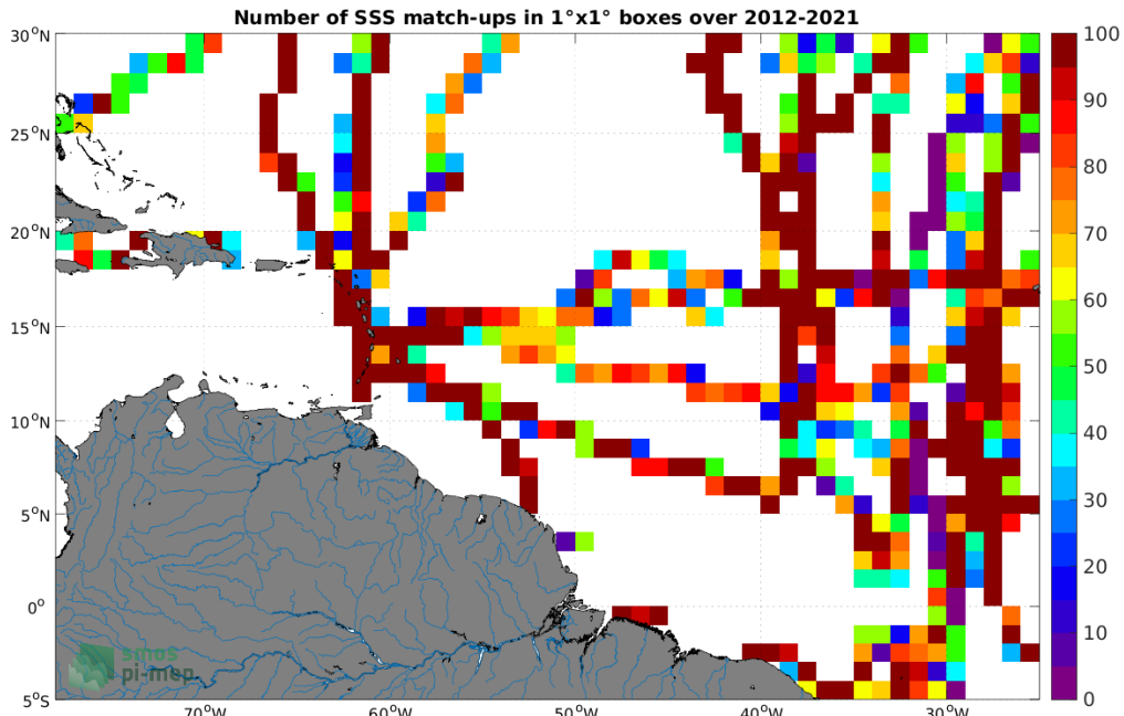
Figure 4: Number of SSS match-ups between TSG (GOSUD-Sailing-ship) SSS and the SMOS SSS L4 OI v342 - Weekly (CMEMS-CATDS-LOPS) SSS product for the Amazon and Orinoco river plumes Pi-MEP region over 1^\circ \times 1^\circ boxes and for the full satellite product period.
