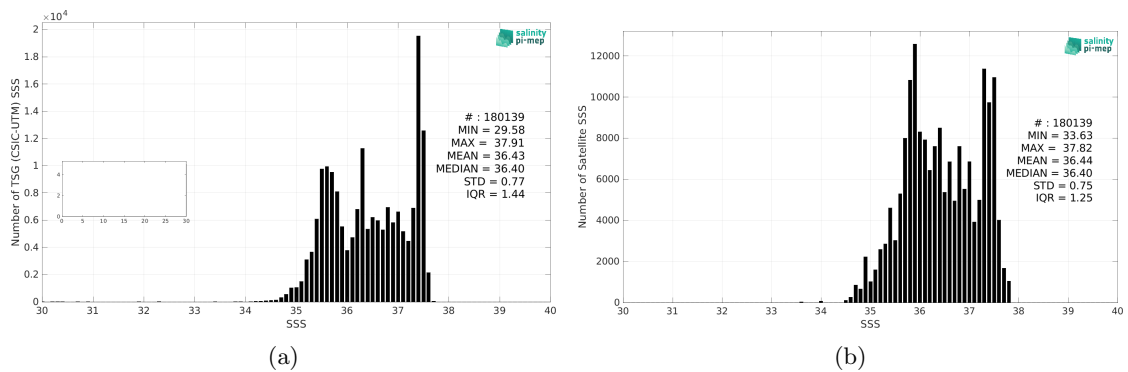
Figure 2: Histograms of SSS from TSG (CSIC-UTM) (a) and SMOS SSS L4 OI v342 - Weekly (CMEMS-CATDS-LOPS) (b) considering all match-up pairs per bins of 0.1 over the Amazon and Orinoco river plumes Pi-MEP region and for the full satellite product period.
