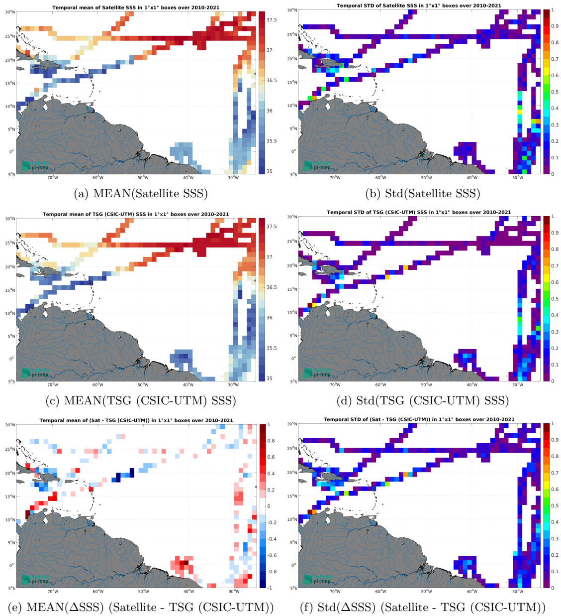
Figure 6: Temporal mean (left) and Std (right) of SSS from SMOS SSS L4 OI v342 - Weekly (CMEMS-CATDS-LOPS) (top), TSG (CSIC-UTM) (middle), and of \Delta SSS (Satellite - TSG (CSIC-UTM)). Only match-up pairs are used to generate these maps.
