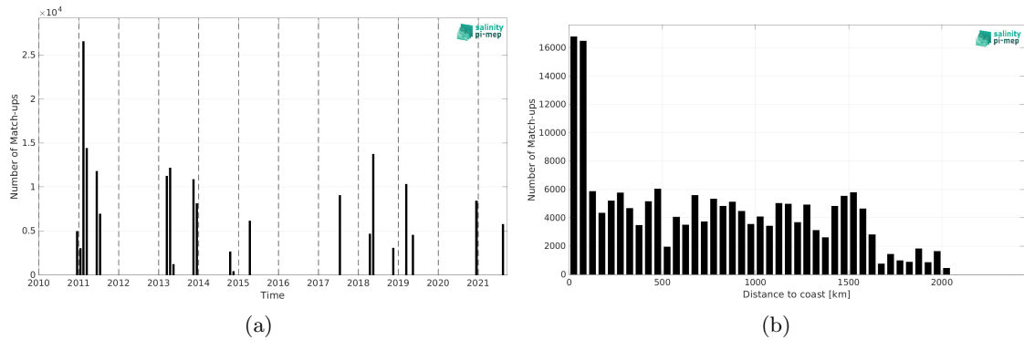
Figure 1: Number of match-ups between TSG (CSIC-UTM) and SMOS SSS L4 OI v342 - Weekly (CMEMS-CATDS-LOPS) SSS as a function of time (a) and as function of the distance to coast (b) over the Amazon and Orinoco river plumes Pi-MEP region and for the full satellite product period.
