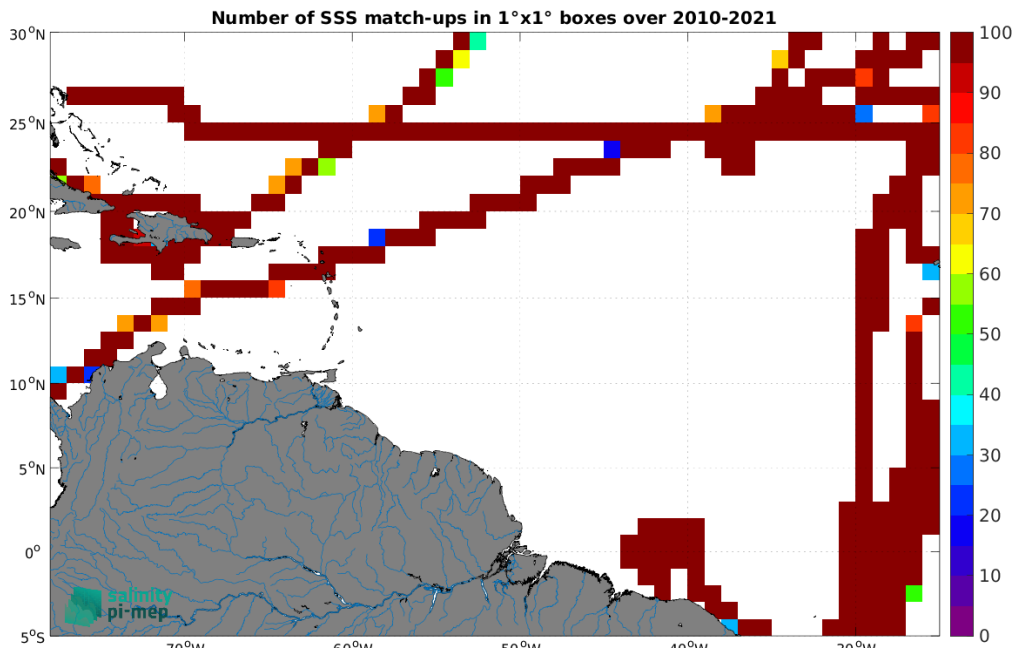
Figure 4: Number of SSS match-ups between TSG (CSIC-UTM) SSS and the SMOS SSS L4 OI v342 - Weekly (CMEMS-CATDS-LOPS) SSS product for the Amazon and Orinoco river plumes Pi-MEP region over 1^\circ \times 1^\circ boxes and for the full satellite product period.
