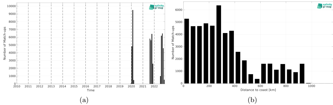
Figure 1: Number of match-ups between Saildrone and SMOS SSS L4 OI v342 - Weekly (CMEMS-CATDS-LOPS) SSS as a function of time (a) and as function of the distance to coast (b) over the Amazon and Orinoco river plumes Pi-MEP region and for the full satellite product period.
