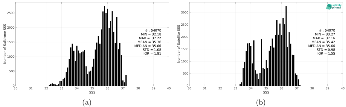
Figure 2: Histograms of SSS from Saildrone (a) and SMOS SSS L4 OI v342 - Weekly (CMEMS-CATDS-LOPS) (b) considering all match-up pairs per bins of 0.1 over the Amazon and Orinoco river plumes Pi-MEP region and for the full satellite product period.
