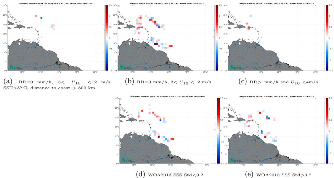
Figure 12: Temporal mean gridded over spatial boxes of size 1^\circ \times 1^\circ of \Delta\text{SSS} (SMOS SSS L4 OI v342 - Weekly (CMEMS-CATDS-LOPS) - Saildrone) for 5 different subdatasets corresponding to:RR=0 mm/h, 3 < U_{10} < 12 m/s, SST >5^\circ\text{C} , distance to coast > 800 km (a), RR=0 mm/h, 3 < U_{10} < 12 m/s (b), RR >1 mm/h and U_{10} < 4 m/s (c), WOA2013 SSS Std <0.2 (d), WOA2013 SSS Std >0.2 (e).
