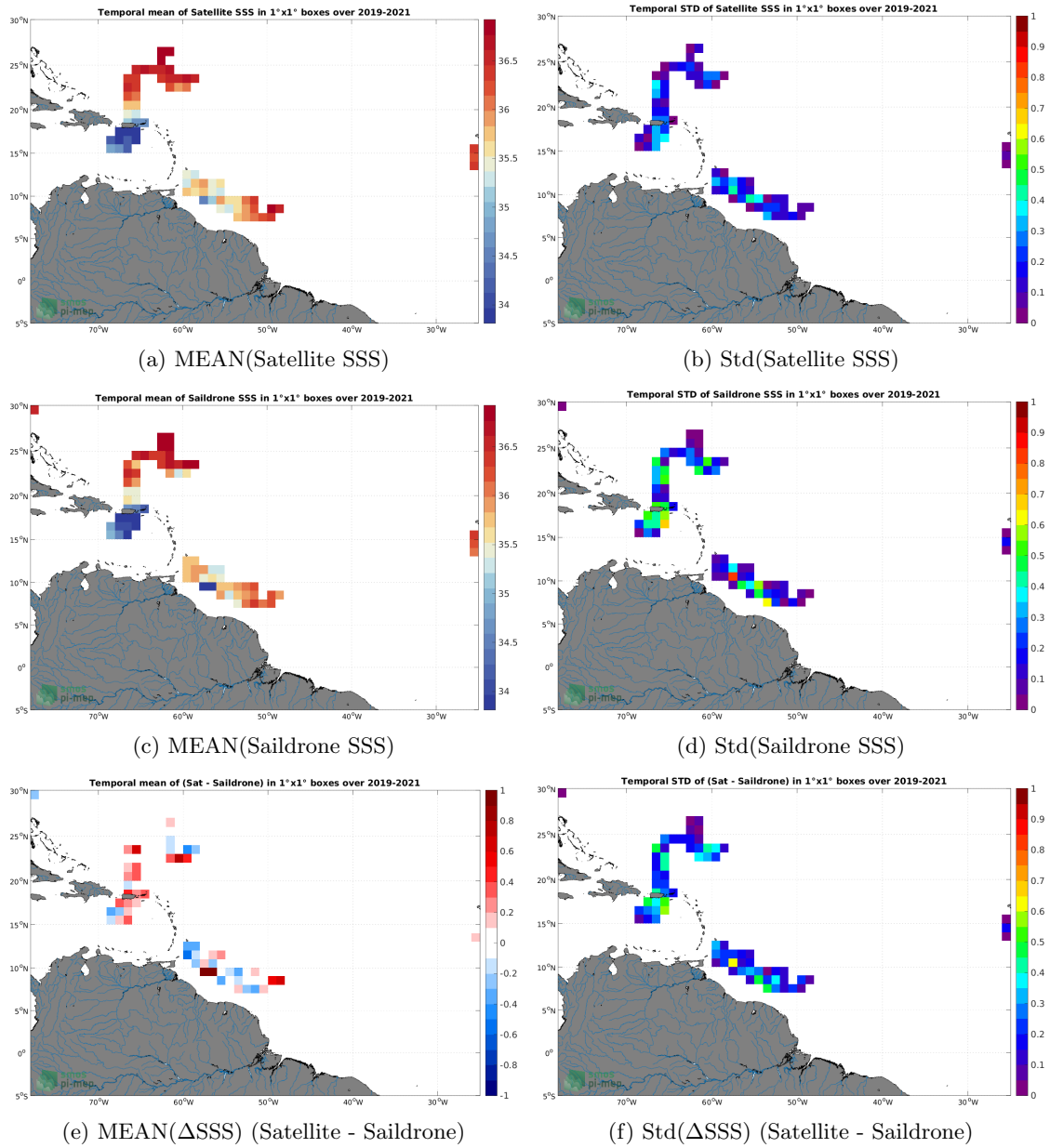
Figure 6: Temporal mean (left) and Std (right) of SSS from SMOS SSS L4 OI v342 - Weekly (CMEMS-CATDS-LOPS) (top), Saildrone (middle), and of \Delta SSS (Satellite - Saildrone). Only match-up pairs are used to generate these maps.
