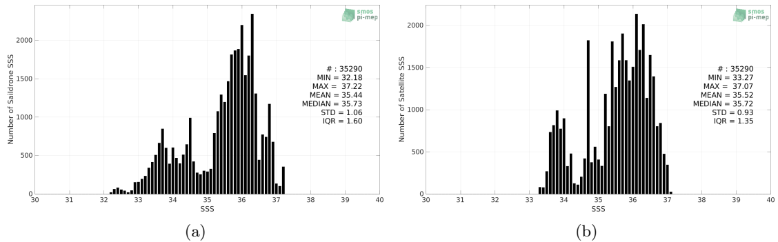
Figure 2: Histograms of SSS from Sairdrone (a) and SMOS SSS L4 OI v342 - Weekly (CMEMS-CATDS-LOPS) (b) considering all match-up pairs per bins of 0.1 over the Amazon and Orinoco river plumes Pi-MEP region and for the full satellite product period.
