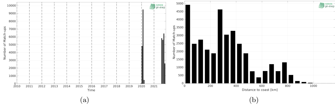
Figure 1: Number of match-ups between Sairdrone and SMOS SSS L4 OI v342 - Weekly (CMEMS-CATDS-LOPS) SSS as a function of time (a) and as function of the distance to coast (b) over the Amazon and Orinoco river plumes Pi-MEP region and for the full satellite product period.
