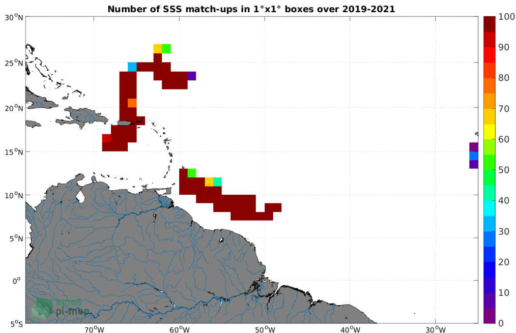
Figure 4: Number of SSS match-ups between Saildrone SSS and the SMOS SSS L4 OI v342 - Weekly (CMEMS-CATDS-LOPS) SSS product for the Amazon and Orinoco river plumes Pi-MEP region over 1^\circ \times 1^\circ boxes and for the full satellite product period.
