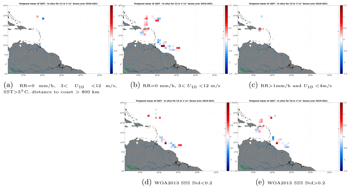
Figure 12: Temporal mean gridded over spatial boxes of size 1^\circ \times 1^\circ of \Delta SSS (SMOS SSS L4 OI v342 - Weekly (CMEMS-CATDS-LOPS) - Saildrone) for 5 different subdatasets corresponding to:RR=0 mm/h, 3 < U_{10} < 12 m/s, SST >5^\circ C, distance to coast > 800 km (a), RR=0 mm/h, 3 < U_{10} < 12 m/s (b), RR >1 mm/h and U_{10} < 4 m/s (c), WOA2013 SSS Std <0.2 (d), WOA2013 SSS Std >0.2 (e).
