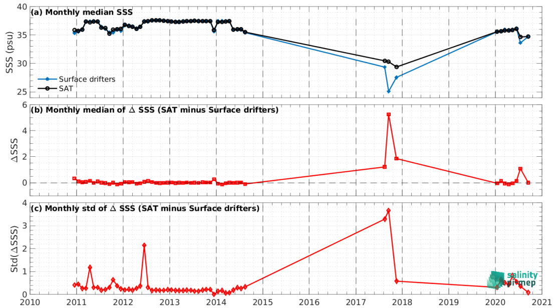
Figure 6: Time series of the monthly median SSS (top), median of \Delta SSS (Satellite - Surface drifters) over the Amazon and Orinoco river plumes Pi-MEP region considering all match-ups collected by the Pi-MEP.
