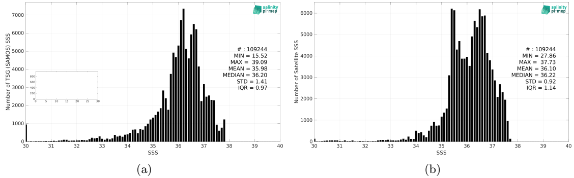
Figure 2: Histograms of SSS from TSG (SAMOS) (a) and SMOS SSS L4 v2 - Daily (BEC) (b) considering all match-up pairs per bins of 0.1 over the Amazon and Orinoco river plumes Pi-MEP region and for the full satellite product period.
