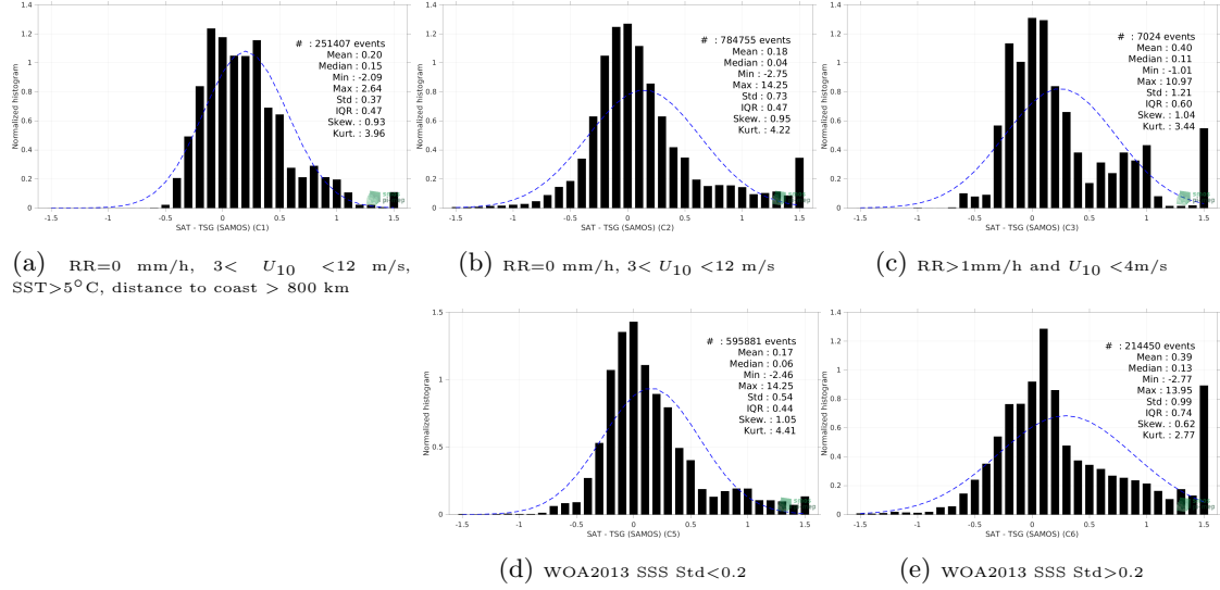
Figure 13: Normalized histogram of \Delta SSS (SMOS SSS L4 v2 - Daily (BEC) - TSG (SAMOS)) for 5 different subdatasets corresponding to: RR=0 mm/h, 3 < U_{10} < 12 m/s, SST>5°C, distance to coast > 800 km (a), RR=0 mm/h, 3 < U_{10} < 12 m/s (b), RR>1mm/h and U_{10} < 4 m/s (c), WOA2013 SSS Std<0.2 (d), WOA2013 SSS Std>0.2 (e).
