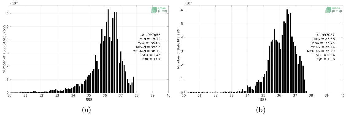
Figure 2: Histograms of SSS from TSG (SAMOS) (a) and SMOS SSS L4 v2 - Daily (BEC) (b) considering all match-up pairs per bins of 0.1 over the Amazon and Orinoco river plumes Pi-MEP region and for the full satellite product period.
