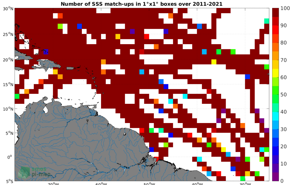
Figure 4: Number of SSS match-ups between TSG (SAMOS) SSS and the SMOS SSS L4 v2 - Daily (BEC) SSS product for the Amazon and Orinoco river plumes Pi-MEP region over 1^\circ \times 1^\circ boxes and for the full satellite product period.
