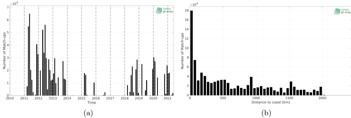
Figure 1: Number of match-ups between TSG (SAMOS) and SMOS SSS L4 v2 - Daily (BEC) SSS as a function of time (a) and as function of the distance to coast (b) over the Amazon and Orinoco river plumes Pi-MEP region and for the full satellite product period.
